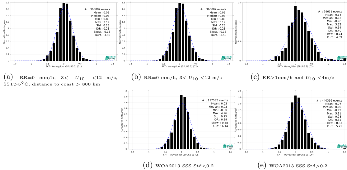
Figure 13: Normalized histogram of \Delta SSS (SMOS SSS L3 v9 - 9 Days (CATDS-CEC-LOCEAN) - Waveglider (SPURS 2)) for 5 different subdatasets corresponding to: RR=0 mm/h, 3 < U_{10} < 12 m/s, SST>5°C, distance to coast > 800 km (a), RR=0 mm/h, 3 < U_{10} < 12 m/s (b), RR>1mm/h and U_{10} < 4 m/s (c), WOA2013 SSS Std<0.2 (d), WOA2013 SSS Std>0.2 (e).
