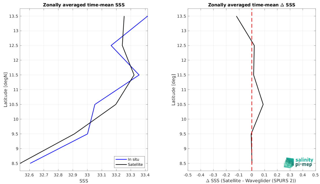
Figure 8: Left panel: Zonal mean SSS from SMOS SSS L3 v9 - 9 Days (CATDS-CEC-LOCEAN) satellite product (black) and from Waveglider (SPURS 2) (blue). Right panel: Zonal mean of \Delta SSS (Satellite - Waveglider (SPURS 2)) for all the collected Pi-MEP match-up pairs estimated over the full satellite product period.
