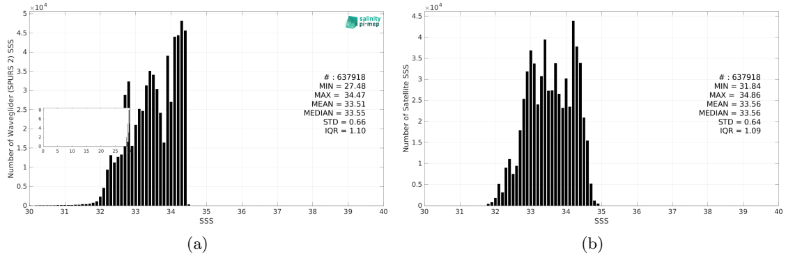
Figure 2: Histograms of SSS from Waveglider (SPURS 2) (a) and SMOS SSS L3 v9 - 9 Days (CATDS-CEC-LOCEAN) (b) considering all match-up pairs per bins of 0.1 over the SPURS 2 Pi-MEP region and for the full satellite product period.
