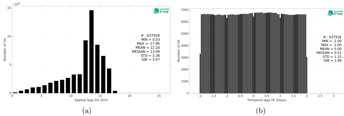
Figure 5: Histograms of the spatial (a) and temporal (b) lags between the location/time of the Waveglider (SPURS 2) measurement and the date of the corresponding SMOS SSS L3 v9 - 9 Days (CATDS-CEC-LOCEAN) SSS pixel.
