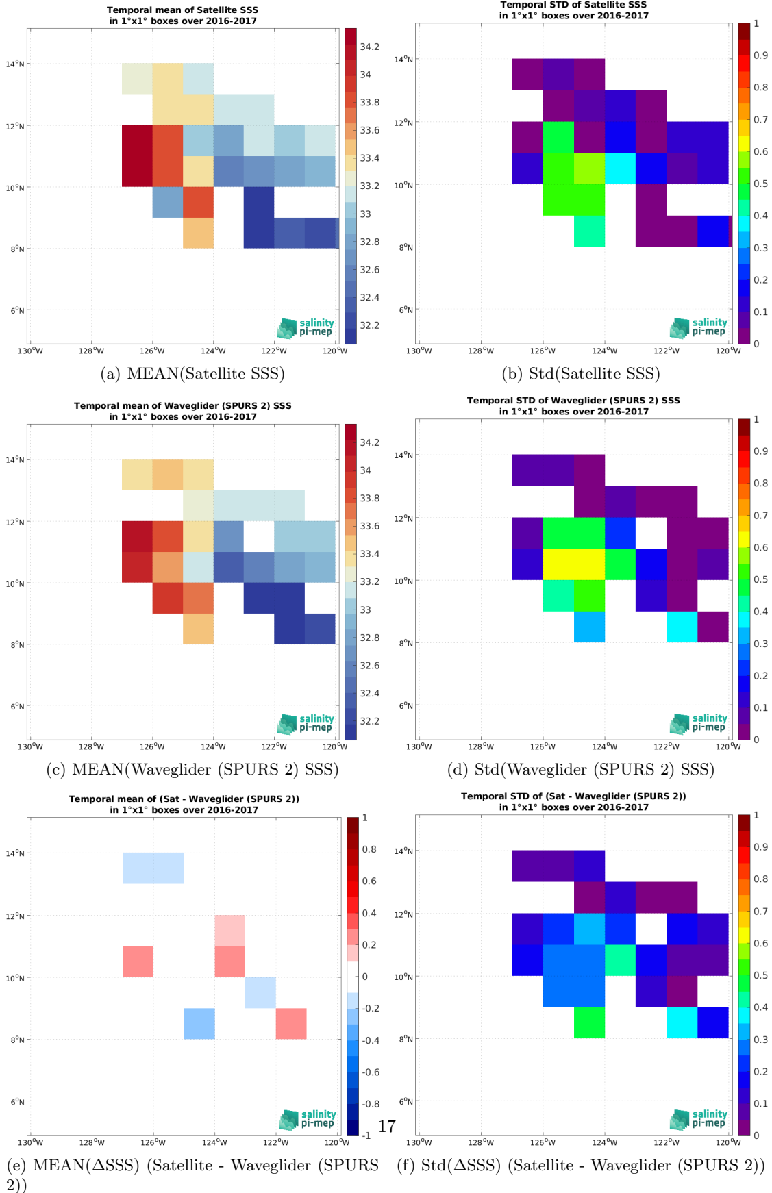
Figure 6: Temporal mean (left) and Std (right) of SSS from SMOS SSS L3 v9 - 9 Days (CATDS-CEC-LOCEAN) (top), Waveglider (SPURS 2) (middle), and of \Delta SSS (Satellite - Waveglider (SPURS 2)). Only match-up pairs are used to generate these maps.
