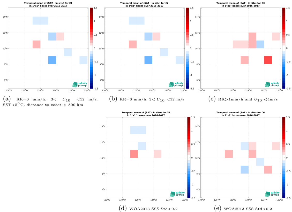
Figure 12: Temporal mean gridded over spatial boxes of size 1^{\circ}\times 1^{\circ} of \Delta\text{SSS} (SMOS SSS L3 v9 - 9 Days (CATDS-CEC-LOCEAN) - Waveglider (SPURS 2)) for 5 different subdatasets corresponding to:RR=0 mm/h, 3 < U_{10} < 12 m/s, SST >5^{\circ}\text{C} , distance to coast > 800 km (a), RR=0 mm/h, 3 < U_{10} < 12 m/s (b), RR >1 mm/h and U_{10} < 4 m/s (c), WOA2013 SSS Std <0.2 (d), WOA2013 SSS Std >0.2 (e).
