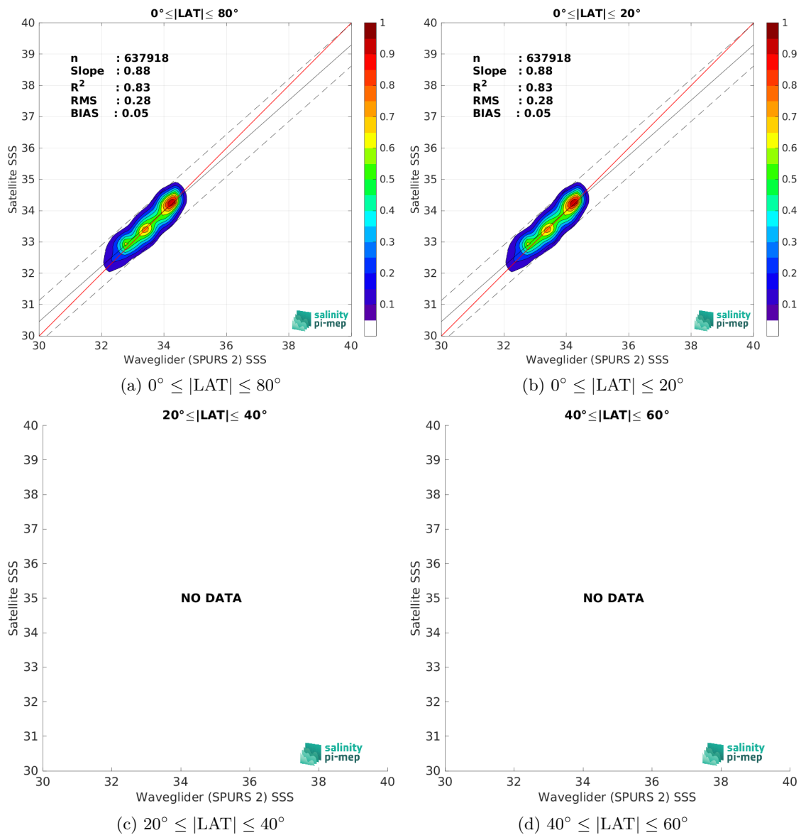
Figure 9: Contour maps of the concentration of SMOS SSS L3 v9 - 9 Days (CATDS-CEC-LOCEAN) SSS (y-axis) versus Waveglider (SPURS 2) SSS (x-axis) at match-up pairs for different latitude bands. For each plot, the red line shows x=y . The black thin and dashed lines indicate a linear fit through the data cloud and the \pm 95\% confidence levels, respectively. The number match-up pairs n , the slope and R^2 coefficient of the linear fit, the root mean square (RMS) and the mean bias between satellite and in situ data are indicated for each latitude band in each plots.
