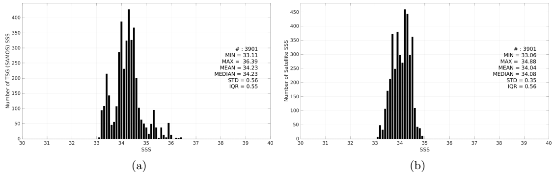
Figure 3: Histograms of SSS from TSG (SAMOS) (a) and SMOS SSS L3 v9 - 9 Days (CATDS-CEC-LOCEAN) (b) considering all match-up pairs per bins of 0.1 over the SPURS 2 Pi-MEP region and for the full satellite product period.
