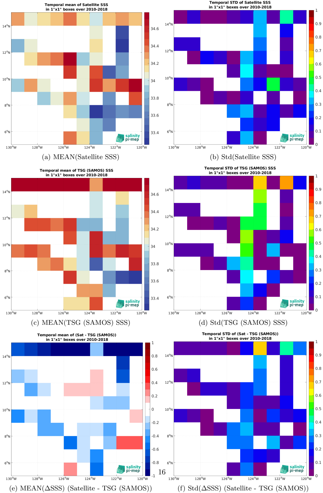
Figure 7: Temporal mean (left) and Std (right) of SSS from SMOS SSS L3 v9 - 9 Days (CATDS-CEC-LOCEAN) (top), TSG (SAMOS) (middle), and of \Delta SSS (Satellite - TSG (SAMOS)). Only match-up pairs are used to generate these maps.
