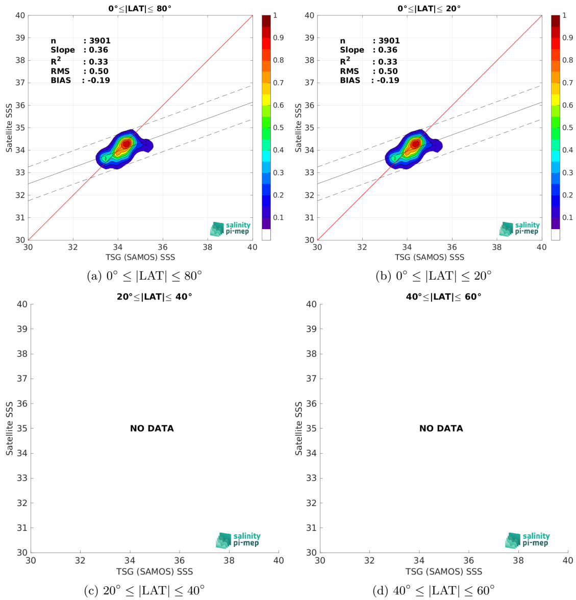
Figure 10: Contour maps of the concentration of SMOS SSS L3 v9 - 9 Days (CATDS-CEC-LOCEAN) SSS (y-axis) versus TSG (SAMOS) SSS (x-axis) at match-up pairs for different latitude bands. For each plot, the red line shows x=y . The black thin and dashed lines indicate a linear fit through the data cloud and the \pm 95\% confidence levels, respectively. The number match-up pairs n , the slope and R^2 coefficient of the linear fit, the root mean square (RMS) and the mean bias between satellite and in situ data are indicated for each latitude band in each plots.
