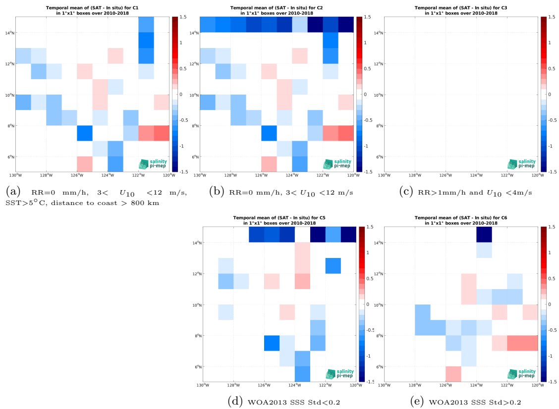
Figure 14: Temporal mean gridded over spatial boxes of size 1^\circ \times 1^\circ of \Delta\text{SSS} (SMOS SSS L3 v9 - 9 Days (CATDS-CEC-LOCEAN) - TSG (SAMOS)) for 5 different subdatasets corresponding to:RR=0 mm/h, 3 < U_{10} < 12 m/s, SST>5°C, distance to coast > 800 km (a), RR=0 mm/h, 3 < U_{10} < 12 m/s (b), RR>1mm/h and U_{10} < 4 m/s (c), WOA2013 SSS Std<0.2 (d), WOA2013 SSS Std>0.2 (e).
