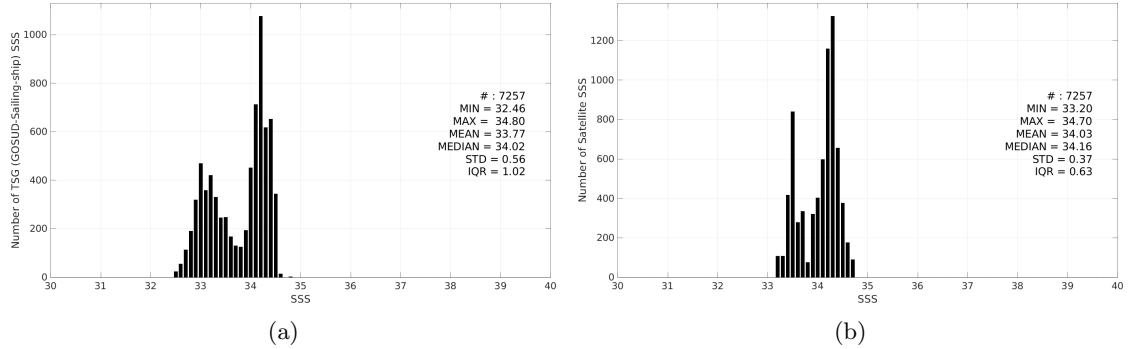
Figure 3: Histograms of SSS from TSG (GOSUD-Sailing-ship) (a) and SMOS SSS L3 v9 - 9 Days (CATDS-CEC-LOCEAN) (b) considering all match-up pairs per bins of 0.1 over the SPURS 2 Pi-MEP region and for the full satellite product period.
