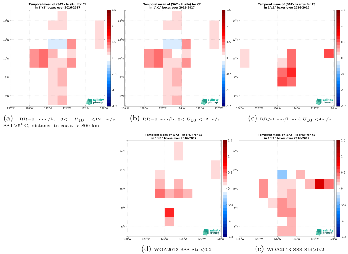
Figure 12: Temporal mean gridded over spatial boxes of size 1^\circ \times 1^\circ of \Delta SSS (SMOS SSS L3 v9 - 9 Days (CATDS-CEC-LOCEAN) - Salinity Snake (SPURS 2)) for 5 different subdatasets corresponding to: RR=0 mm/h, 3 < U_{10} < 12 m/s, SST > 5°C, distance to coast > 800 km (a), RR=0 mm/h, 3 < U_{10} < 12 m/s (b), RR > 1mm/h and U_{10} < 4 m/s (c), WOA2013 SSS Std < 0.2 (d), WOA2013 SSS Std > 0.2 (e).
