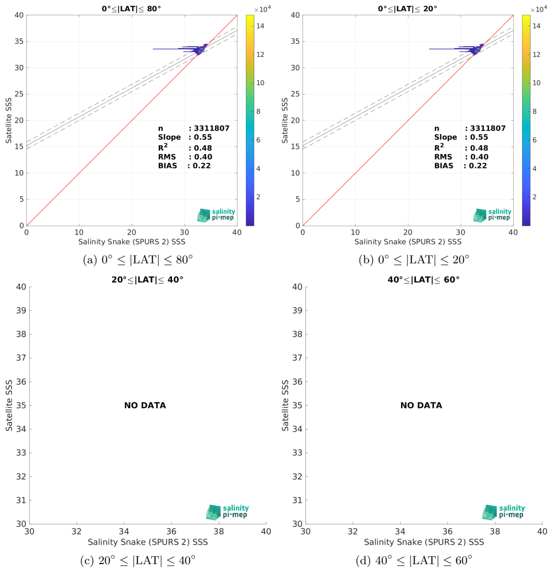
Figure 9: Contour maps of the concentration of SMOS SSS L3 v9 - 9 Days (CATDS-CEC-LOCEAN) SSS (y-axis) versus Salinity Snake (SPURS 2) SSS (x-axis) at match-up pairs for different latitude bands. For each plot, the red line shows x=y . The black thin and dashed lines indicate a linear fit through the data cloud and the \pm 95\% confidence levels, respectively. The number match-up pairs n , the slope and R^2 coefficient of the linear fit, the root mean square (RMS) and the mean bias between satellite and in situ data are indicated for each latitude band in each plots.
