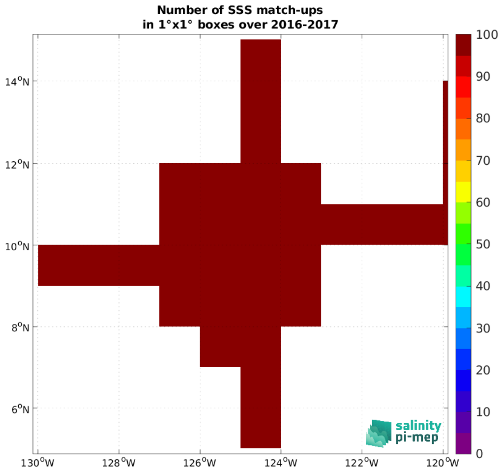
Figure 4: Number of SSS match-ups between Salinity Snake (SPURS 2) SSS and the SMOS SSS L3 v9 - 9 Days (CATDS-CEC-LOCEAN) SSS product for the SPURS 2 Pi-MEP region over 1^\circ \times 1^\circ boxes and for the full satellite product period.
