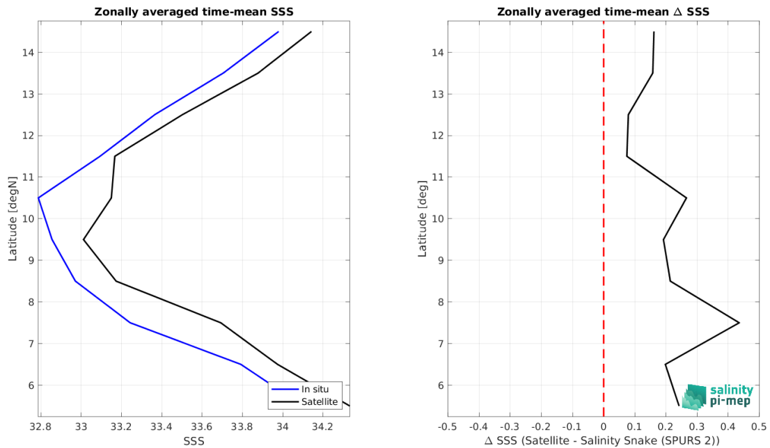
Figure 8: Left panel: Zonal mean SSS from SMOS SSS L3 v9 - 9 Days (CATDS-CEC-LOCEAN) satellite product (black) and from Salinity Snake (SPURS 2) (blue). Right panel: Zonal mean of \Delta SSS (Satellite - Salinity Snake (SPURS 2)) for all the collected Pi-MEP match-up pairs estimated over the full satellite product period.
