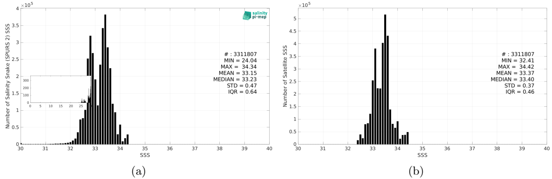
Figure 2: Histograms of SSS from Salinity Snake (SPURS 2) (a) and SMOS SSS L3 v9 - 9 Days (CATDS-CEC-LOCEAN) (b) considering all match-up pairs per bins of 0.1 over the SPURS 2 Pi-MEP region and for the full satellite product period.
