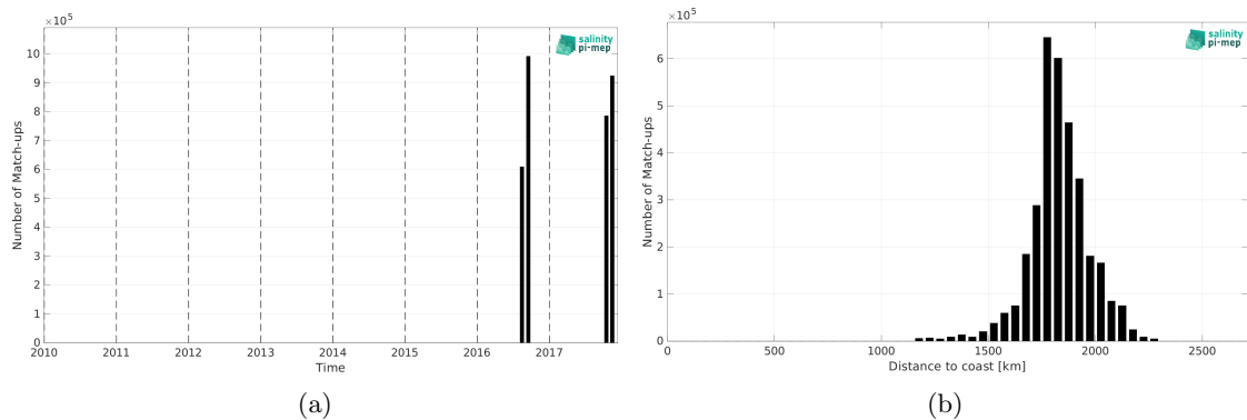
Figure 1: Number of match-ups between Salinity Snake (SPURS 2) and SMOS SSS L3 v9 - 9 Days (CATDS-CEC-LOCEAN) SSS as a function of time (a) and as function of the distance to coast (b) over the SPURS 2 Pi-MEP region and for the full satellite product period.
