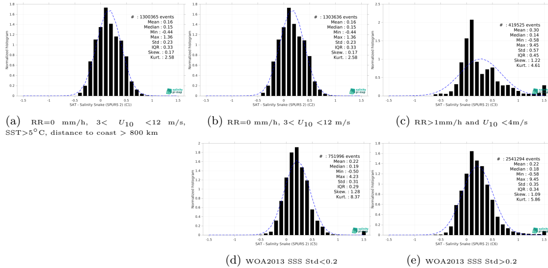
Figure 13: Normalized histogram of \Delta SSS (SMOS SSS L3 v9 - 9 Days (CATDS-CEC-LOCEAN) - Salinity Snake (SPURS 2)) for 5 different subdatasets corresponding to: RR=0 mm/h, 3 < U_{10} < 12 m/s, SST>5°C, distance to coast > 800 km (a), RR=0 mm/h, 3 < U_{10} < 12 m/s (b), RR>1mm/h and U_{10} < 4 m/s (c), WOA2013 SSS Std<0.2 (d), WOA2013 SSS Std>0.2 (e).
