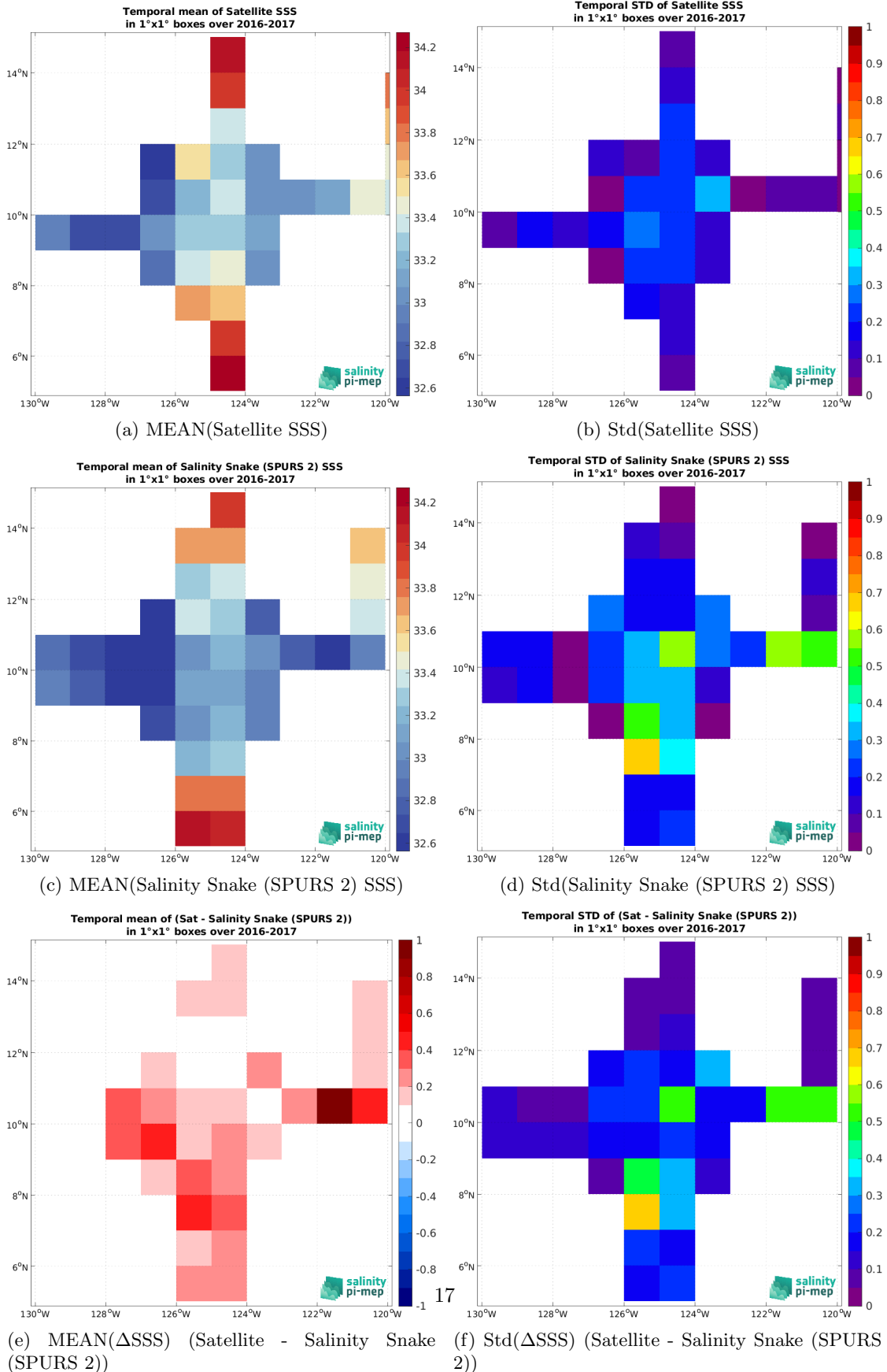
Figure 6: Temporal mean (left) and Std (right) of SSS from SMOS SSS L3 v9 - 9 Days (CATDS-CEC-LOCEAN) (top), Salinity Snake (SPURS 2) (middle), and of \Delta SSS (Satellite - Salinity Snake (SPURS 2)). Only match-up pairs are used to generate these maps.
