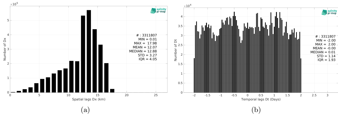
Figure 5: Histograms of the spatial (a) and temporal (b) lags between the location/time of the Salinity Snake (SPURS 2) measurement and the date of the corresponding SMOS SSS L3 v9 - 9 Days (CATDS-CEC-LOCEAN) SSS pixel.
