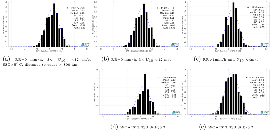
Figure 15: Normalized histogram of \Delta SSS (SMOS SSS L3 v9 - 9 Days (CATDS-CEC-LOCEAN) - Seaglider (SPURS 2)) for 5 different subdatasets corresponding to: RR=0 mm/h, 3 < U_{10} < 12 m/s, SST>5°C, distance to coast > 800 km (a), RR=0 mm/h, 3 < U_{10} < 12 m/s (b), RR>1mm/h and U_{10} < 4 m/s (c), WOA2013 SSS Std<0.2 (d), WOA2013 SSS Std>0.2 (e).
