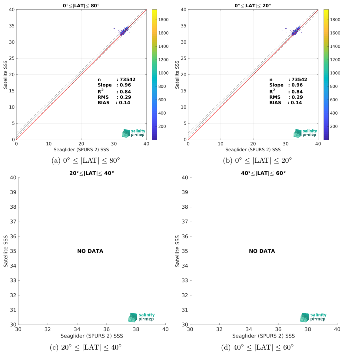
Figure 10: Contour maps of the concentration of SMOS SSS L3 v9 - 9 Days (CATDS-CEC-LOCEAN) SSS (y-axis) versus Seaglider (SPURS 2) SSS (x-axis) at match-up pairs for different latitude bands. For each plot, the red line shows x=y . The black thin and dashed lines indicate a linear fit through the data cloud and the \pm 95\% confidence levels, respectively. The number match-up pairs n , the slope and R^2 coefficient of the linear fit, the root mean square (RMS) and the mean bias between satellite and in situ data are indicated for each latitude band in each plots.
