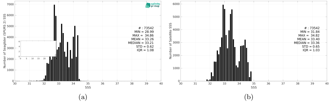
Figure 3: Histograms of SSS from Seaglider (SPURS 2) (a) and SMOS SSS L3 v9 - 9 Days (CATDS-CEC-LOCEAN) (b) considering all match-up pairs per bins of 0.1 over the SPURS 2 Pi-MEP region and for the full satellite product period.
