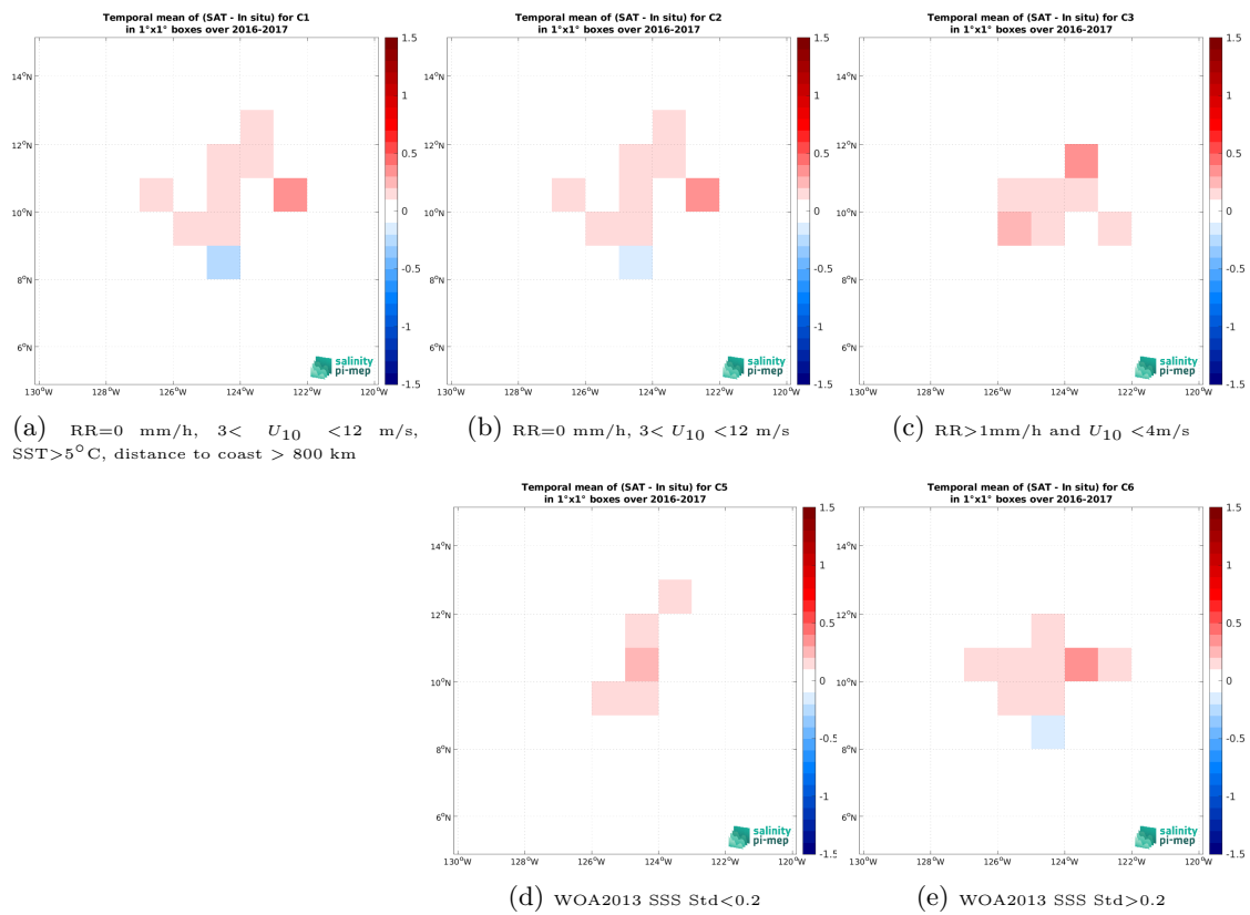
Figure 14: Temporal mean gridded over spatial boxes of size 1^\circ \times 1^\circ of \Delta SSS (SMOS SSS L3 v9 - 9 Days (CATDS-CEC-LOCEAN) - Seaglider (SPURS 2)) for 5 different subdatasets corresponding to:RR=0 mm/h, 3 < U_{10} < 12 m/s, SST >5^\circ C, distance to coast > 800 km (a), RR=0 mm/h, 3 < U_{10} < 12 m/s (b), RR >1 mm/h and U_{10} < 4 m/s (c), WOA2013 SSS Std <0.2 (d), WOA2013 SSS Std >0.2 (e).
