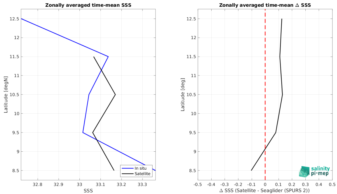
Figure 9: Left panel: Zonal mean SSS from SMOS SSS L3 v9 - 9 Days (CATDS-CEC-LOCEAN) satellite product (black) and from Seaglider (SPURS 2) (blue). Right panel: Zonal mean of \Delta SSS (Satellite - Seaglider (SPURS 2)) for all the collected Pi-MEP match-up pairs estimated over the full satellite product period.
