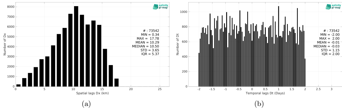
Figure 6: Histograms of the spatial (a) and temporal (b) lags between the location/time of the Seaglider (SPURS 2) measurement and the date of the corresponding SMOS SSS L3 v9 - 9 Days (CATDS-CEC-LOCEAN) SSS pixel.
