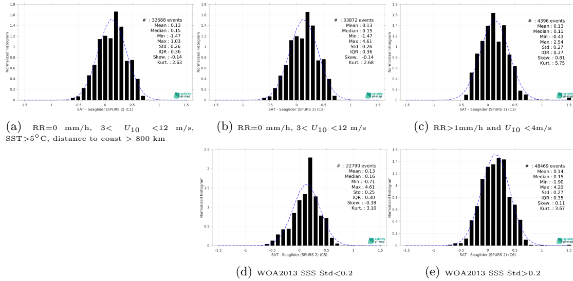
Figure 13: Normalized histogram of \Delta\text{SSS} (SMOS SSS L3 v9 - 9 Days (CATDS-CEC-LOCEAN) - Seaglider (SPURS 2)) for 5 different subdatasets corresponding to: RR=0 mm/h, 3 < U_{10} < 12 m/s, SST >5^{\circ}\text{C} , distance to coast > 800 km (a), RR=0 mm/h, 3 < U_{10} < 12 m/s (b), RR >1 mm/h and U_{10} < 4 m/s (c), WOA2013 SSS Std <0.2 (d), WOA2013 SSS Std >0.2 (e).
