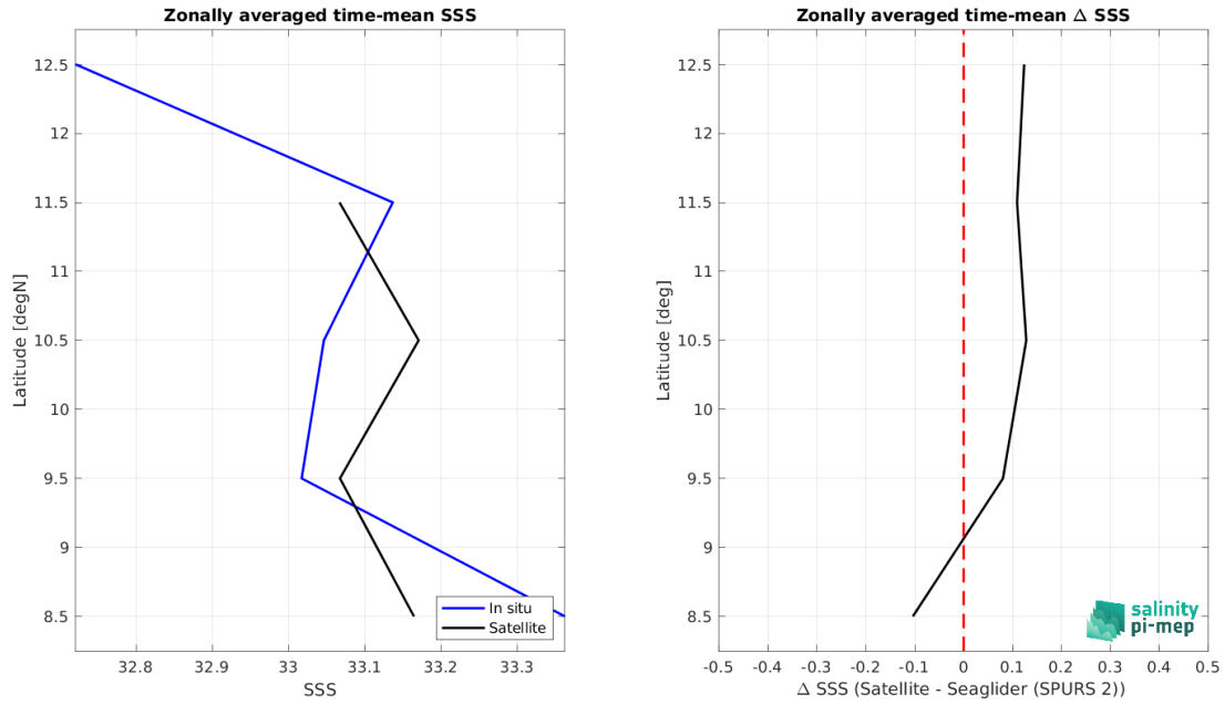
Figure 8: Left panel: Zonal mean SSS from SMOS SSS L3 v9 - 9 Days (CATDS-CEC-LOCEAN) satellite product (black) and from Seaglider (SPURS 2) (blue). Right panel: Zonal mean of \Delta SSS (Satellite - Seaglider (SPURS 2)) for all the collected Pi-MEP match-up pairs estimated over the full satellite product period.
