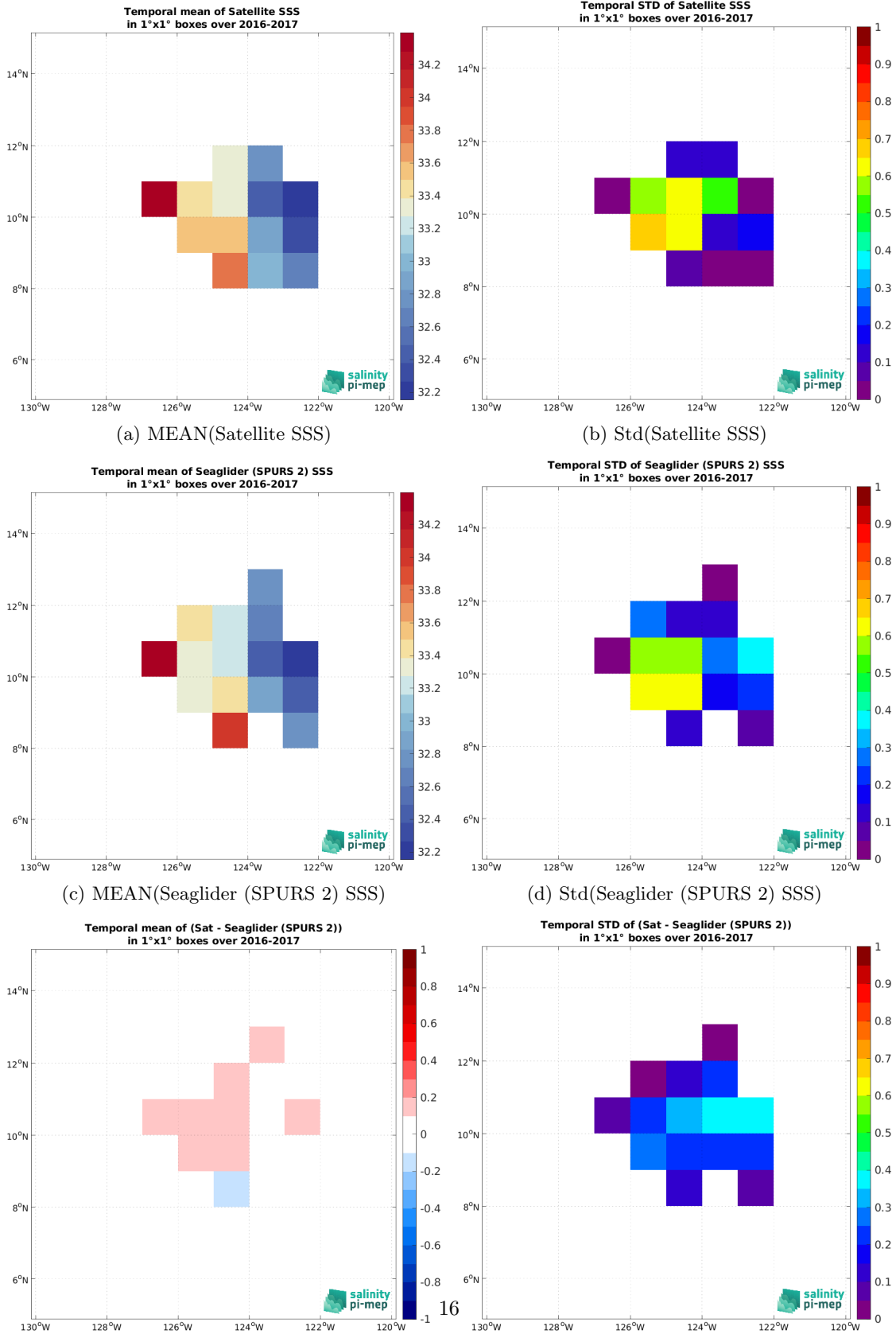
(e) MEAN( \Delta SSS) (Satellite - Seaglider (SPURS 2)) (f) Std( \Delta SSS) (Satellite - Seaglider (SPURS 2)) Figure 6: Temporal mean (left) and Std (right) of SSS from SMOS SSS L3 v9 - 9 Days (CATDS-CEC-LOCEAN) (top), Seaglider (SPURS 2) (middle), and of \Delta SSS (Satellite - Seaglider (SPURS 2)). Only match-up pairs are used to generate these maps.
