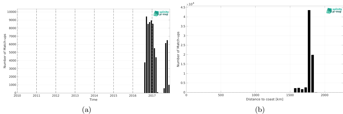
Figure 1: Number of match-ups between Seaglider (SPURS 2) and SMOS SSS L3 v9 - 9 Days (CATDS-CEC-LOCEAN) SSS as a function of time (a) and as function of the distance to coast (b) over the SPURS 2 Pi-MEP region and for the full satellite product period.
