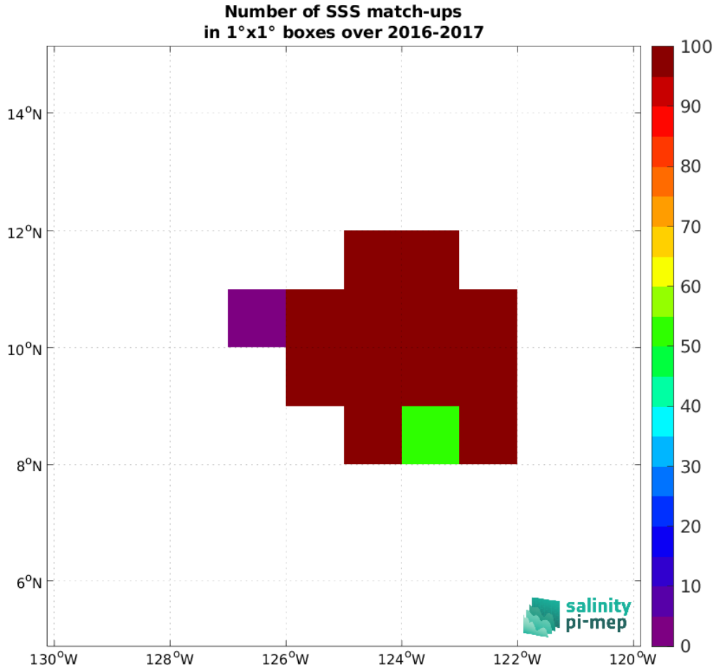
Figure 4: Number of SSS match-ups between Seaglider (SPURS 2) SSS and the SMOS SSS L3 v9 - 9 Days (CATDS-CEC-LOCEAN) SSS product for the SPURS 2 Pi-MEP region over 1^\circ \times 1^\circ boxes and for the full satellite product period.
