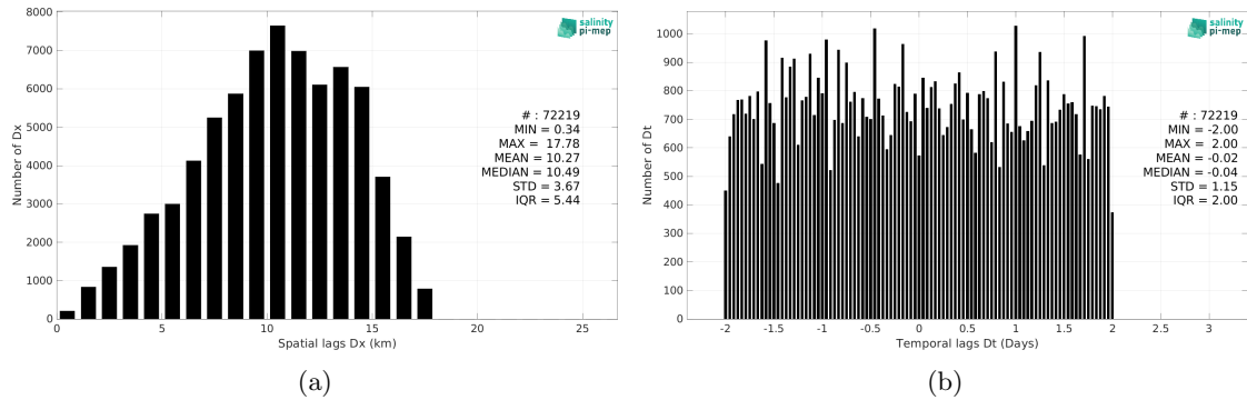
Figure 5: Histograms of the spatial (a) and temporal (b) lags between the location/time of the Seaglider (SPURS 2) measurement and the date of the corresponding SMOS SSS L3 v9 - 9 Days (CATDS-CEC-LOCEAN) SSS pixel.
