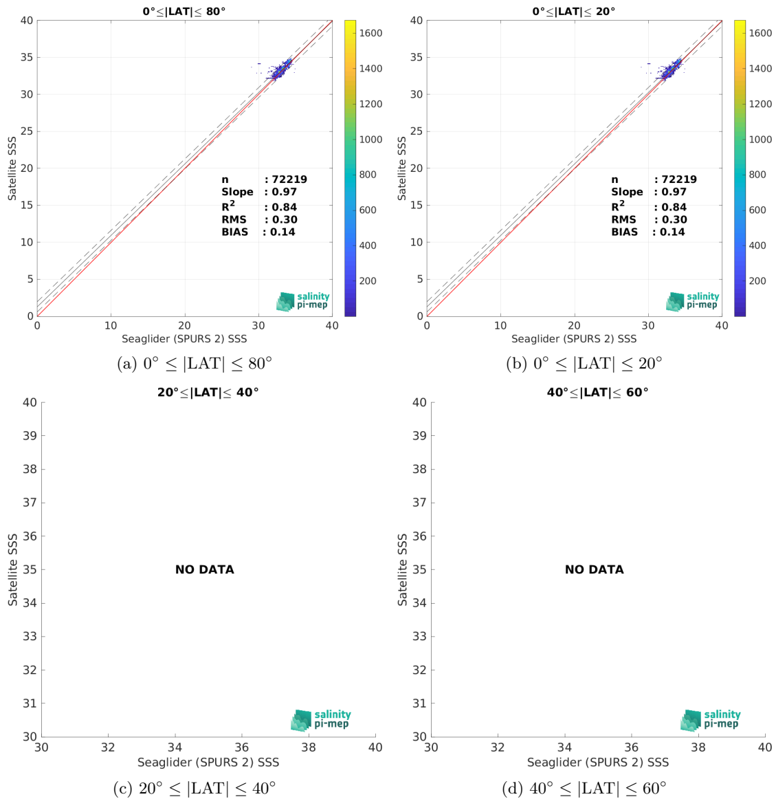
Figure 9: Contour maps of the concentration of SMOS SSS L3 v9 - 9 Days (CATDS-CEC-LOCEAN) SSS (y-axis) versus Seaglider (SPURS 2) SSS (x-axis) at match-up pairs for different latitude bands. For each plot, the red line shows x=y . The black thin and dashed lines indicate a linear fit through the data cloud and the \pm 95\% confidence levels, respectively. The number match-up pairs n , the slope and R^2 coefficient of the linear fit, the root mean square (RMS) and the mean bias between satellite and in situ data are indicated for each latitude band in each plots.
