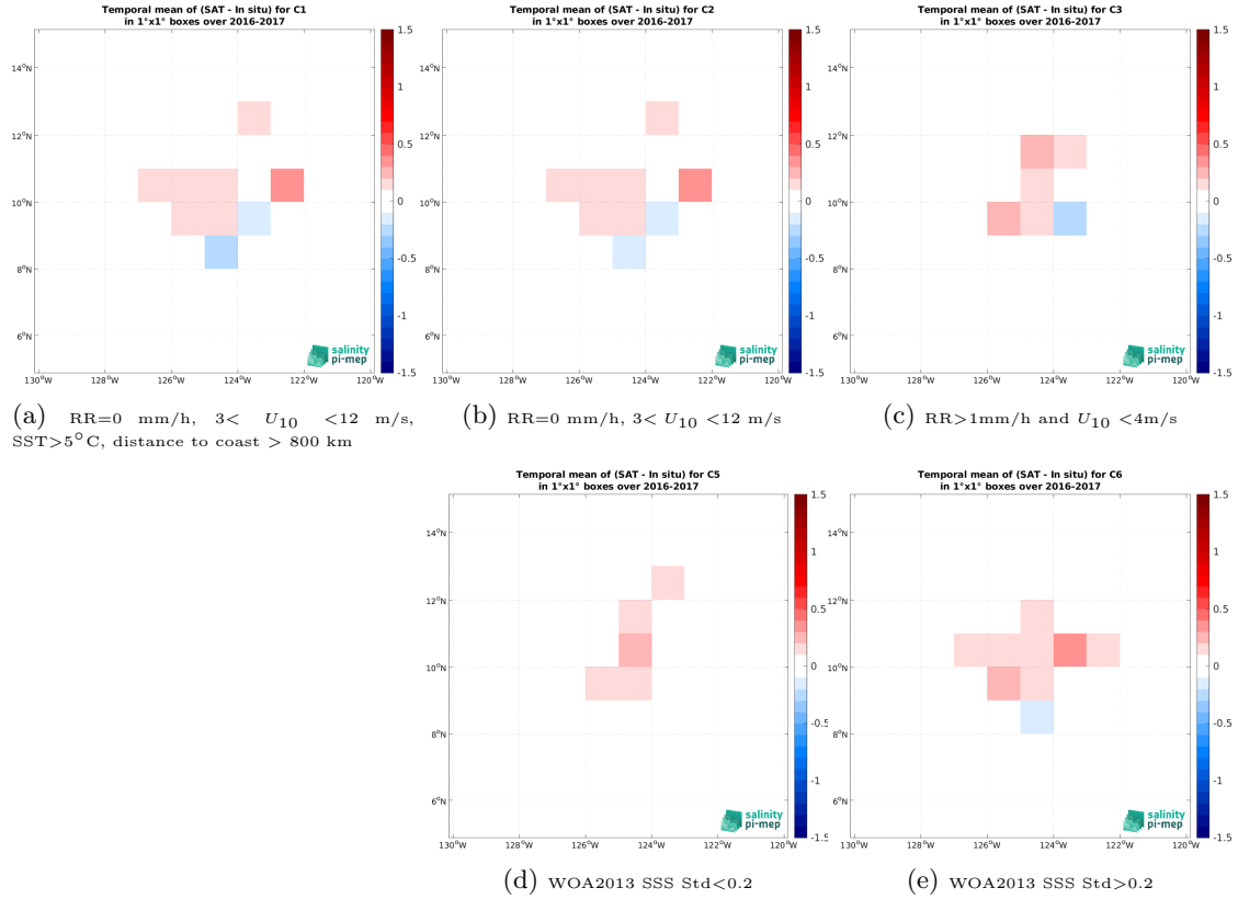
Figure 12: Temporal mean gridded over spatial boxes of size 1^{\circ}\times 1^{\circ} of \Delta\text{SSS} (SMOS SSS L3 v9 - 9 Days (CATDS-CEC-LOCEAN) - Seaglider (SPURS 2)) for 5 different subdatasets corresponding to:RR=0 mm/h, 3 < U_{10} < 12 m/s, SST >5^{\circ}\text{C} , distance to coast > 800 km (a), RR=0 mm/h, 3 < U_{10} < 12 m/s (b), RR >1 mm/h and U_{10} < 4 m/s (c), WOA2013 SSS Std <0.2 (d), WOA2013 SSS Std >0.2 (e).
