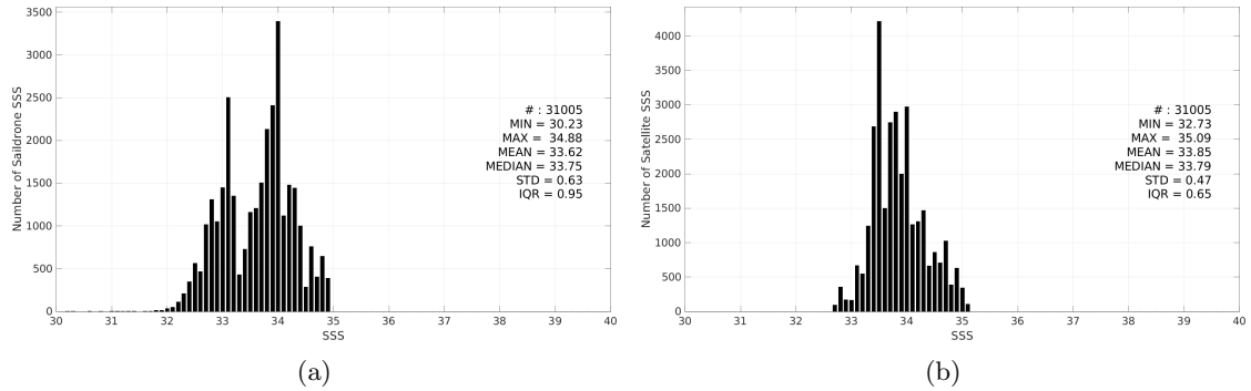
Figure 3: Histograms of SSS from Saildrone (a) and SMOS SSS L3 v9 - 9 Days (CATDS-CEC-LOCEAN) (b) considering all match-up pairs per bins of 0.1 over the SPURS 2 Pi-MEP region and for the full satellite product period.
