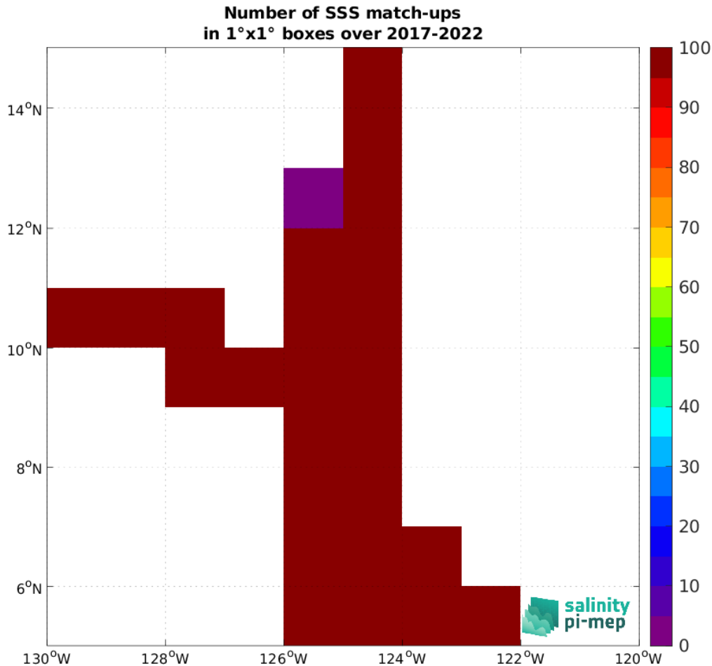
Figure 5: Number of SSS match-ups between Saildrone SSS and the SMOS SSS L3 v9 - 9 Days (CATDS-CEC-LOCEAN) SSS product for the SPURS 2 Pi-MEP region over 1^\circ \times 1^\circ boxes and for the full satellite product period.
