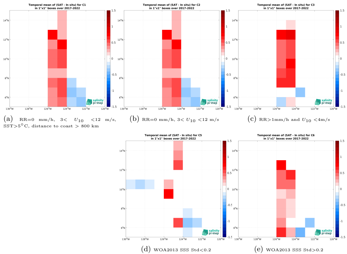
Figure 14: Temporal mean gridded over spatial boxes of size 1^\circ \times 1^\circ of \Delta\text{SSS} (SMOS SSS L3 v9 - 9 Days (CATDS-CEC-LOCEAN) - Saifdrone) for 5 different subdatasets corresponding to:RR=0 mm/h, 3 < U_{10} < 12 m/s, SST>5°C, distance to coast > 800 km (a), RR=0 mm/h, 3 < U_{10} < 12 m/s (b), RR>1mm/h and U_{10} < 4 m/s (c), WOA2013 SSS Std<0.2 (d), WOA2013 SSS Std>0.2 (e).
