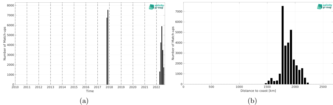
Figure 2: Number of match-ups between Saildrone and SMOS SSS L3 v9 - 9 Days (CATDS-CEC-LOCEAN) SSS as a function of time (a) and as function of the distance to coast (b) over the SPURS 2 Pi-MEP region and for the full satellite product period.
