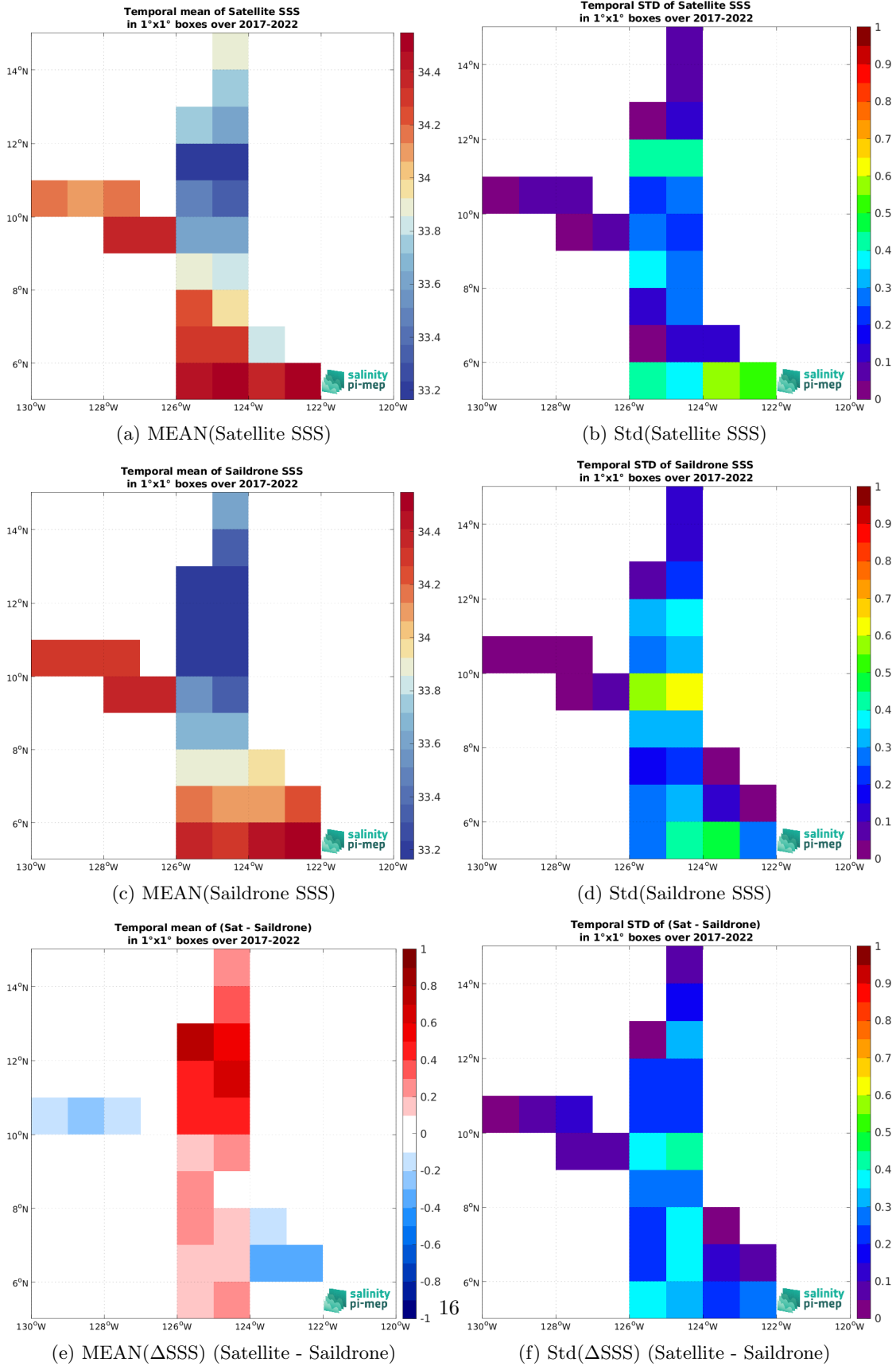
Figure 7: Temporal mean (left) and Std (right) of SSS from SMOS SSS L3 v9 - 9 Days (CATDS-CEC-LOCEAN) (top), Saildrone (middle), and of \Delta SSS (Satellite - Saildrone). Only match-up pairs are used to generate these maps.
