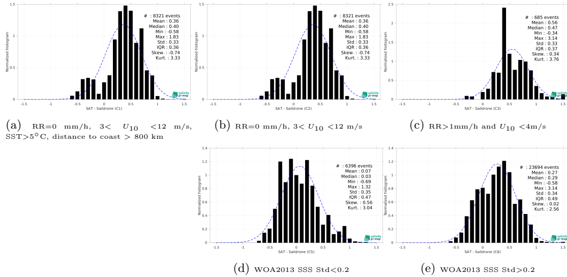
Figure 15: Normalized histogram of \Delta SSS (SMOS SSS L3 v9 - 9 Days (CATDS-CEC-LOCEAN) - Sairdronne) for 5 different subdatasets corresponding to: RR=0 mm/h, 3 < U_{10} < 12 m/s, SST > 5°C, distance to coast > 800 km (a), RR=0 mm/h, 3 < U_{10} < 12 m/s (b), RR > 1mm/h and U_{10} < 4 m/s (c), WOA2013 SSS Std < 0.2 (d), WOA2013 SSS Std > 0.2 (e).
