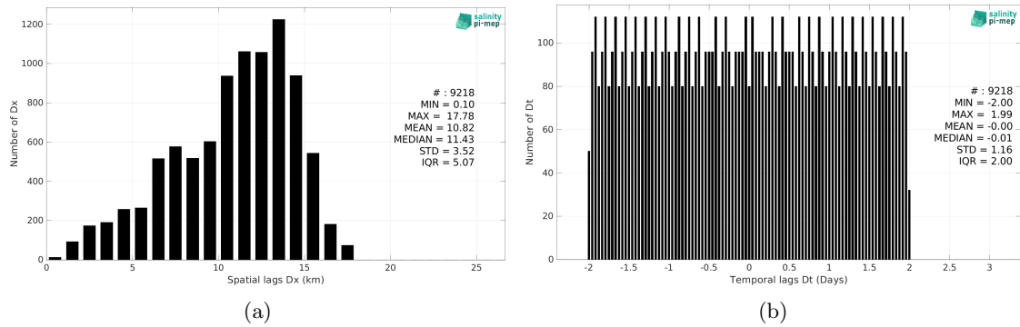
Figure 6: Histograms of the spatial (a) and temporal (b) lags between the location/time of the Saildronne (SPURS 2) measurement and the date of the corresponding SMOS SSS L3 v9 - 9 Days (CATDS-CEC-LOCEAN) SSS pixel.
