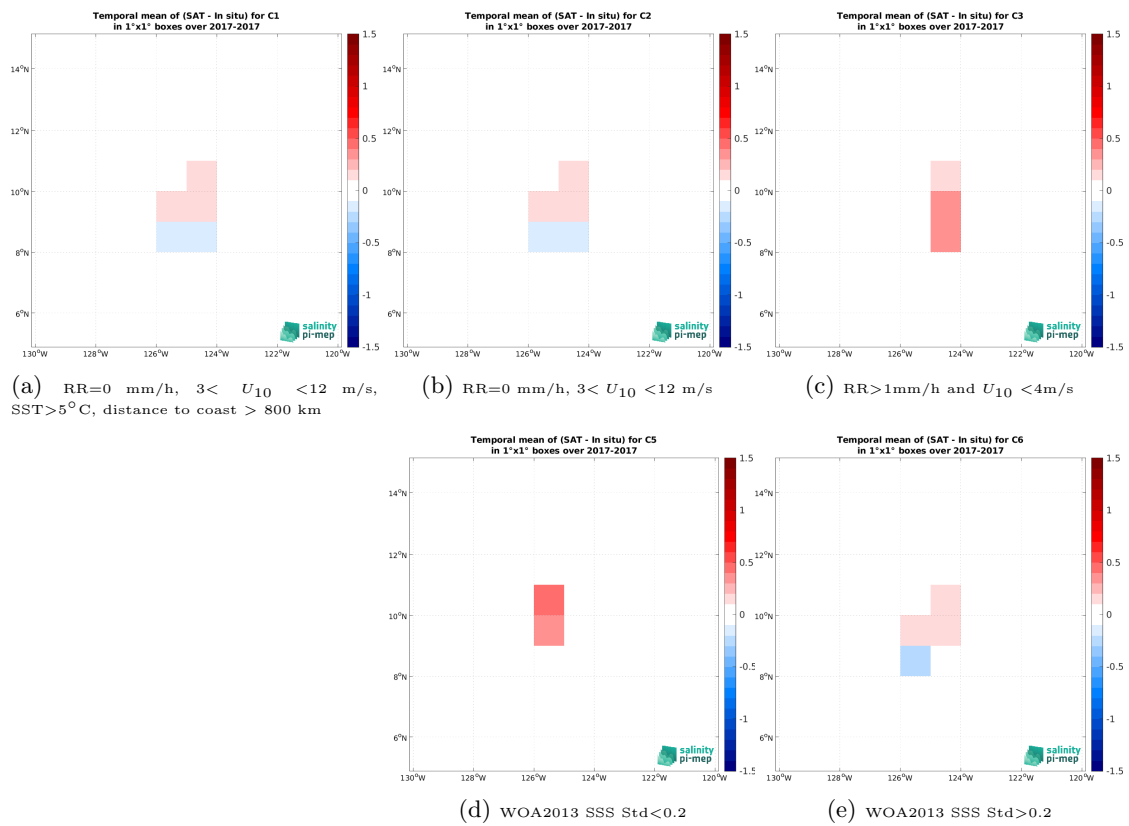
Figure 14: Temporal mean gridded over spatial boxes of size 1^\circ \times 1^\circ of \Delta SSS (SMOS SSS L3 v9 - 9 Days (CATDS-CEC-LOCEAN) - Saildrone (SPURS 2)) for 5 different subdatasets corresponding to:RR=0 mm/h, 3 < U_{10} < 12 m/s, SST >5^\circ C, distance to coast > 800 km (a), RR=0 mm/h, 3 < U_{10} < 12 m/s (b), RR >1 mm/h and U_{10} < 4 m/s (c), WOA2013 SSS Std <0.2 (d), WOA2013 SSS Std >0.2 (e).
