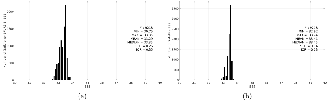
Figure 3: Histograms of SSS from Sairdrone (SPURS 2) (a) and SMOS SSS L3 v9 - 9 Days (CATDS-CEC-LOCEAN) (b) considering all match-up pairs per bins of 0.1 over the SPURS 2 Pi-MEP region and for the full satellite product period.
