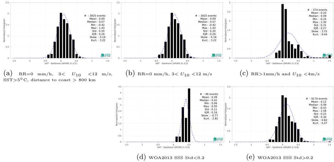
Figure 15: Normalized histogram of \Delta SSS (SMOS SSS L3 v9 - 9 Days (CATDS-CEC-LOCEAN) - Saildrone (SPURS 2)) for 5 different subdatasets corresponding to: RR=0 mm/h, 3 < U_{10} < 12 m/s, SST>5°C, distance to coast > 800 km (a), RR=0 mm/h, 3 < U_{10} < 12 m/s (b), RR>1mm/h and U_{10} < 4 m/s (c), WOA2013 SSS Std<0.2 (d), WOA2013 SSS Std>0.2 (e).
