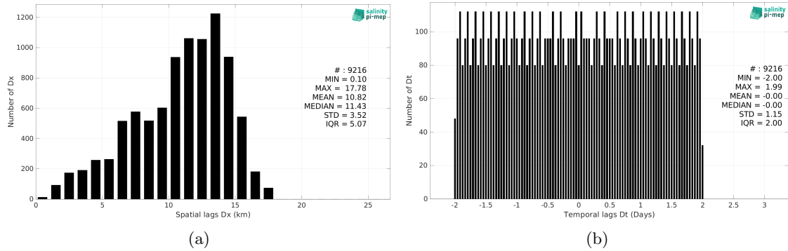
Figure 6: Histograms of the spatial (a) and temporal (b) lags between the location/time of the Saildrone (SPURS 2) measurement and the date of the corresponding SMOS SSS L3 v9 - 9 Days (CATDS-CEC-LOCEAN) SSS pixel.
