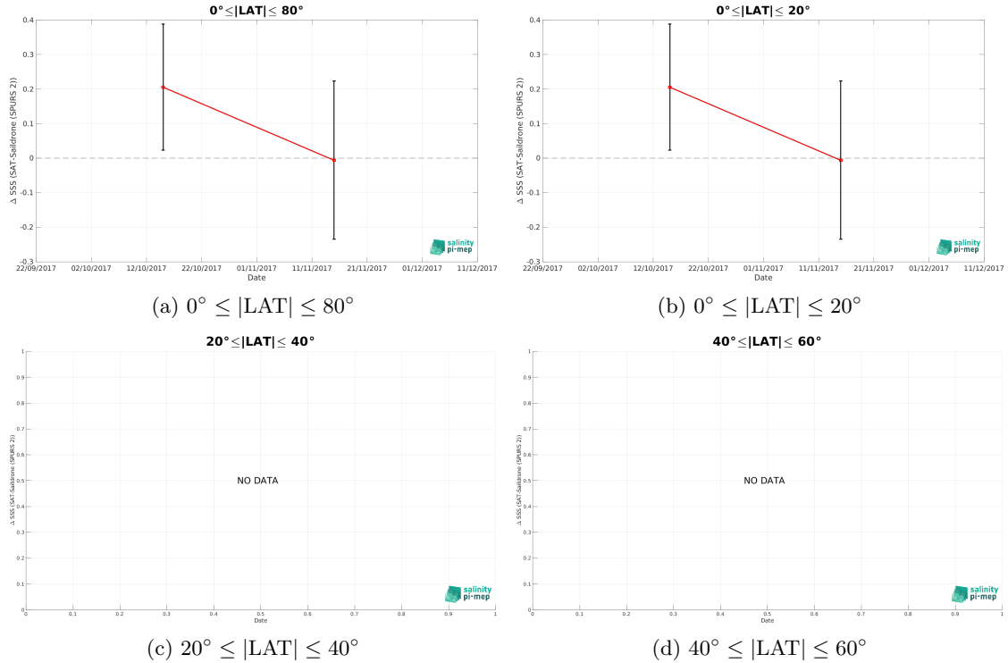
Figure 11: Monthly median (red curves) of \Delta SSS (Satellite - Sairdronne (SPURS 2)) and \pm 1 Std (black vertical thick bars) as function of time for all the collected Pi-MEP match-up pairs estimated over the SPURS 2 Pi-MEP region and for the full satellite product period are shown for different latitude bands: (a) 80^\circ\text{S}-80^\circ\text{N} , (b) 20^\circ\text{S}-20^\circ\text{N} , (c) 40^\circ\text{S}-20^\circ\text{S} and 20^\circ\text{N}-40^\circ\text{N} and (d) 60^\circ\text{S}-40^\circ\text{S} and 40^\circ\text{N}-60^\circ\text{N} .
