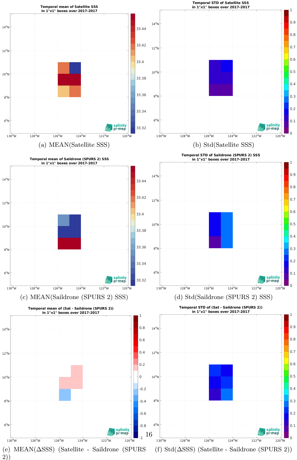
Figure 7: Temporal mean (left) and Std (right) of SSS from SMOS SSS L3 v9 - 9 Days (CATDS-CEC-LOCEAN) (top), Saildrone (SPURS 2) (middle), and of \Delta SSS (Satellite - Saildrone (SPURS 2)). Only match-up pairs are used to generate these maps.
