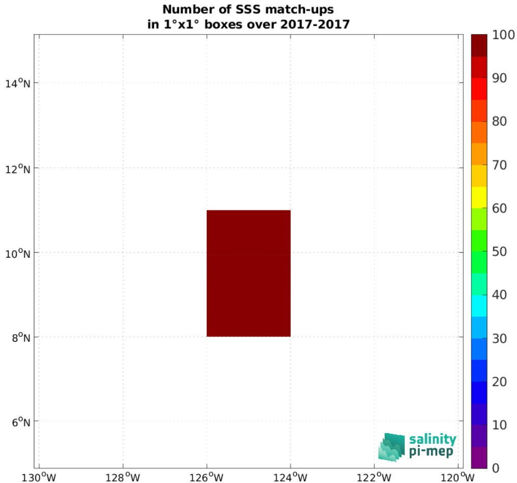
Figure 5: Number of SSS match-ups between Saildrone (SPURS 2) SSS and the SMOS SSS L3 v9 - 9 Days (CATDS-CEC-LOCEAN) SSS product for the SPURS 2 Pi-MEP region over 1^\circ \times 1^\circ boxes and for the full satellite product period.
