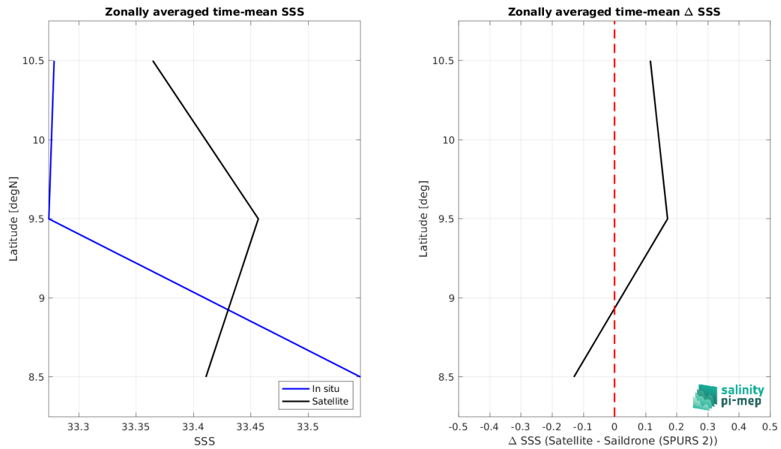
Figure 9: Left panel: Zonal mean SSS from SMOS SSS L3 v9 - 9 Days (CATDS-CEC-LOCEAN) satellite product (black) and from Sairdron (SPURS 2) (blue). Right panel: Zonal mean of \Delta SSS (Satellite - Sairdron (SPURS 2)) for all the collected Pi-MEP match-up pairs estimated over the full satellite product period.
