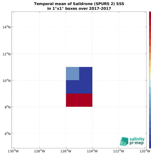
(c) MEAN(Saildrone (SPURS 2) SSS)
