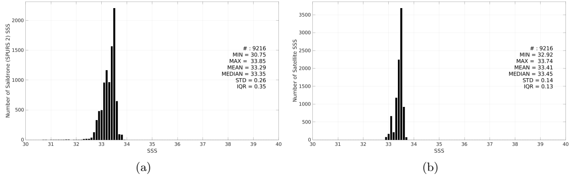
Figure 2: Histograms of SSS from Saildrone (SPURS 2) (a) and SMOS SSS L3 v9 - 9 Days (CATDS-CEC-LOCEAN) (b) considering all match-up pairs per bins of 0.1 over the SPURS 2 Pi-MEP region and for the full satellite product period.
