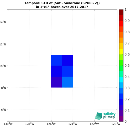
(f) Std( \Delta SSS) (Satellite - Saildrone (SPURS 2))
