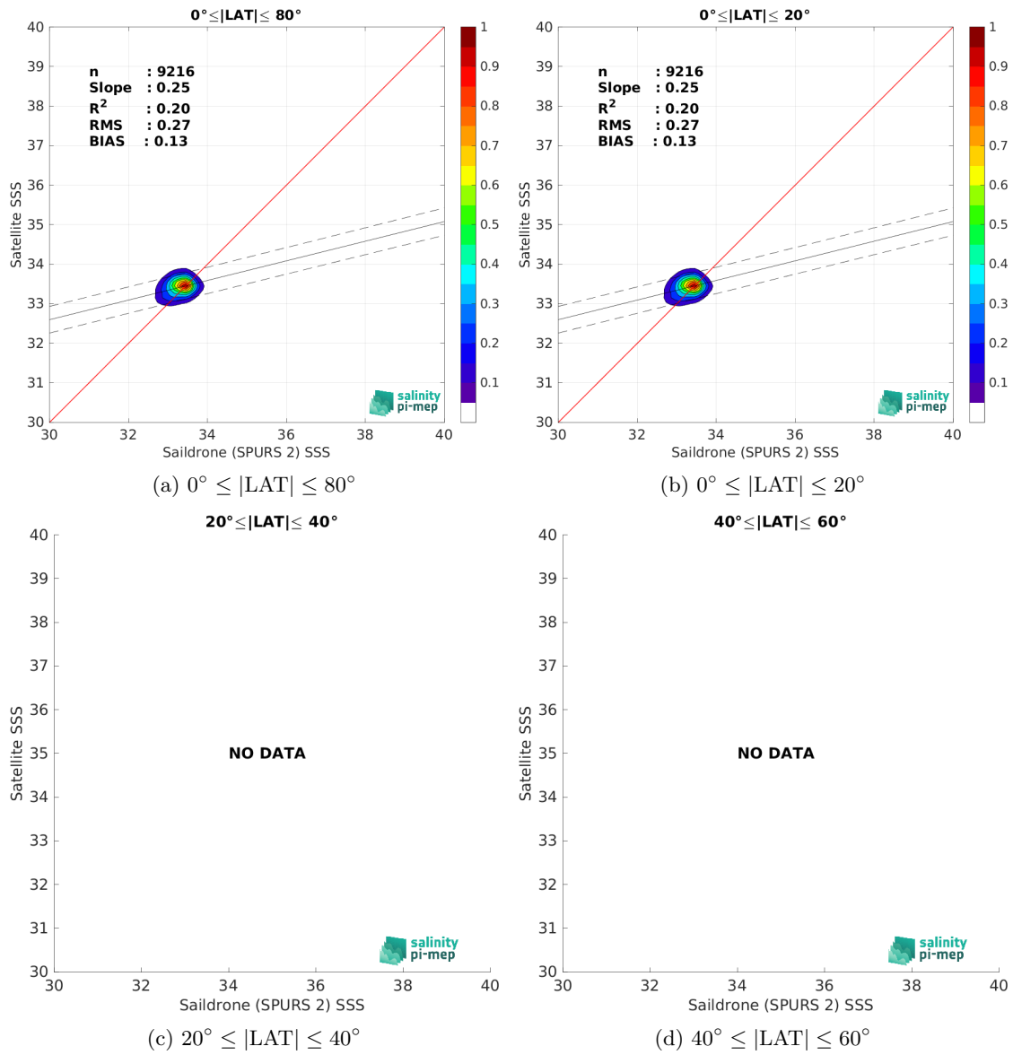
Figure 9: Contour maps of the concentration of SMOS SSS L3 v9 - 9 Days (CATDS-CEC-LOCEAN) SSS (y-axis) versus Saildrone (SPURS 2) SSS (x-axis) at match-up pairs for different latitude bands. For each plot, the red line shows x=y . The black thin and dashed lines indicate a linear fit through the data cloud and the \pm 95\% confidence levels, respectively. The number match-up pairs n , the slope and R^2 coefficient of the linear fit, the root mean square (RMS) and the mean bias between satellite and in situ data are indicated for each latitude band in each plots.
