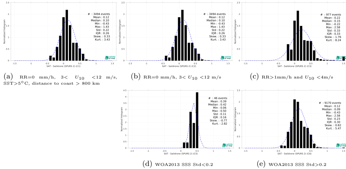
Figure 13: Normalized histogram of \Delta SSS (SMOS SSS L3 v9 - 9 Days (CATDS-CEC-LOCEAN) - Saildrone (SPURS 2)) for 5 different subdatasets corresponding to: RR=0 mm/h, 3 < U_{10} < 12 m/s, SST > 5°C, distance to coast > 800 km (a), RR=0 mm/h, 3 < U_{10} < 12 m/s (b), RR > 1mm/h and U_{10} < 4 m/s (c), WOA2013 SSS Std < 0.2 (d), WOA2013 SSS Std > 0.2 (e).
