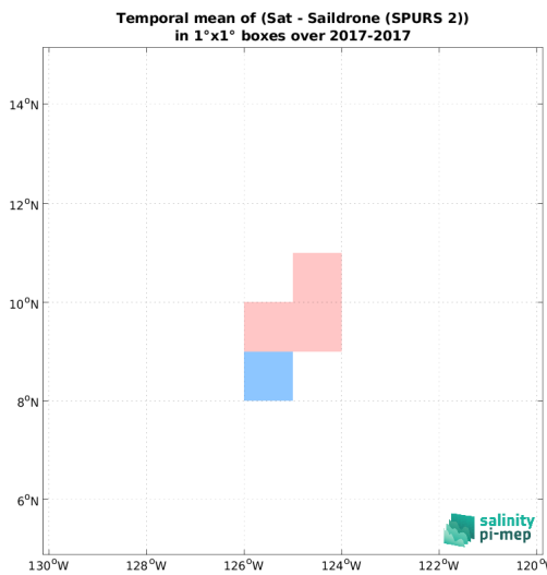
(e) MEAN( \Delta SSS) (Satellite - Saildrone (SPURS 2))
