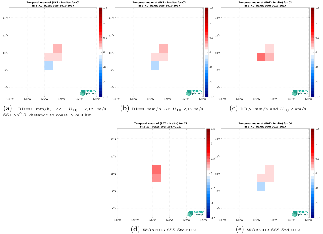
Figure 12: Temporal mean gridded over spatial boxes of size 1^{\circ}\times 1^{\circ} of \Delta\text{SSS} (SMOS SSS L3 v9 - 9 Days (CATDS-CEC-LOCEAN) - Sailability (SPURS 2)) for 5 different subdatasets corresponding to:RR=0 mm/h, 3 < U_{10} < 12 m/s, SST >5^{\circ}\text{C} , distance to coast > 800 km (a), RR=0 mm/h, 3 < U_{10} < 12 m/s (b), RR >1 mm/h and U_{10} < 4 m/s (c), WOA2013 SSS Std <0.2 (d), WOA2013 SSS Std >0.2 (e).
