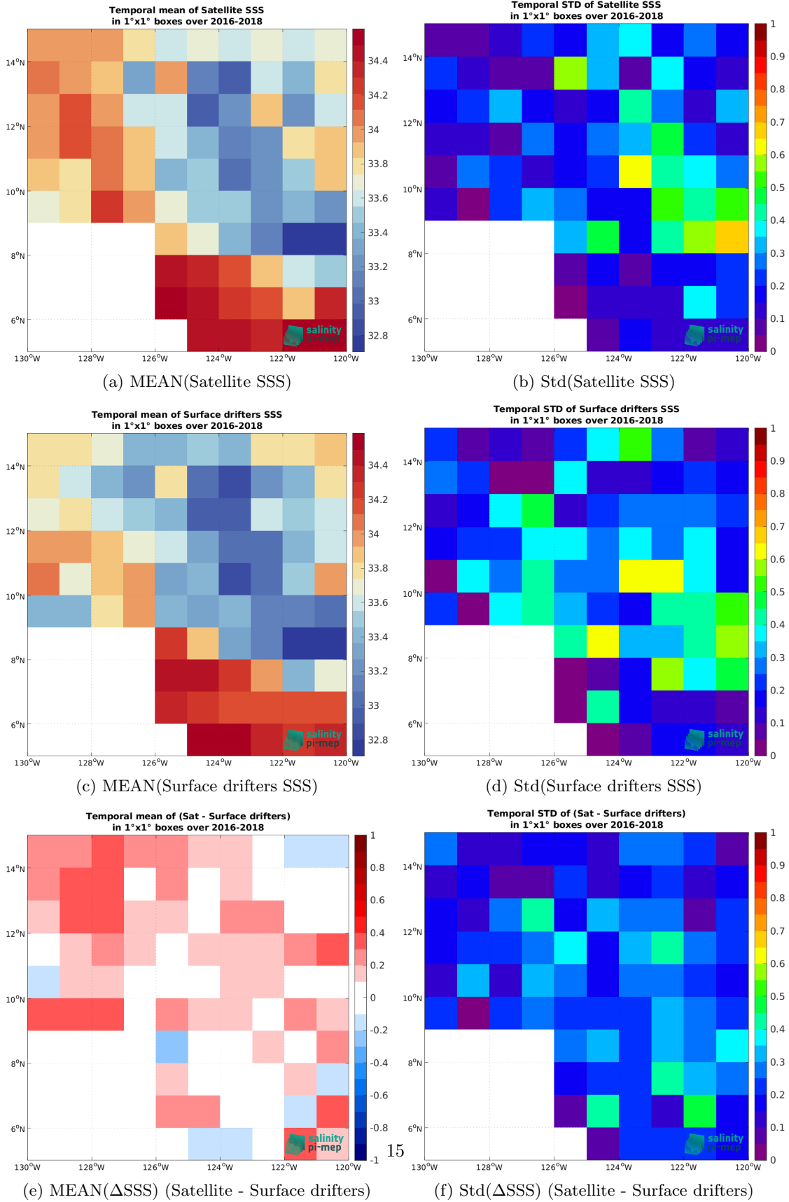
Figure 5: Temporal mean (left) and Std (right) of SSS from SMOS SSS L3 v9 - 9 Days (CATDS-CEC-LOCEAN) (top), Surface drifters (middle), and of \Delta SSS (Satellite - Surface drifters). Only match-up pairs are used to generate these maps.
