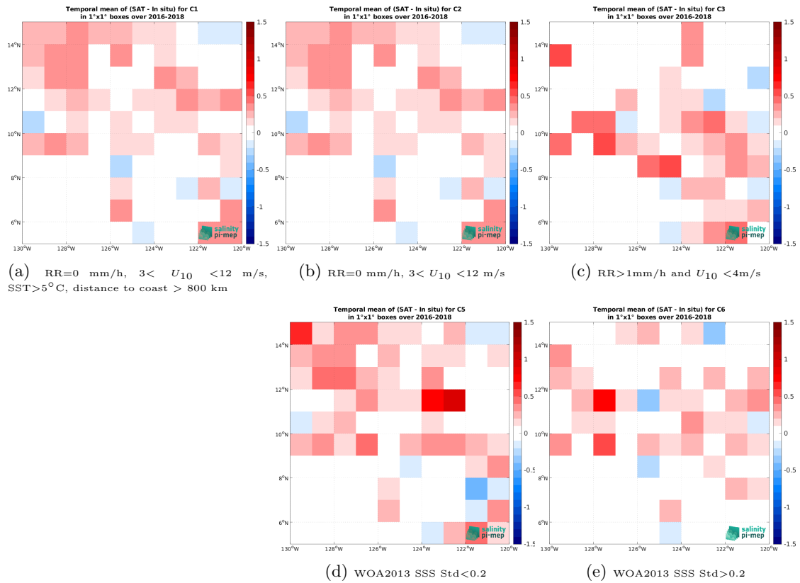
Figure 11: Temporal mean gridded over spatial boxes of size 1^\circ \times 1^\circ of \Delta SSS (SMOS SSS L3 v9 - 9 Days (CATDS-CEC-LOCEAN) - Surface drifters) for 5 different subdatasets corresponding to: RR=0 mm/h, 3 < U_{10} < 12 m/s, SST > 5^\circ\text{C} , distance to coast > 800 km (a), RR=0 mm/h, 3 < U_{10} < 12 m/s (b), RR > 1 mm/h and U_{10} < 4 m/s (c), WOA2013 SSS Std < 0.2 (d), WOA2013 SSS Std > 0.2 (e).
