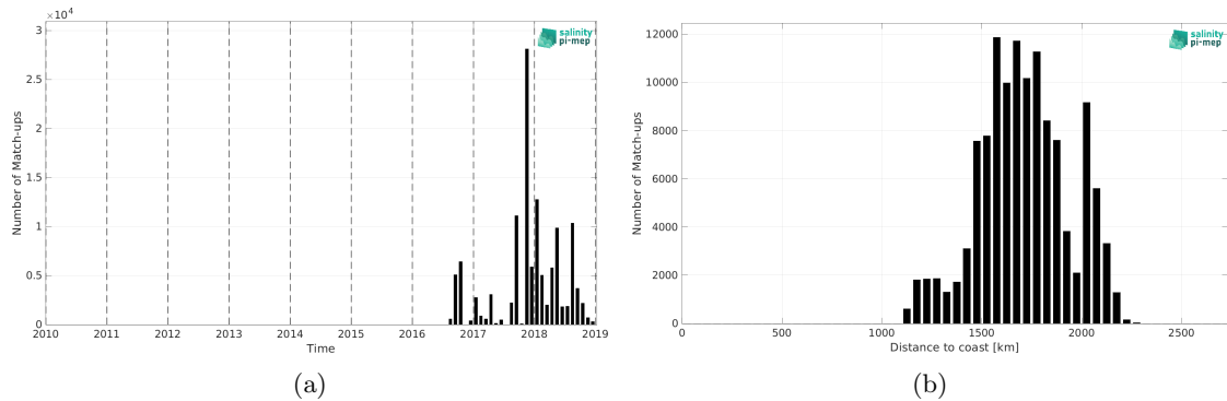
Figure 1: Number of match-ups between Surface drifters and SMOS SSS L3 v9 - 9 Days (CATDS-CEC-LOCEAN) SSS as a function of time (a) and as function of the distance to coast (b) over the SPURS 2 Pi-MEP region and for the full satellite product period.
