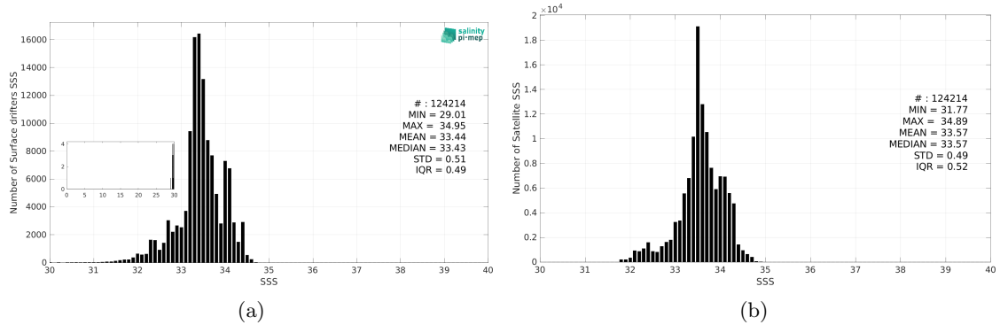
Figure 2: Histograms of SSS from Surface drifters (a) and SMOS SSS L3 v9 - 9 Days (CATDS-CEC-LOCEAN) (b) considering all match-up pairs per bins of 0.1 over the SPURS 2 Pi-MEP region and for the full satellite product period.
