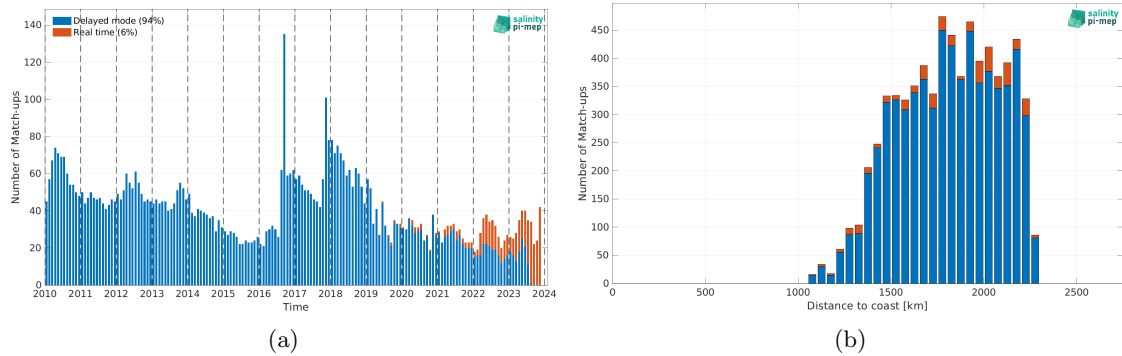
Figure 2: Number of match-ups between Argo and SMOS SSS L3 v9 - 9 Days (CATDS-CEC-LOCEAN) SSS as a function of time (a) and as function of the distance to coast (b) over the SPURS 2 Pi-MEP region and for the full satellite product period.
