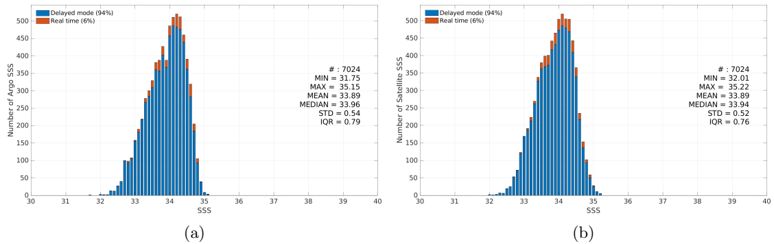
Figure 3: Histograms of SSS from Argo (a) and SMOS SSS L3 v9 - 9 Days (CATDS-CEC-LOCEAN) (b) considering all match-up pairs per bins of 0.1 over the SPURS 2 Pi-MEP region and for the full satellite product period.
