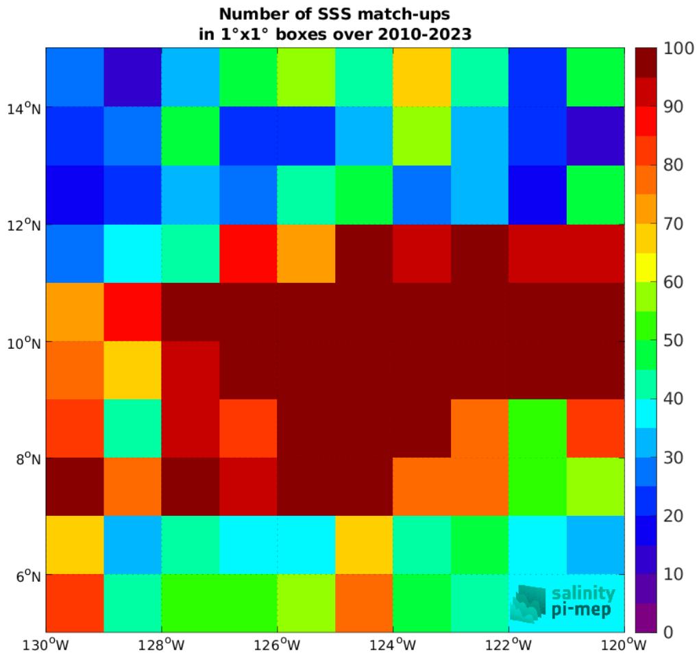
Figure 5: Number of SSS match-ups between Argo SSS and the SMOS SSS L3 v9 - 9 Days (CATDS-CEC-LOCEAN) SSS product for the SPURS 2 Pi-MEP region over 1°x1° boxes and for the full satellite product period.
