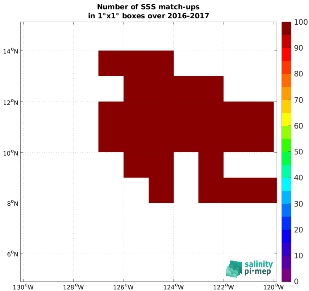
Figure 5: Number of SSS match-ups between Waveglider (SPURS 2) SSS and the SMOS SSS L3 v9 - 18 Days (CATDS-CEC-LOCEAN) SSS product for the SPURS 2 Pi-MEP region over 1^\circ \times 1^\circ boxes and for the full satellite product period.
