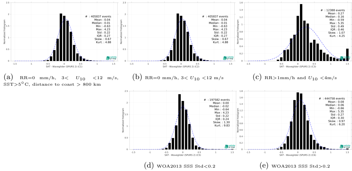
Figure 15: Normalized histogram of \Delta SSS (SMOS SSS L3 v9 - 18 Days (CATDS-CEC-LOCEAN) - Waveglider (SPURS 2)) for 5 different subdatasets corresponding to: RR=0 mm/h, 3 < U_{10} < 12 m/s, SST>5°C, distance to coast > 800 km (a), RR=0 mm/h, 3 < U_{10} < 12 m/s (b), RR>1mm/h and U_{10} < 4 m/s (c), WOA2013 SSS Std<0.2 (d), WOA2013 SSS Std>0.2 (e).
