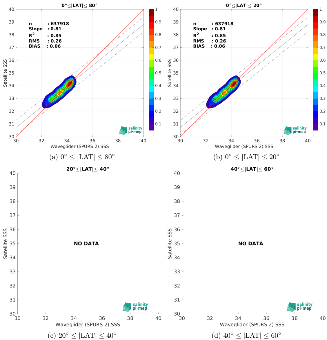
Figure 10: Contour maps of the concentration of SMOS SSS L3 v9 - 18 Days (CATDS-CEC-LOCEAN) SSS (y-axis) versus Waveglider (SPURS 2) SSS (x-axis) at match-up pairs for different latitude bands. For each plot, the red line shows x=y . The black thin and dashed lines indicate a linear fit through the data cloud and the \pm 95\% confidence levels, respectively. The number match-up pairs n , the slope and R^2 coefficient of the linear fit, the root mean square (RMS) and the mean bias between satellite and in situ data are indicated for each latitude band in each plots.
