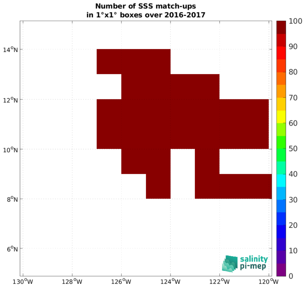
Figure 5: Number of SSS match-ups between Waveglider (SPURS 2) SSS and the SMOS SSS L3 v9 - 18 Days (CATDS-CEC-LOCEAN) SSS product for the SPURS 2 Pi-MEP region over 1°x1° boxes and for the full satellite product period.
