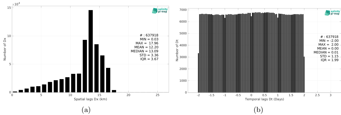
Figure 6: Histograms of the spatial (a) and temporal (b) lags between the location/time of the Waveglider (SPURS 2) measurement and the date of the corresponding SMOS SSS L3 v9 - 18 Days (CATDS-CEC-LOCEAN) SSS pixel.
