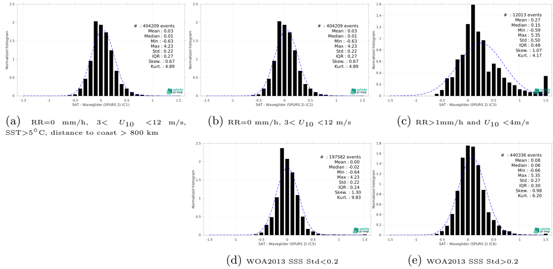
Figure 15: Normalized histogram of \Delta SSS (SMOS SSS L3 v9 - 18 Days (CATDS-CEC-LOCEAN) - Waveglider (SPURS 2)) for 5 different subdatasets corresponding to: RR=0 mm/h, 3 < U_{10} < 12 m/s, SST > 5°C, distance to coast > 800 km (a), RR=0 mm/h, 3 < U_{10} < 12 m/s (b), RR > 1mm/h and U_{10} < 4 m/s (c), WOA2013 SSS Std < 0.2 (d), WOA2013 SSS Std > 0.2 (e).
