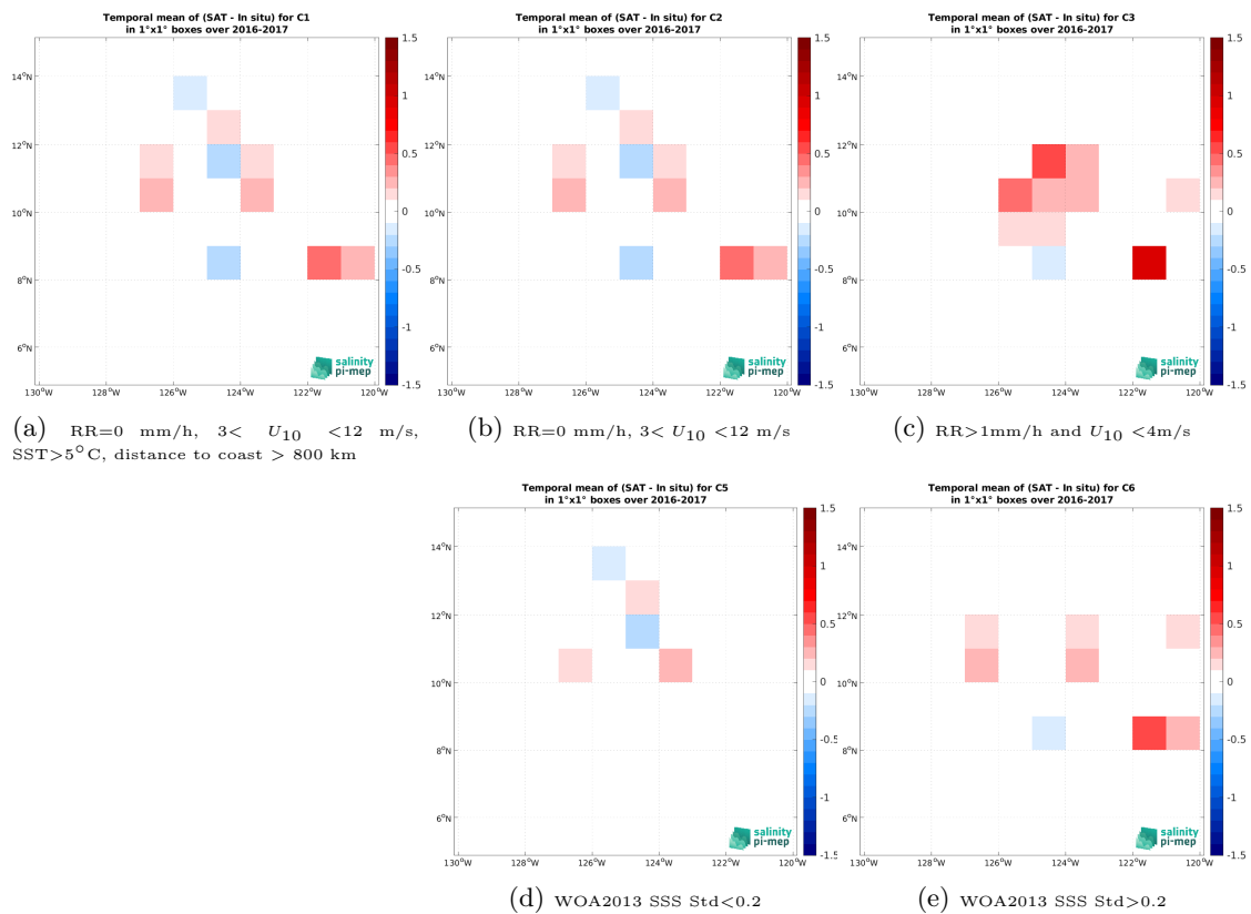
Figure 14: Temporal mean gridded over spatial boxes of size 1^\circ \times 1^\circ of \Delta SSS (SMOS SSS L3 v9 - 18 Days (CATDS-CEC-LOCEAN) - Waveglider (SPURS 2)) for 5 different subdatasets corresponding to:RR=0 mm/h, 3 < U_{10} < 12 m/s, SST >5^\circ C, distance to coast > 800 km (a), RR=0 mm/h, 3 < U_{10} < 12 m/s (b), RR >1 mm/h and U_{10} < 4 m/s (c), WOA2013 SSS Std <0.2 (d), WOA2013 SSS Std >0.2 (e).
