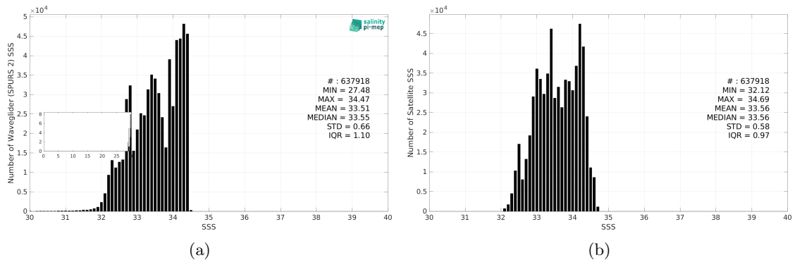
Figure 3: Histograms of SSS from Waveglider (SPURS 2) (a) and SMOS SSS L3 v9 - 18 Days (CATDS-CEC-LOCEAN) (b) considering all match-up pairs per bins of 0.1 over the SPURS 2 Pi-MEP region and for the full satellite product period.
