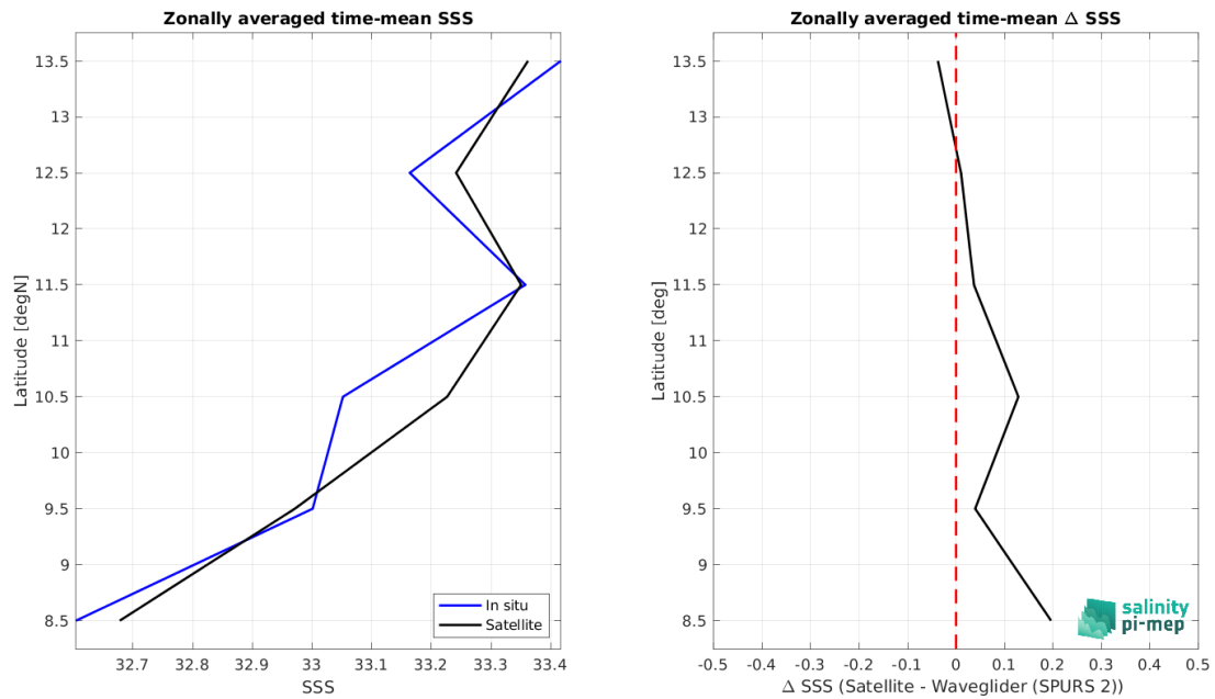
Figure 8: Left panel: Zonal mean SSS from SMOS SSS L3 v9 - 18 Days (CATDS-CEC-LOCEAN) satellite product (black) and from Waveglider (SPURS 2) (blue). Right panel: Zonal mean of \Delta SSS (Satellite - Waveglider (SPURS 2)) for all the collected Pi-MEP match-up pairs estimated over the full satellite product period.
