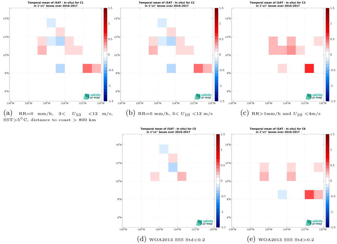
Figure 12: Temporal mean gridded over spatial boxes of size 1^{\circ}\times 1^{\circ} of \Delta\text{SSS} (SMOS SSS L3 v9 - 18 Days (CATDS-CEC-LOCEAN) - Waveglider (SPURS 2)) for 5 different subdatasets corresponding to:RR=0 mm/h, 3 < U_{10} < 12 m/s, SST >5^{\circ}\text{C} , distance to coast > 800 km (a), RR=0 mm/h, 3 < U_{10} < 12 m/s (b), RR >1 mm/h and U_{10} < 4 m/s (c), WOA2013 SSS Std <0.2 (d), WOA2013 SSS Std >0.2 (e).
