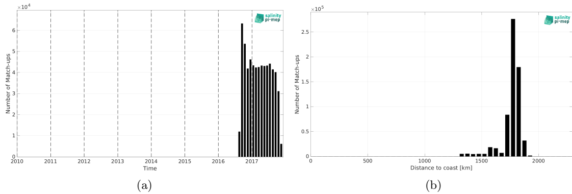
Figure 1: Number of match-ups between Waveglider (SPURS 2) and SMOS SSS L3 v9 - 18 Days (CATDS-CEC-LOCEAN) SSS as a function of time (a) and as function of the distance to coast (b) over the SPURS 2 Pi-MEP region and for the full satellite product period.
