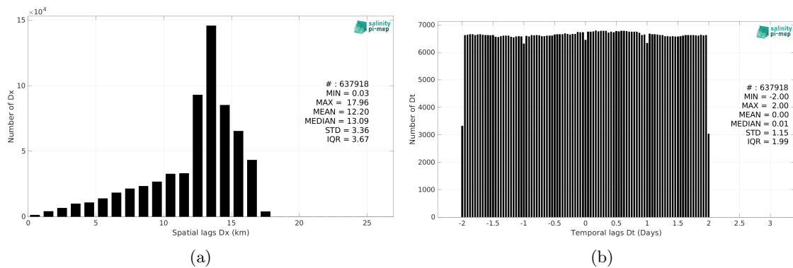
Figure 5: Histograms of the spatial (a) and temporal (b) lags between the location/time of the Waveglider (SPURS 2) measurement and the date of the corresponding SMOS SSS L3 v9 - 18 Days (CATDS-CEC-LOCEAN) SSS pixel.
