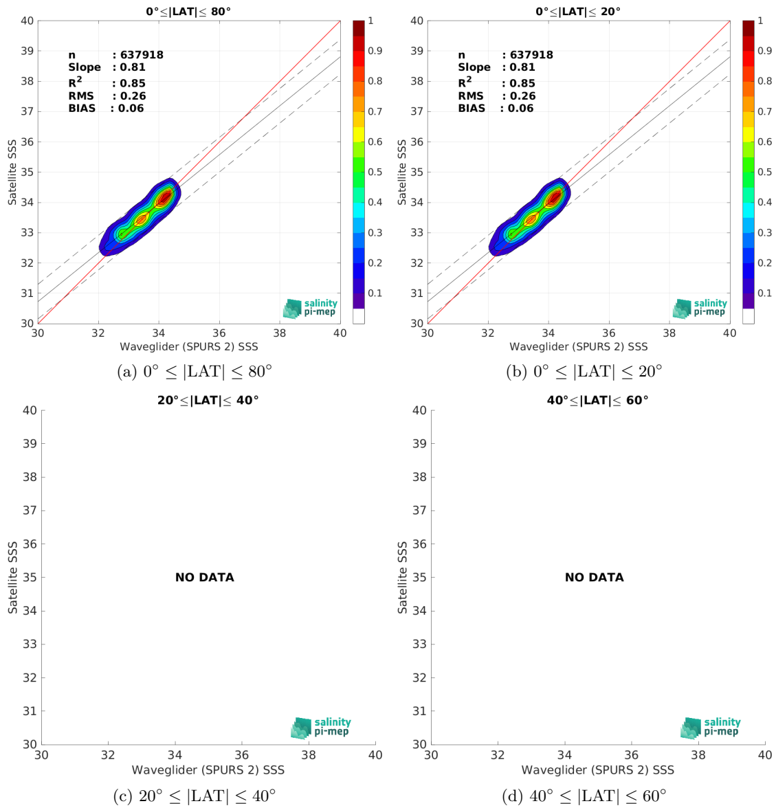
Figure 9: Contour maps of the concentration of SMOS SSS L3 v9 - 18 Days (CATDS-CEC-LOCEAN) SSS (y-axis) versus Waveglider (SPURS 2) SSS (x-axis) at match-up pairs for different latitude bands. For each plot, the red line shows x=y . The black thin and dashed lines indicate a linear fit through the data cloud and the \pm 95\% confidence levels, respectively. The number match-up pairs n , the slope and R^2 coefficient of the linear fit, the root mean square (RMS) and the mean bias between satellite and in situ data are indicated for each latitude band in each plots.
