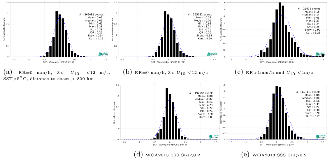
Figure 13: Normalized histogram of \Delta\text{SSS} (SMOS SSS L3 v9 - 18 Days (CATDS-CEC-LOCEAN) - Waveglider (SPURS 2)) for 5 different subdatasets corresponding to: RR=0 mm/h, 3 < U_{10} < 12 m/s, SST >5^{\circ}\text{C} , distance to coast > 800 km (a), RR=0 mm/h, 3 < U_{10} < 12 m/s (b), RR >1 mm/h and U_{10} < 4 m/s (c), WOA2013 SSS Std <0.2 (d), WOA2013 SSS Std >0.2 (e).
