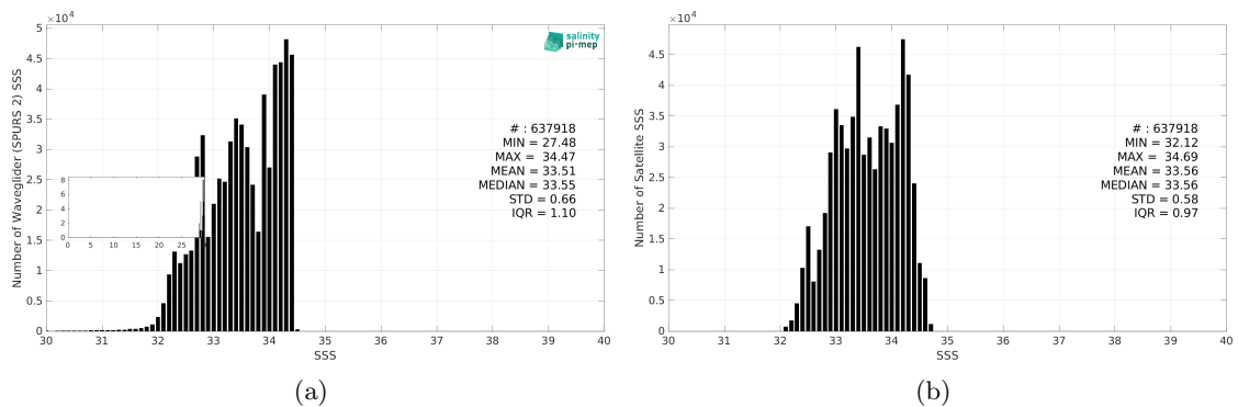
Figure 2: Histograms of SSS from Waveglider (SPURS 2) (a) and SMOS SSS L3 v9 - 18 Days (CATDS-CEC-LOCEAN) (b) considering all match-up pairs per bins of 0.1 over the SPURS 2 Pi-MEP region and for the full satellite product period.
