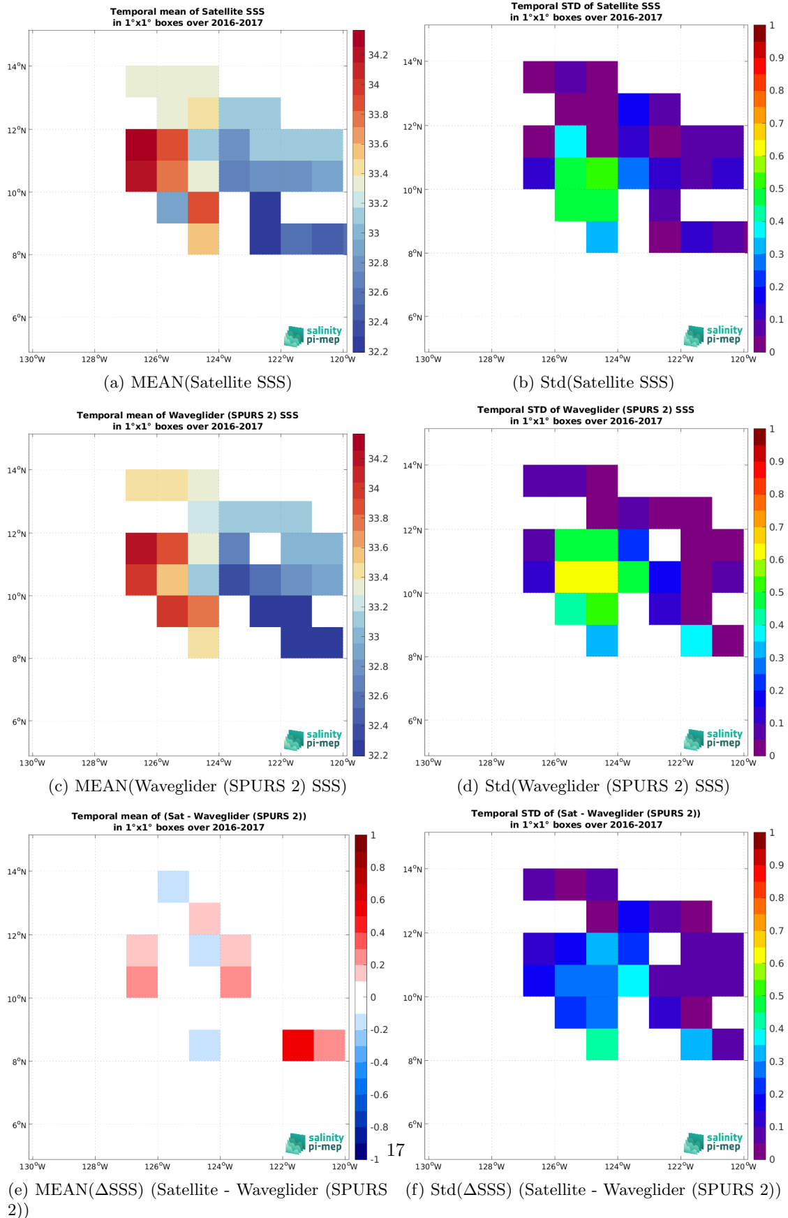
Figure 6: Temporal mean (left) and Std (right) of SSS from SMOS SSS L3 v9 - 18 Days (CATDS-CEC-LOCEAN) (top), Waveglider (SPURS 2) (middle), and of \Delta SSS (Satellite - Waveglider (SPURS 2)). Only match-up pairs are used to generate these maps.
