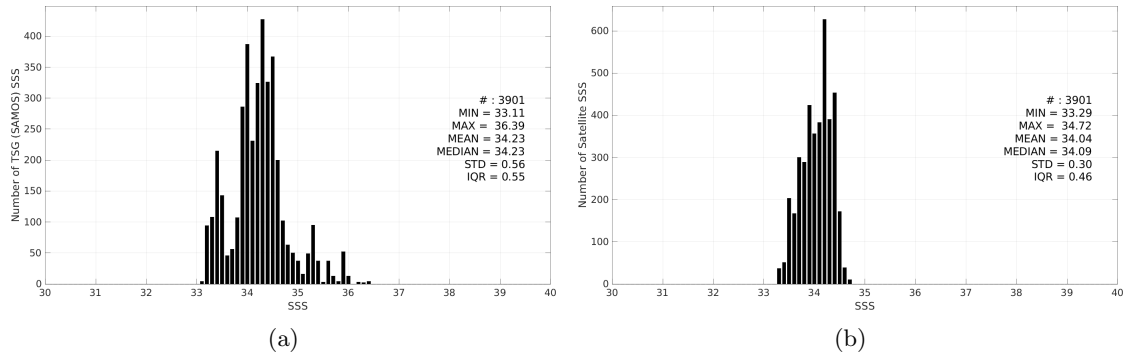
Figure 3: Histograms of SSS from TSG (SAMOS) (a) and SMOS SSS L3 v9 - 18 Days (CATDS-CEC-LOCEAN) (b) considering all match-up pairs per bins of 0.1 over the SPURS 2 Pi-MEP region and for the full satellite product period.
