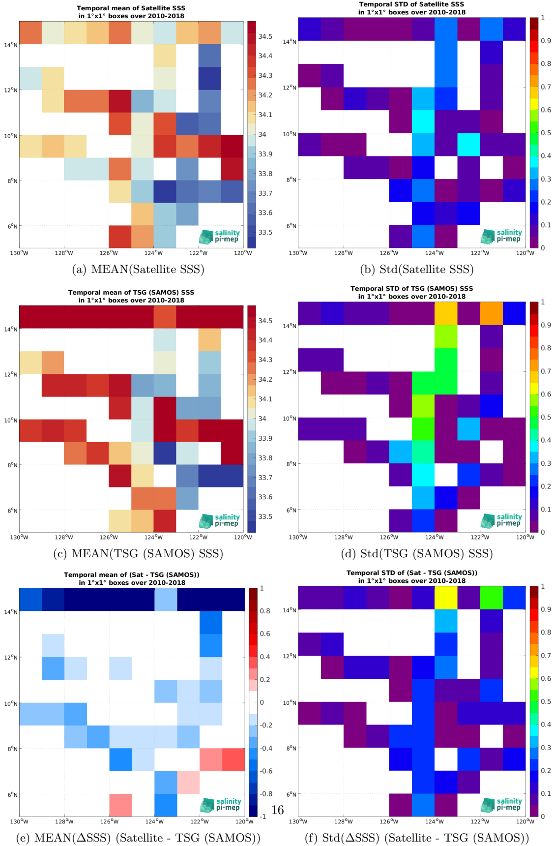
Figure 7: Temporal mean (left) and Std (right) of SSS from SMOS SSS L3 v9 - 18 Days (CATDS-CEC-LOCEAN) (top), TSG (SAMOS) (middle), and of \Delta SSS (Satellite - TSG (SAMOS)). Only match-up pairs are used to generate these maps.
