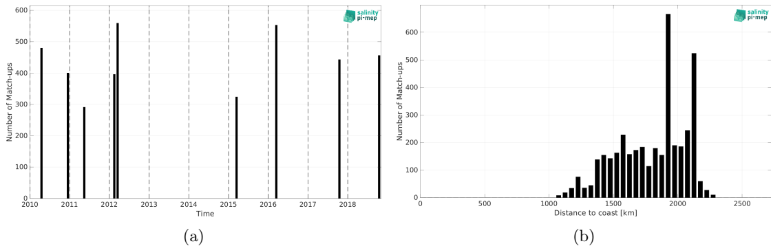
Figure 2: Number of match-ups between TSG (SAMOS) and SMOS SSS L3 v9 - 18 Days (CATDS-CEC-LOCEAN) SSS as a function of time (a) and as function of the distance to coast (b) over the SPURS 2 Pi-MEP region and for the full satellite product period.
