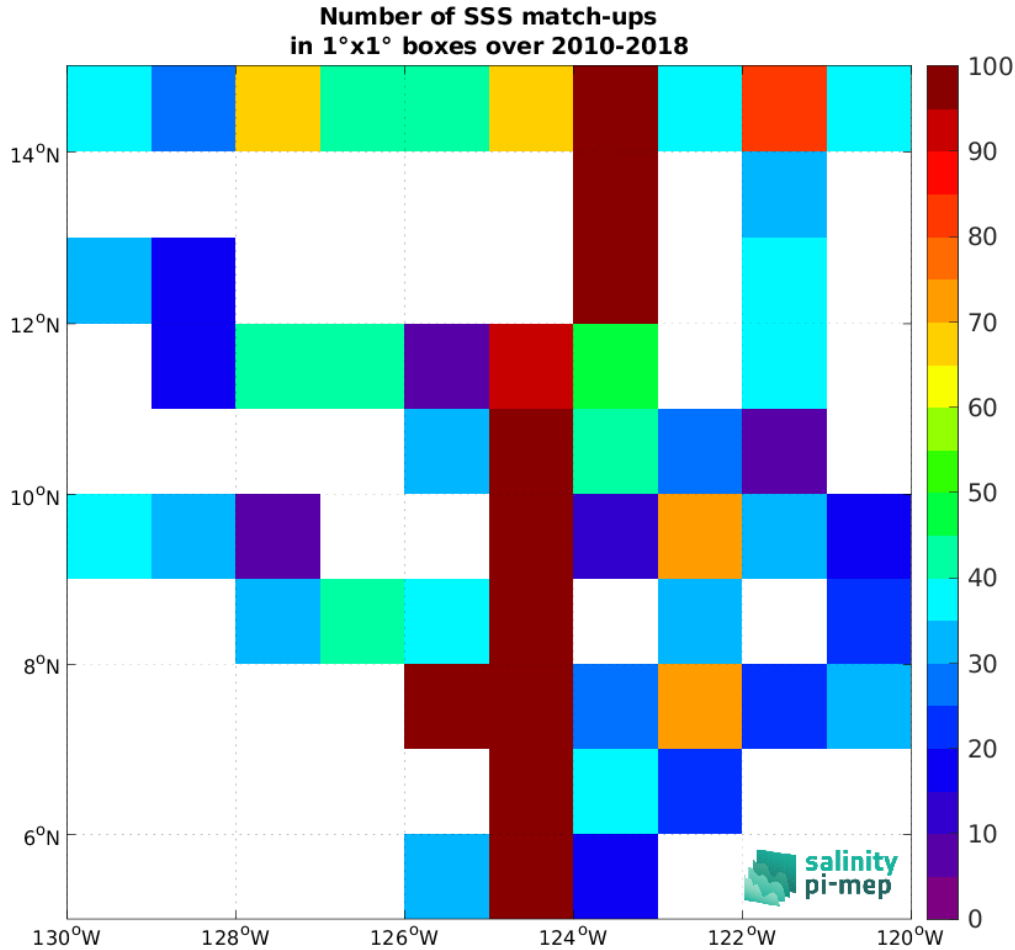
Figure 5: Number of SSS match-ups between TSG (SAMOS) SSS and the SMOS SSS L3 v9 - 18 Days (CATDS-CEC-LOCEAN) SSS product for the SPURS 2 Pi-MEP region over 1^\circ \times 1^\circ boxes and for the full satellite product period.
