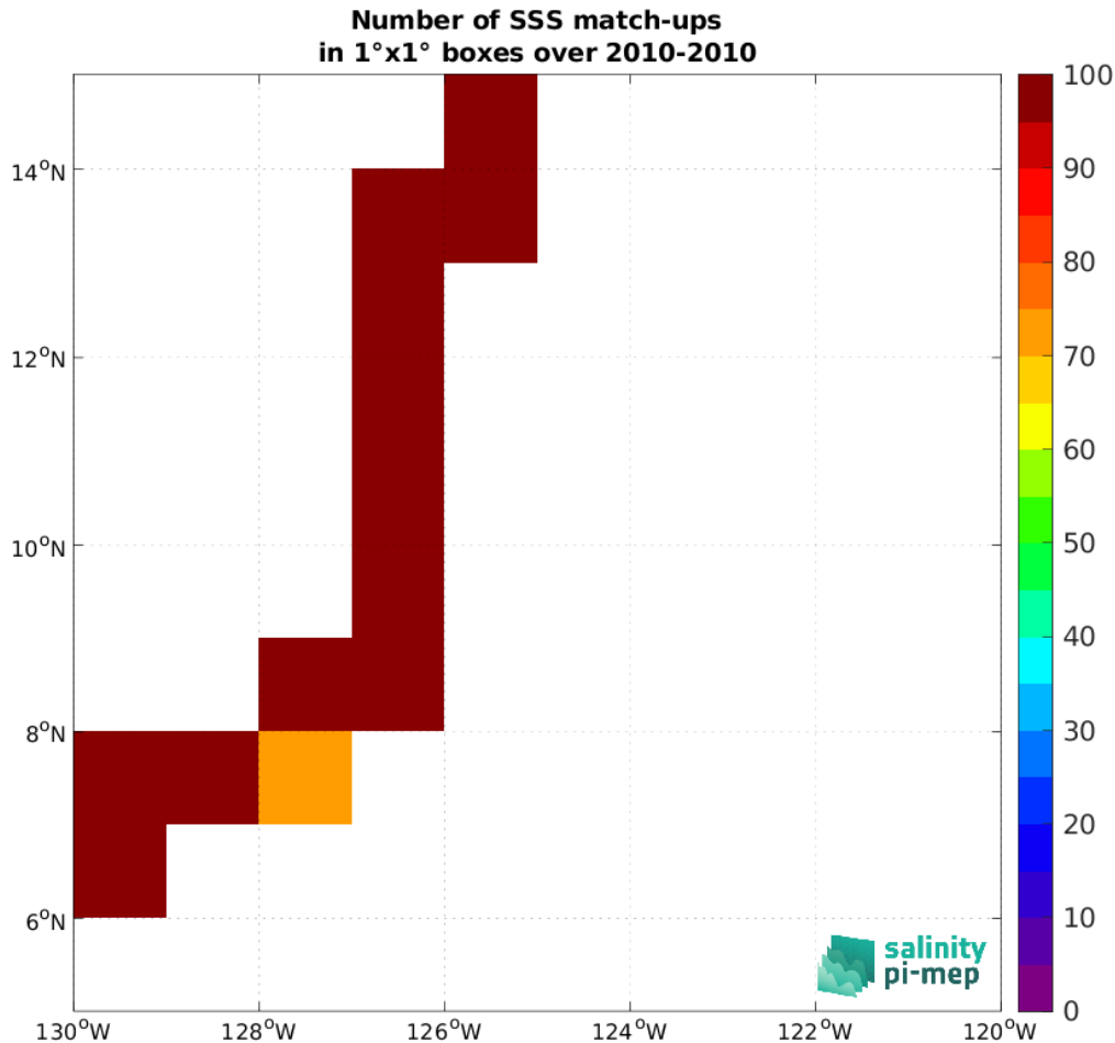
Figure 4: Number of SSS match-ups between TSG (GOSUD-Sailing-ship) SSS and the SMOS SSS L3 v9 - 18 Days (CATDS-CEC-LOCEAN) SSS product for the SPURS 2 Pi-MEP region over 1^\circ \times 1^\circ boxes and for the full satellite product period.
