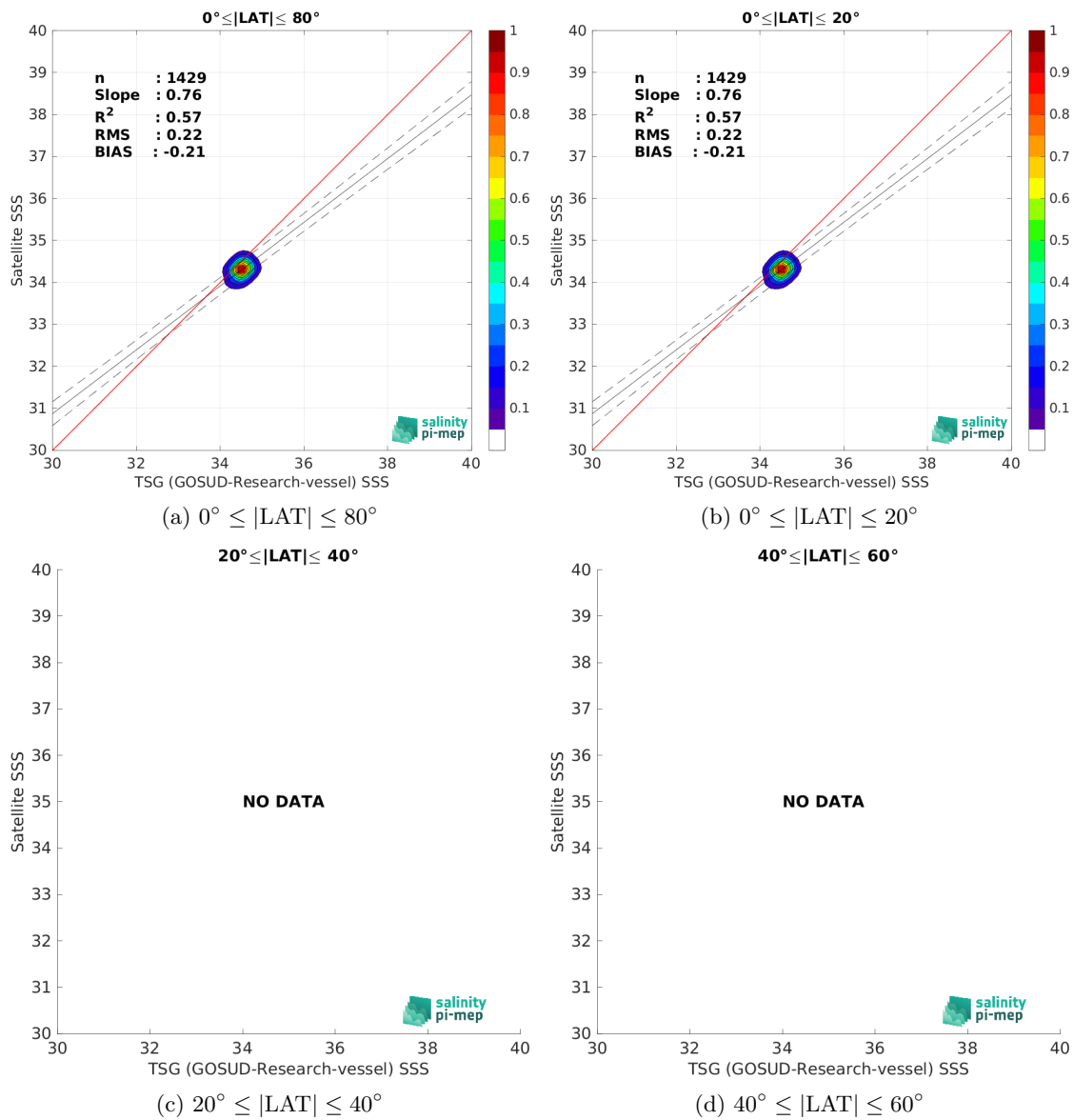
Figure 9: Contour maps of the concentration of SMOS SSS L3 v9 - 18 Days (CATDS-CEC-LOCEAN) SSS (y-axis) versus TSG (GOSUD-Research-vessel) SSS (x-axis) at match-up pairs for different latitude bands. For each plot, the red line shows x=y . The black thin and dashed lines indicate a linear fit through the data cloud and the \pm 95\% confidence levels, respectively. The number match-up pairs n , the slope and R^2 coefficient of the linear fit, the root mean square (RMS) and the mean bias between satellite and in situ data are indicated for each latitude band in each plots.
