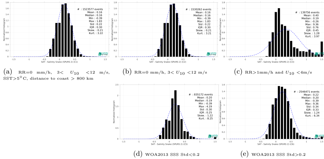
Figure 15: Normalized histogram of \Delta SSS (SMOS SSS L3 v9 - 18 Days (CATDS-CEC-LOCEAN) - Salinity Snake (SPURS 2)) for 5 different subdatasets corresponding to: RR=0 mm/h, 3 < U_{10} < 12 m/s, SST>5°C, distance to coast > 800 km (a), RR=0 mm/h, 3 < U_{10} < 12 m/s (b), RR>1mm/h and U_{10} < 4 m/s (c), WOA2013 SSS Std<0.2 (d), WOA2013 SSS Std>0.2 (e).
