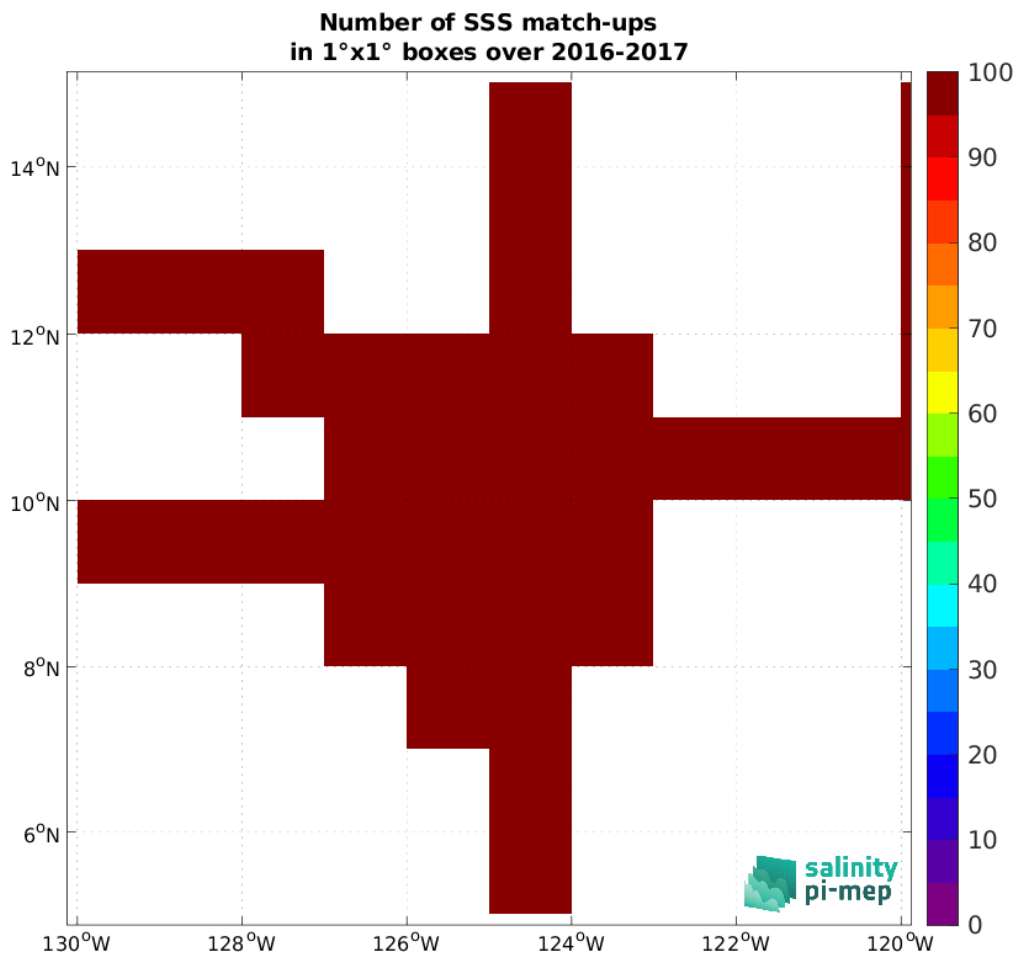
Figure 5: Number of SSS match-ups between Salinity Snake (SPURS 2) SSS and the SMOS SSS L3 v9 - 18 Days (CATDS-CEC-LOCEAN) SSS product for the SPURS 2 Pi-MEP region over 1^\circ \times 1^\circ boxes and for the full satellite product period.
