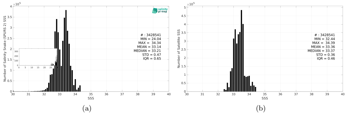
Figure 3: Histograms of SSS from Salinity Snake (SPURS 2) (a) and SMOS SSS L3 v9 - 18 Days (CATDS-CEC-LOCEAN) (b) considering all match-up pairs per bins of 0.1 over the SPURS 2 Pi-MEP region and for the full satellite product period.
