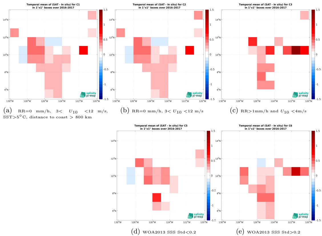
Figure 14: Temporal mean gridded over spatial boxes of size 1^\circ \times 1^\circ of \Delta SSS (SMOS SSS L3 v9 - 18 Days (CATDS-CEC-LOCEAN) - Salinity Snake (SPURS 2)) for 5 different subdatasets corresponding to:RR=0 mm/h, 3 < U_{10} < 12 m/s, SST > 5^\circ\text{C} , distance to coast > 800 km (a), RR=0 mm/h, 3 < U_{10} < 12 m/s (b), RR > 1 mm/h and U_{10} < 4 m/s (c), WOA2013 SSS Std < 0.2 (d), WOA2013 SSS Std > 0.2 (e).
