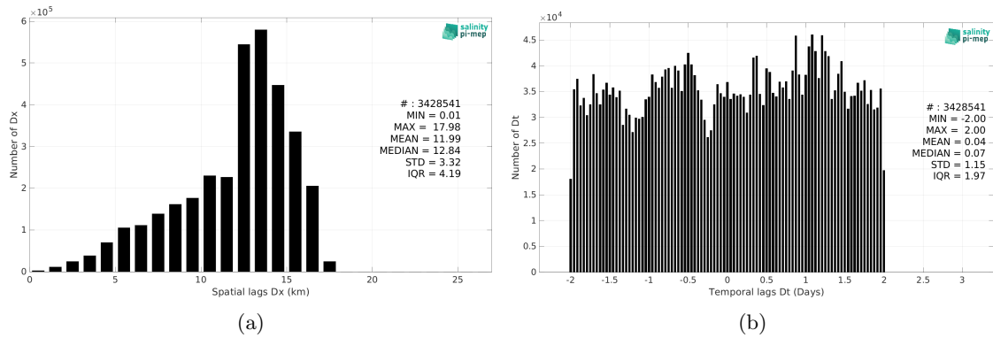
Figure 6: Histograms of the spatial (a) and temporal (b) lags between the location/time of the Salinity Snake (SPURS 2) measurement and the date of the corresponding SMOS SSS L3 v9 - 18 Days (CATDS-CEC-LOCEAN) SSS pixel.
