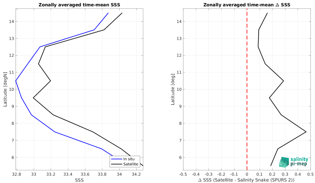
Figure 9: Left panel: Zonal mean SSS from SMOS SSS L3 v9 - 18 Days (CATDS-CEC-LOCEAN) satellite product (black) and from Salinity Snake (SPURS 2) (blue). Right panel: Zonal mean of \Delta SSS (Satellite - Salinity Snake (SPURS 2)) for all the collected Pi-MEP match-up pairs estimated over the full satellite product period.
