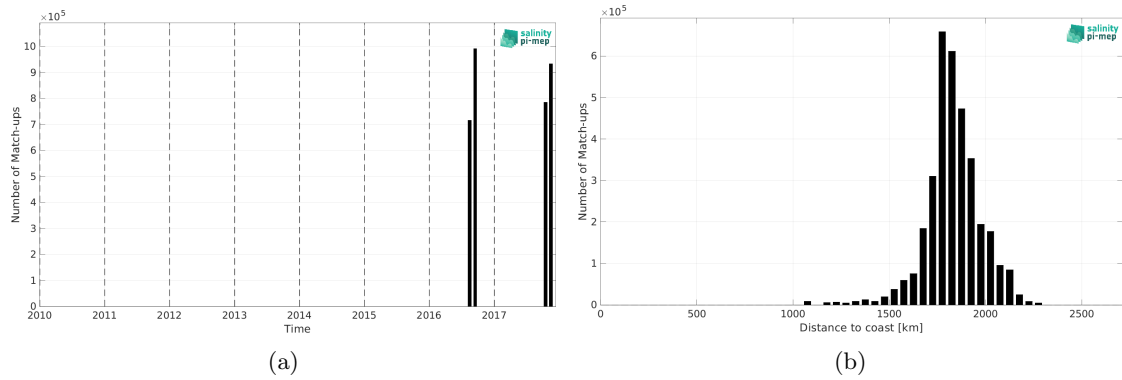
Figure 2: Number of match-ups between Salinity Snake (SPURS 2) and SMOS SSS L3 v9 - 18 Days (CATDS-CEC-LOCEAN) SSS as a function of time (a) and as function of the distance to coast (b) over the SPURS 2 Pi-MEP region and for the full satellite product period.
