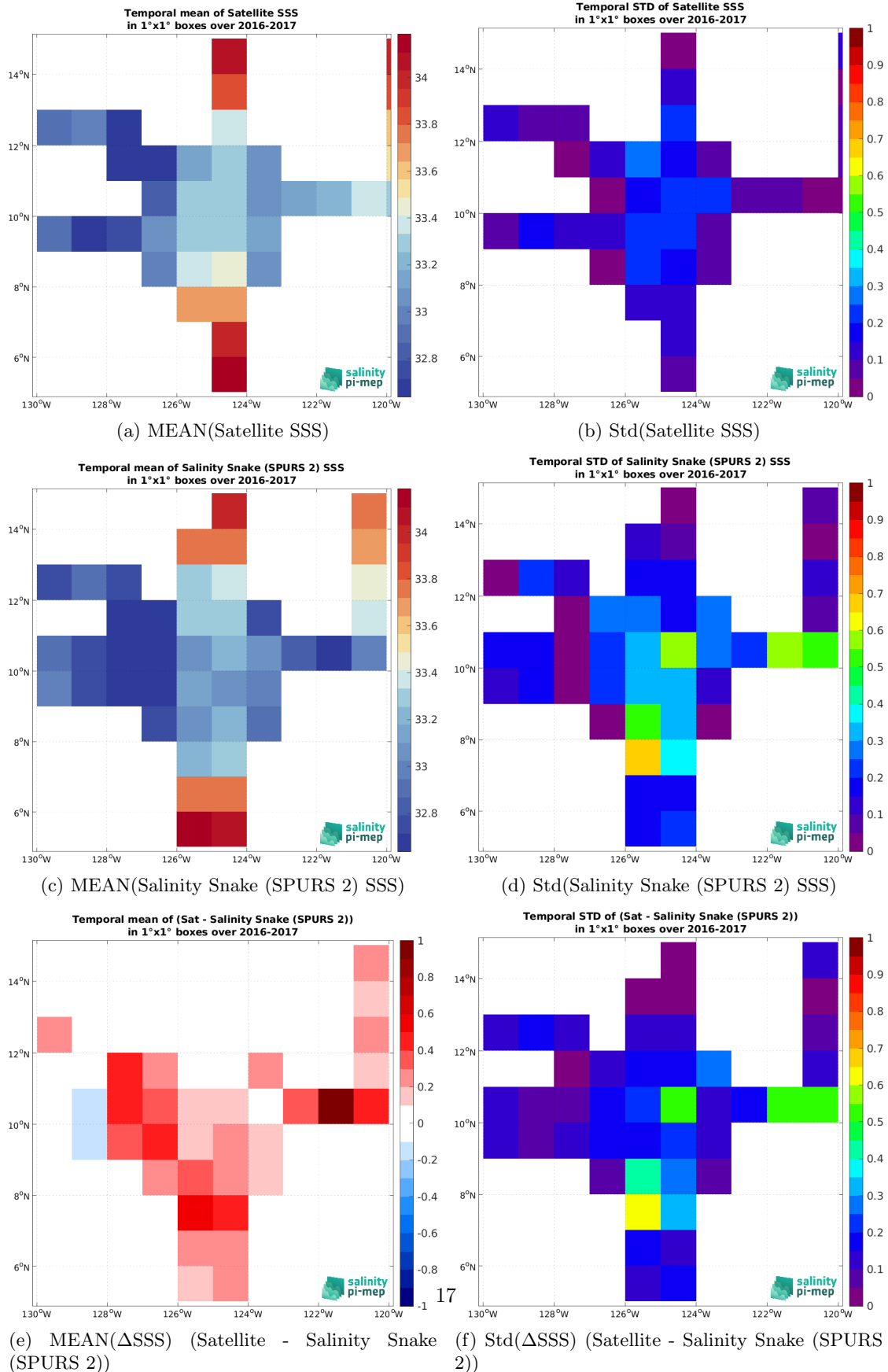
Figure 7: Temporal mean (left) and Std (right) of SSS from SMOS SSS L3 v9 - 18 Days (CATDS-CEC-LOCEAN) (top), Salinity Snake (SPURS 2) (middle), and of \Delta SSS (Satellite - Salinity Snake (SPURS 2)). Only match-up pairs are used to generate these maps.
