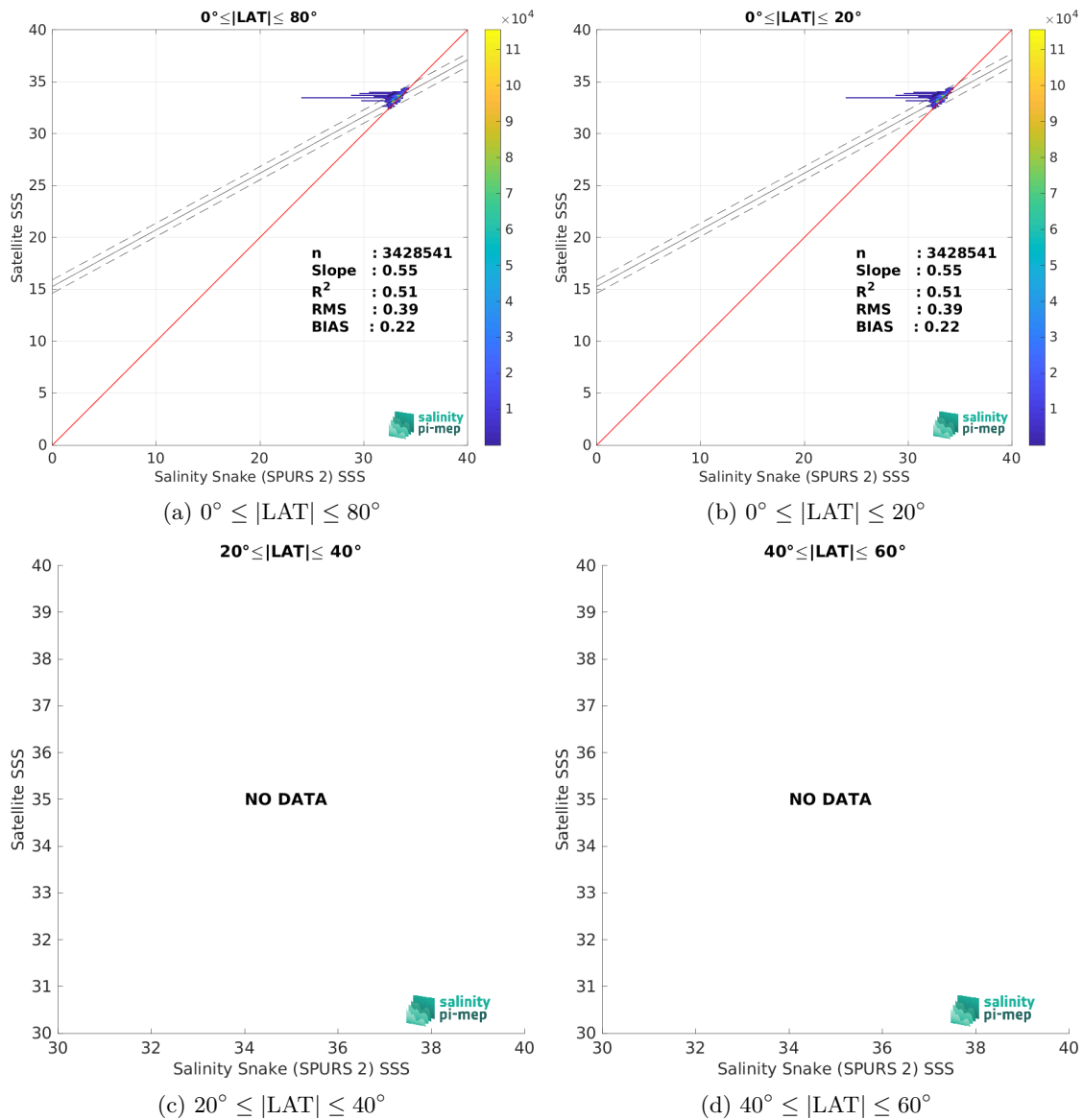
Figure 10: Contour maps of the concentration of SMOS SSS L3 v9 - 18 Days (CATDS-CEC-LOCEAN) SSS (y-axis) versus Salinity Snake (SPURS 2) SSS (x-axis) at match-up pairs for different latitude bands. For each plot, the red line shows x=y . The black thin and dashed lines indicate a linear fit through the data cloud and the \pm 95\% confidence levels, respectively. The number match-up pairs n , the slope and R^2 coefficient of the linear fit, the root mean square (RMS) and the mean bias between satellite and in situ data are indicated for each latitude band in each plots.
