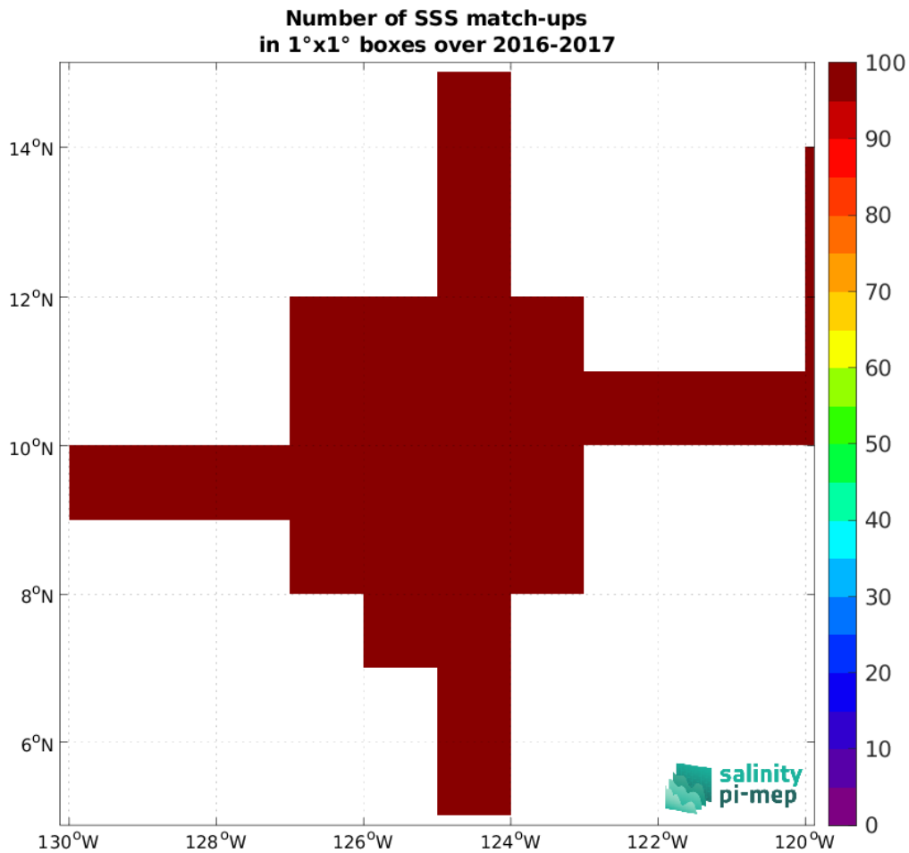
Figure 4: Number of SSS match-ups between Salinity Snake (SPURS 2) SSS and the SMOS SSS L3 v9 - 18 Days (CATDS-CEC-LOCEAN) SSS product for the SPURS 2 Pi-MEP region over 1^\circ \times 1^\circ boxes and for the full satellite product period.
