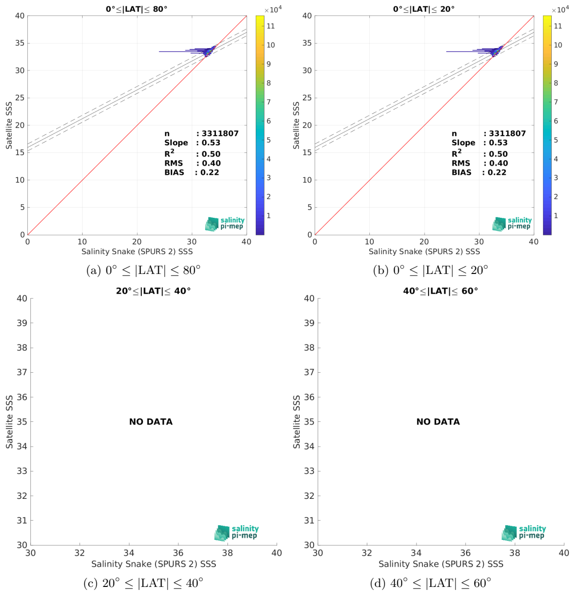
Figure 9: Contour maps of the concentration of SMOS SSS L3 v9 - 18 Days (CATDS-CEC-LOCEAN) SSS (y-axis) versus Salinity Snake (SPURS 2) SSS (x-axis) at match-up pairs for different latitude bands. For each plot, the red line shows x=y . The black thin and dashed lines indicate a linear fit through the data cloud and the \pm 95\% confidence levels, respectively. The number match-up pairs n , the slope and R^2 coefficient of the linear fit, the root mean square (RMS) and the mean bias between satellite and in situ data are indicated for each latitude band in each plots.
