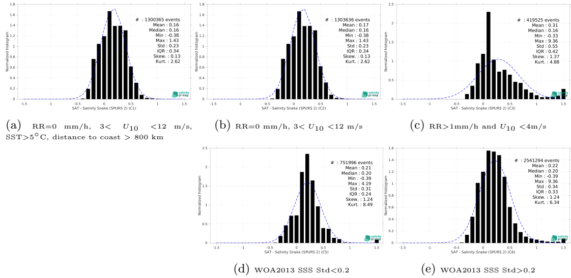
Figure 13: Normalized histogram of \Delta SSS (SMOS SSS L3 v9 - 18 Days (CATDS-CEC-LOCEAN) - Salinity Snake (SPURS 2)) for 5 different subdatasets corresponding to: RR=0 mm/h, 3 < U_{10} < 12 m/s, SST>5°C, distance to coast > 800 km (a), RR=0 mm/h, 3 < U_{10} < 12 m/s (b), RR>1mm/h and U_{10} < 4 m/s (c), WOA2013 SSS Std<0.2 (d), WOA2013 SSS Std>0.2 (e).
