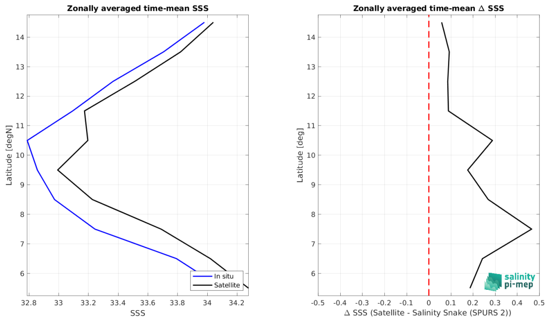
Figure 8: Left panel: Zonal mean SSS from SMOS SSS L3 v9 - 18 Days (CATDS-CEC-LOCEAN) satellite product (black) and from Salinity Snake (SPURS 2) (blue). Right panel: Zonal mean of \Delta SSS (Satellite - Salinity Snake (SPURS 2)) for all the collected Pi-MEP match-up pairs estimated over the full satellite product period.
