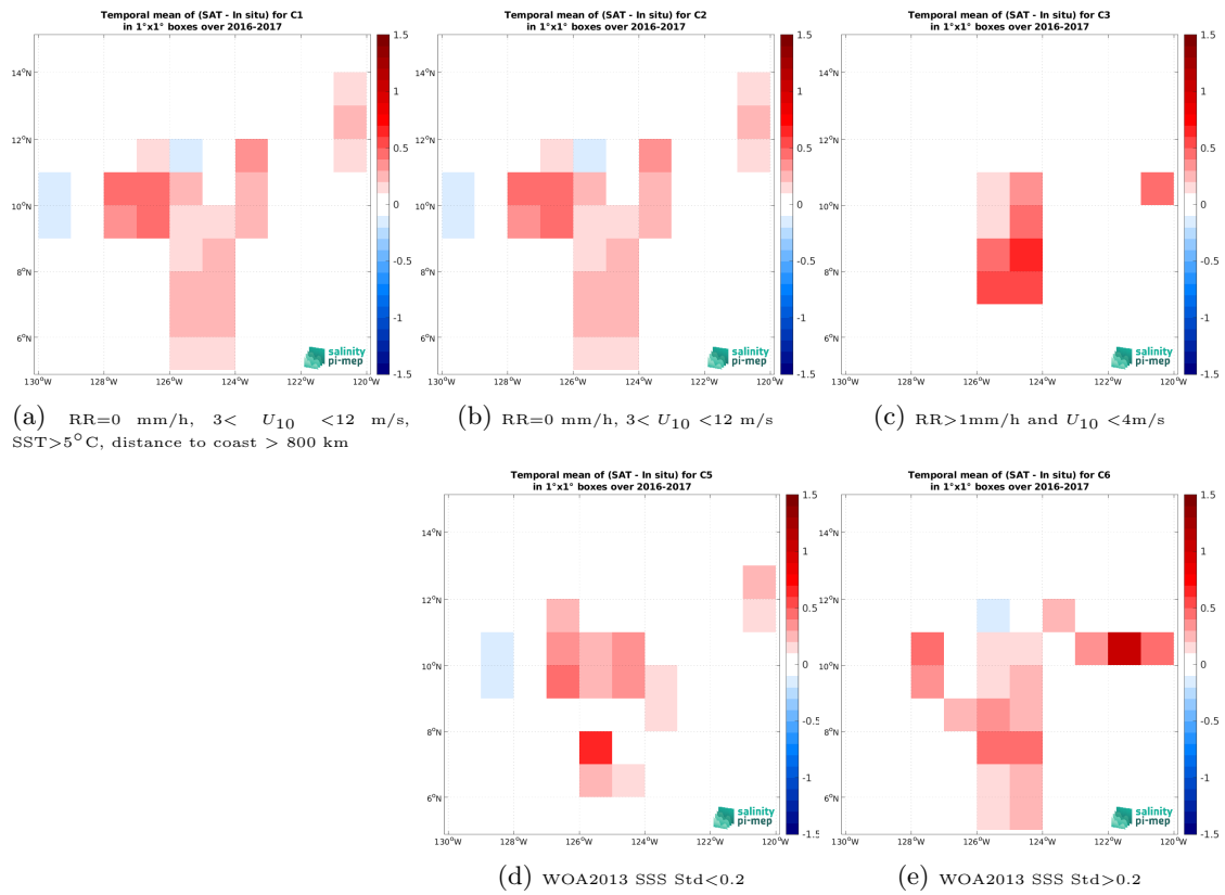
Figure 12: Temporal mean gridded over spatial boxes of size 1^\circ \times 1^\circ of \Delta SSS (SMOS SSS L3 v9 - 18 Days (CATDS-CEC-LOCEAN) - Salinity Snake (SPURS 2)) for 5 different subdatasets corresponding to: RR=0 mm/h, 3 < U_{10} < 12 m/s, SST>5°C, distance to coast > 800 km (a), RR=0 mm/h, 3 < U_{10} < 12 m/s (b), RR>1mm/h and U_{10} < 4 m/s (c), WOA2013 SSS Std<0.2 (d), WOA2013 SSS Std>0.2 (e).
