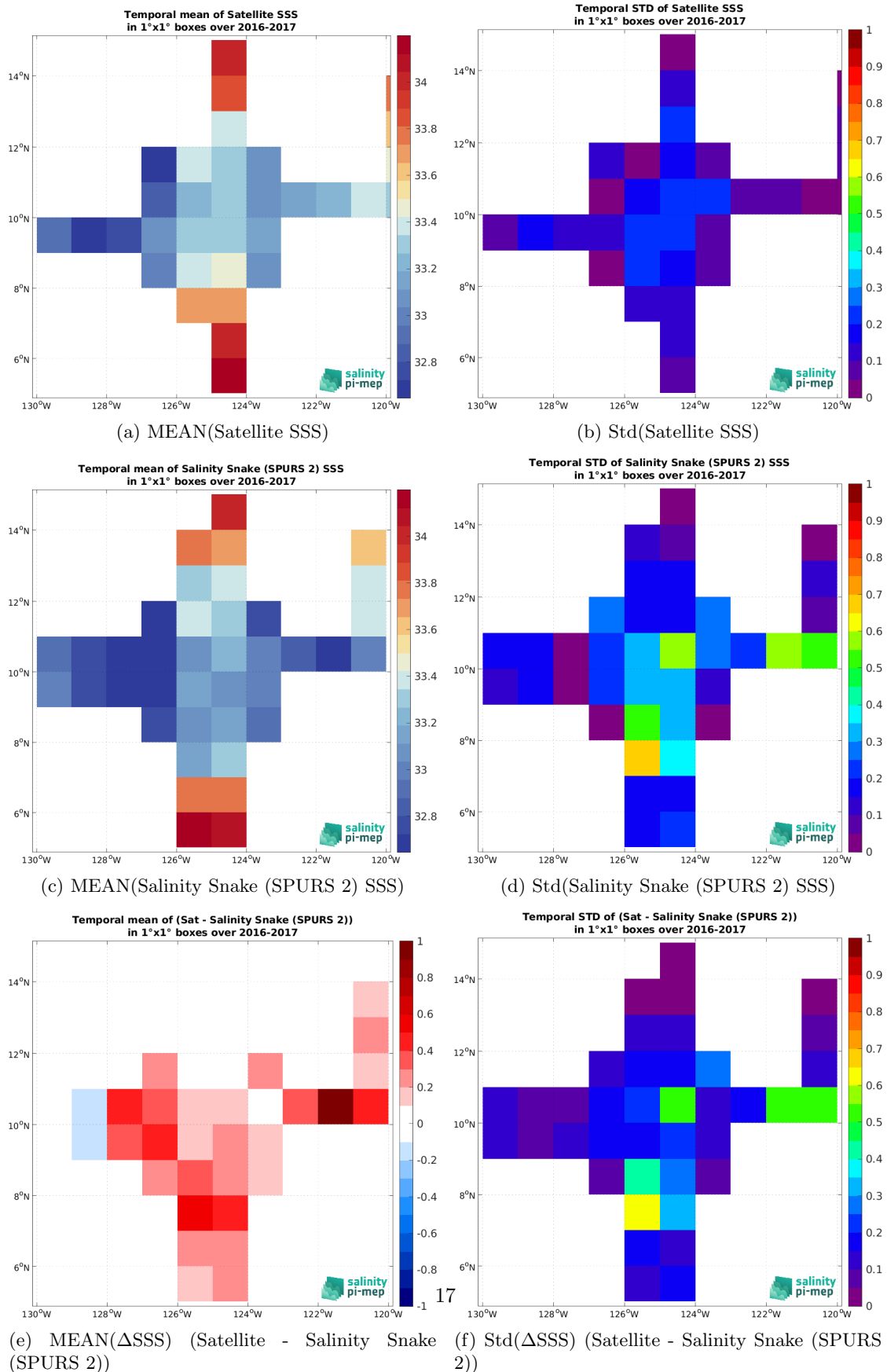
Figure 6: Temporal mean (left) and Std (right) of SSS from SMOS SSS L3 v9 - 18 Days (CATDS-CEC-LOCEAN) (top), Salinity Snake (SPURS 2) (middle), and of \Delta SSS (Satellite - Salinity Snake (SPURS 2)). Only match-up pairs are used to generate these maps.
