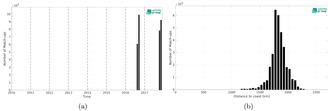
Figure 1: Number of match-ups between Salinity Snake (SPURS 2) and SMOS SSS L3 v9 - 18 Days (CATDS-CEC-LOCEAN) SSS as a function of time (a) and as function of the distance to coast (b) over the SPURS 2 Pi-MEP region and for the full satellite product period.
