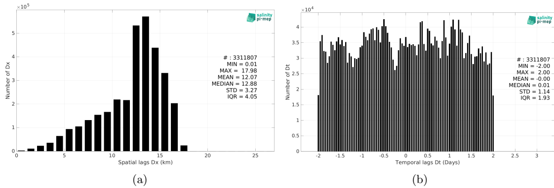
Figure 5: Histograms of the spatial (a) and temporal (b) lags between the location/time of the Salinity Snake (SPURS 2) measurement and the date of the corresponding SMOS SSS L3 v9 - 18 Days (CATDS-CEC-LOCEAN) SSS pixel.
