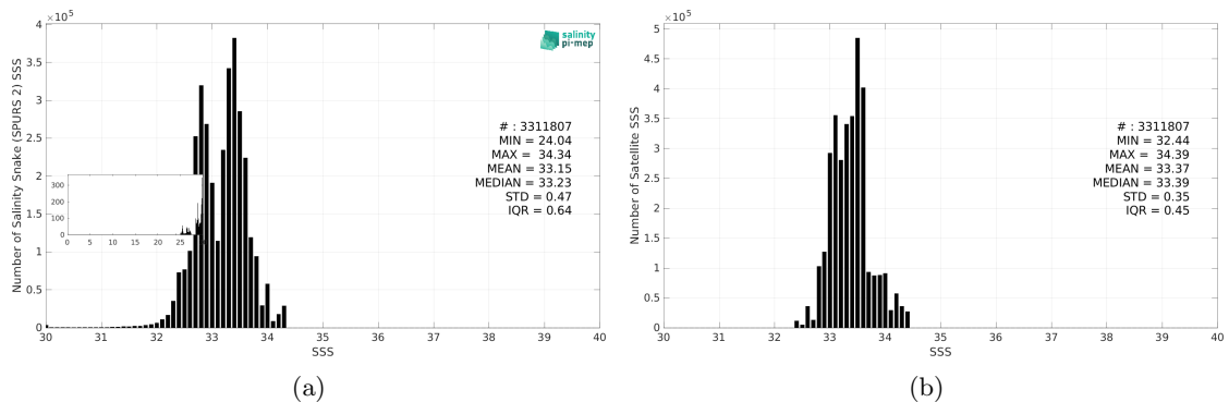
Figure 2: Histograms of SSS from Salinity Snake (SPURS 2) (a) and SMOS SSS L3 v9 - 18 Days (CATDS-CEC-LOCEAN) (b) considering all match-up pairs per bins of 0.1 over the SPURS 2 Pi-MEP region and for the full satellite product period.
