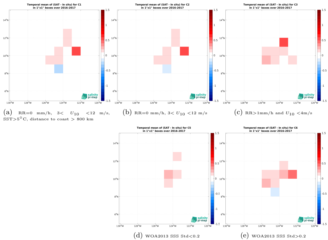
Figure 14: Temporal mean gridded over spatial boxes of size 1^\circ \times 1^\circ of \Delta SSS (SMOS SSS L3 v9 - 18 Days (CATDS-CEC-LOCEAN) - Seaglider (SPURS 2)) for 5 different subdatasets corresponding to:RR=0 mm/h, 3 < U_{10} < 12 m/s, SST >5^\circ C, distance to coast > 800 km (a), RR=0 mm/h, 3 < U_{10} < 12 m/s (b), RR >1 mm/h and U_{10} < 4 m/s (c), WOA2013 SSS Std <0.2 (d), WOA2013 SSS Std >0.2 (e).
