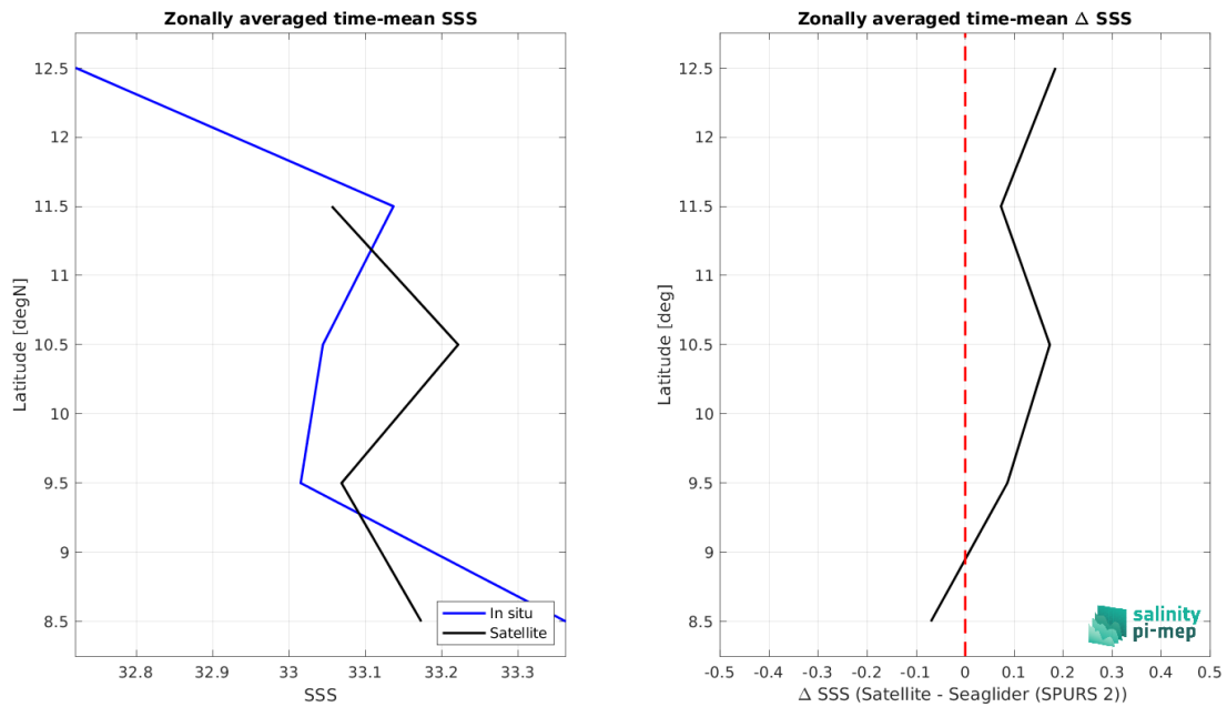
Figure 9: Left panel: Zonal mean SSS from SMOS SSS L3 v9 - 18 Days (CATDS-CEC-LOCEAN) satellite product (black) and from Seaglider (SPURS 2) (blue). Right panel: Zonal mean of \Delta SSS (Satellite - Seaglider (SPURS 2)) for all the collected Pi-MEP match-up pairs estimated over the full satellite product period.
