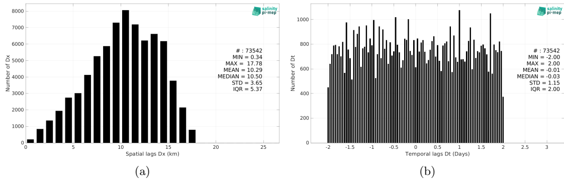
Figure 6: Histograms of the spatial (a) and temporal (b) lags between the location/time of the Seaglider (SPURS 2) measurement and the date of the corresponding SMOS SSS L3 v9 - 18 Days (CATDS-CEC-LOCEAN) SSS pixel.
