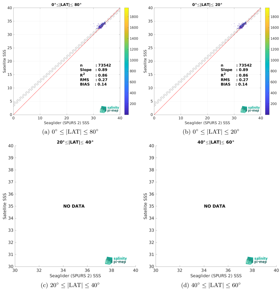
Figure 10: Contour maps of the concentration of SMOS SSS L3 v9 - 18 Days (CATDS-CEC-LOCEAN) SSS (y-axis) versus Seaglider (SPURS 2) SSS (x-axis) at match-up pairs for different latitude bands. For each plot, the red line shows x=y . The black thin and dashed lines indicate a linear fit through the data cloud and the \pm 95\% confidence levels, respectively. The number match-up pairs n , the slope and R^2 coefficient of the linear fit, the root mean square (RMS) and the mean bias between satellite and in situ data are indicated for each latitude band in each plots.
