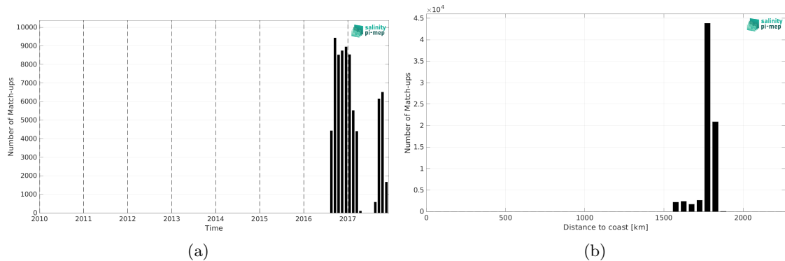
Figure 2: Number of match-ups between Seaglider (SPURS 2) and SMOS SSS L3 v9 - 18 Days (CATDS-CEC-LOCEAN) SSS as a function of time (a) and as function of the distance to coast (b) over the SPURS 2 Pi-MEP region and for the full satellite product period.
