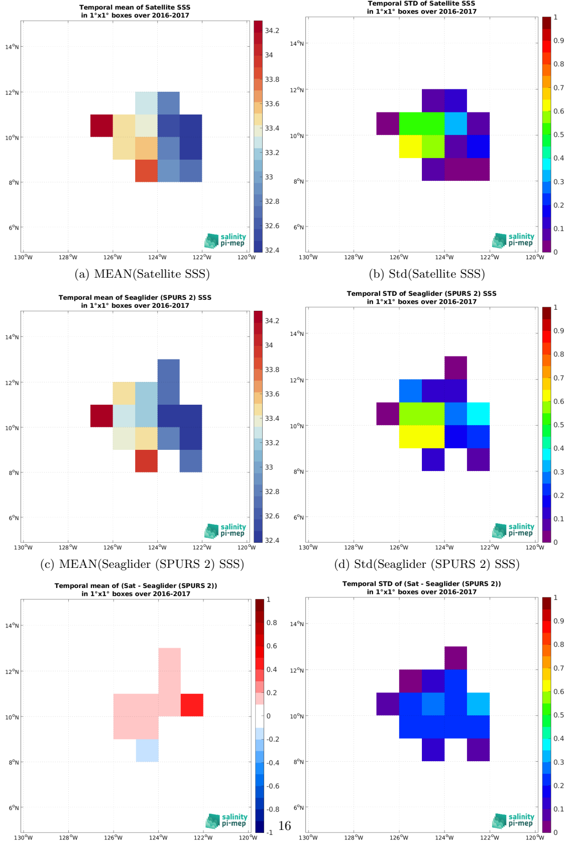
Figure 7: Temporal mean (left) and Std (right) of SSS from SMOS SSS L3 v9 - 18 Days (CATDS-CEC-LOCEAN) (top), Seaglider (SPURS 2) (middle), and of \Delta SSS (Satellite - Seaglider (SPURS 2)). Only match-up pairs are used to generate these maps.
