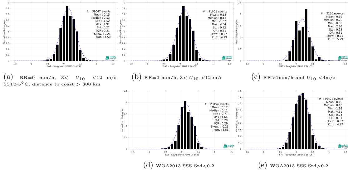
Figure 15: Normalized histogram of \Delta SSS (SMOS SSS L3 v9 - 18 Days (CATDS-CEC-LOCEAN) - Seaglider (SPURS 2)) for 5 different subdatasets corresponding to: RR=0 mm/h, 3 < U_{10} < 12 m/s, SST>5°C, distance to coast > 800 km (a), RR=0 mm/h, 3 < U_{10} < 12 m/s (b), RR>1mm/h and U_{10} < 4 m/s (c), WOA2013 SSS Std<0.2 (d), WOA2013 SSS Std>0.2 (e).
