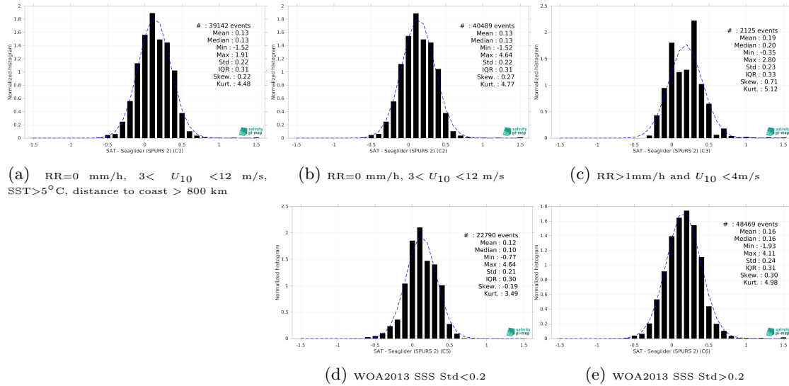
Figure 15: Normalized histogram of \Delta SSS (SMOS SSS L3 v9 - 18 Days (CATDS-CEC-LOCEAN) - Seaglider (SPURS 2)) for 5 different subdatasets corresponding to: RR=0 mm/h, 3 < U_{10} < 12 m/s, SST > 5°C, distance to coast > 800 km (a), RR=0 mm/h, 3 < U_{10} < 12 m/s (b), RR > 1mm/h and U_{10} < 4 m/s (c), WOA2013 SSS Std < 0.2 (d), WOA2013 SSS Std > 0.2 (e).
