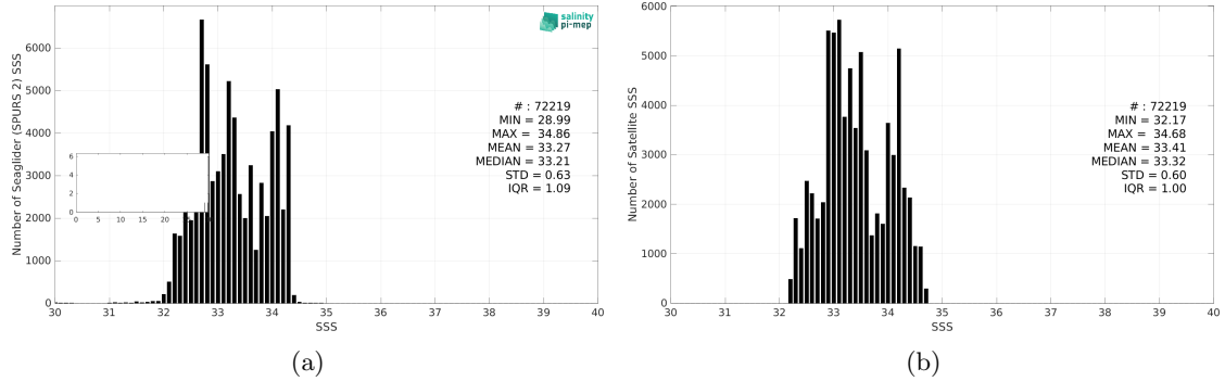
Figure 3: Histograms of SSS from Seagliders (SPURS 2) (a) and SMOS SSS L3 v9 - 18 Days (CATDS-CEC-LOCEAN) (b) considering all match-up pairs per bins of 0.1 over the SPURS 2 Pi-MEP region and for the full satellite product period.
