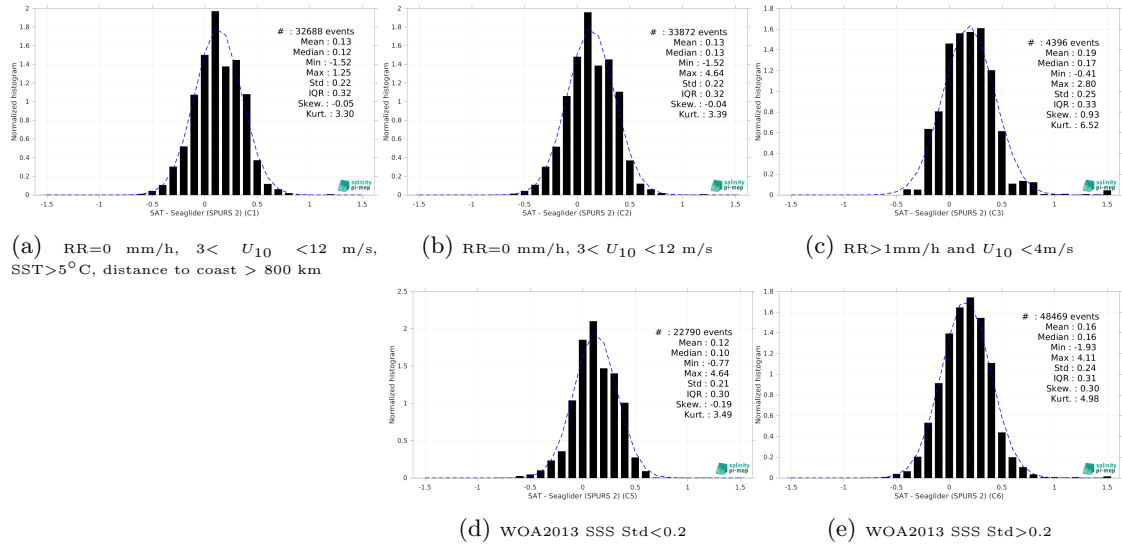
Figure 13: Normalized histogram of \Delta SSS (SMOS SSS L3 v9 - 18 Days (CATDS-CEC-LOCEAN) - Seaglider (SPURS 2)) for 5 different subdatasets corresponding to: RR=0 mm/h, 3 < U_{10} < 12 m/s, SST > 5°C, distance to coast > 800 km (a), RR=0 mm/h, 3 < U_{10} < 12 m/s (b), RR > 1mm/h and U_{10} < 4 m/s (c), WOA2013 SSS Std < 0.2 (d), WOA2013 SSS Std > 0.2 (e).
