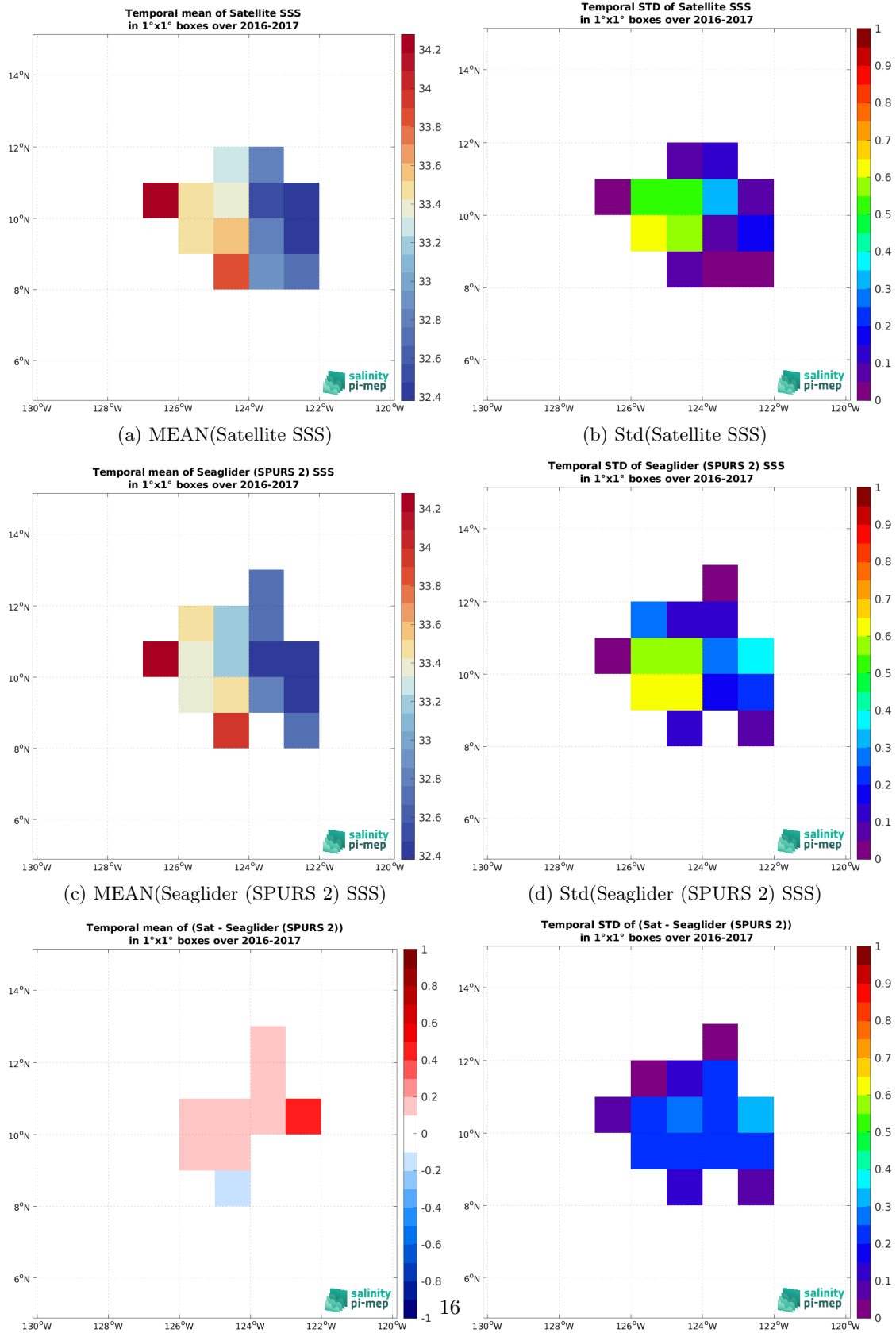
Figure 6: Temporal mean (left) and Std (right) of SSS from SMOS SSS L3 v9 - 18 Days (CATDS-CEC-LOCEAN) (top), Seaglider (SPURS 2) (middle), and of \Delta SSS (Satellite - Seaglider (SPURS 2)). Only match-up pairs are used to generate these maps.
