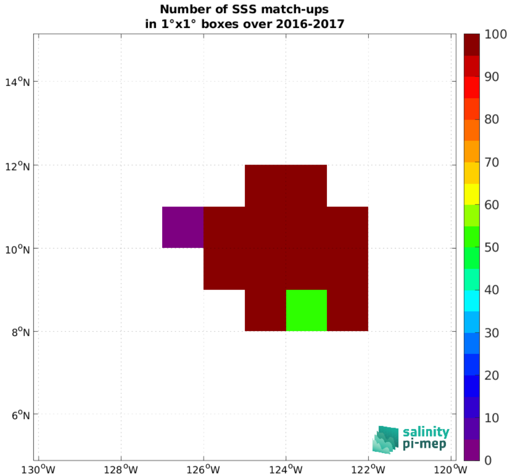
Figure 4: Number of SSS match-ups between Seaglider (SPURS 2) SSS and the SMOS SSS L3 v9 - 18 Days (CATDS-CEC-LOCEAN) SSS product for the SPURS 2 Pi-MEP region over 1^\circ \times 1^\circ boxes and for the full satellite product period.
