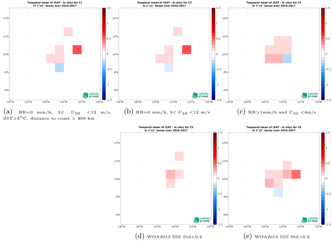
Figure 12: Temporal mean gridded over spatial boxes of size 1^{\circ}\times 1^{\circ} of \Delta\text{SSS} (SMOS SSS L3 v9 - 18 Days (CATDS-CEC-LOCEAN) - Seaglider (SPURS 2)) for 5 different subdatasets corresponding to:RR=0 mm/h, 3 < U_{10} < 12 m/s, SST >5^{\circ}\text{C} , distance to coast > 800 km (a), RR=0 mm/h, 3 < U_{10} < 12 m/s (b), RR >1 mm/h and U_{10} < 4 m/s (c), WOA2013 SSS Std <0.2 (d), WOA2013 SSS Std >0.2 (e).
