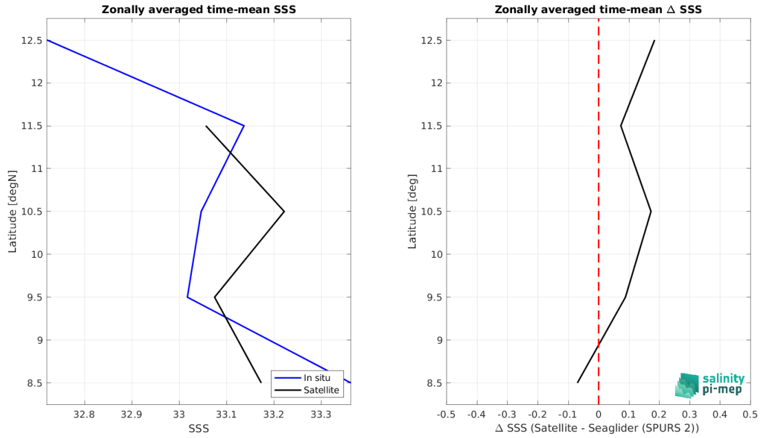
Figure 8: Left panel: Zonal mean SSS from SMOS SSS L3 v9 - 18 Days (CATDS-CEC-LOCEAN) satellite product (black) and from Seaglider (SPURS 2) (blue). Right panel: Zonal mean of \Delta SSS (Satellite - Seaglider (SPURS 2)) for all the collected Pi-MEP match-up pairs estimated over the full satellite product period.
