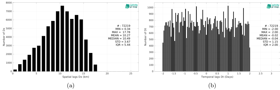
Figure 5: Histograms of the spatial (a) and temporal (b) lags between the location/time of the Seaglider (SPURS 2) measurement and the date of the corresponding SMOS SSS L3 v9 - 18 Days (CATDS-CEC-LOCEAN) SSS pixel.
