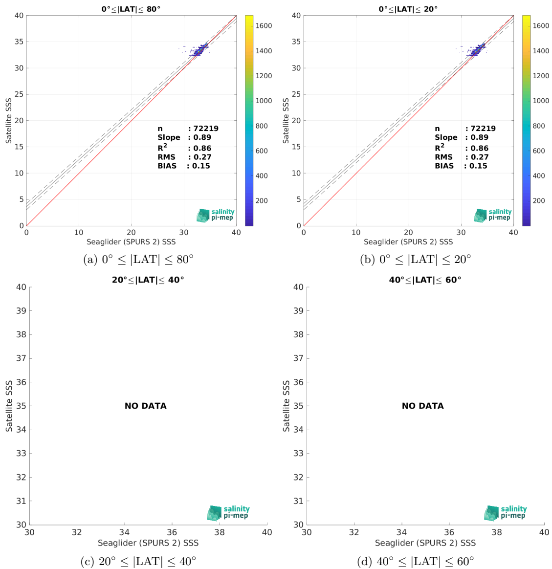
Figure 9: Contour maps of the concentration of SMOS SSS L3 v9 - 18 Days (CATDS-CEC-LOCEAN) SSS (y-axis) versus Seaglider (SPURS 2) SSS (x-axis) at match-up pairs for different latitude bands. For each plot, the red line shows x=y . The black thin and dashed lines indicate a linear fit through the data cloud and the \pm 95\% confidence levels, respectively. The number match-up pairs n , the slope and R^2 coefficient of the linear fit, the root mean square (RMS) and the mean bias between satellite and in situ data are indicated for each latitude band in each plots.
