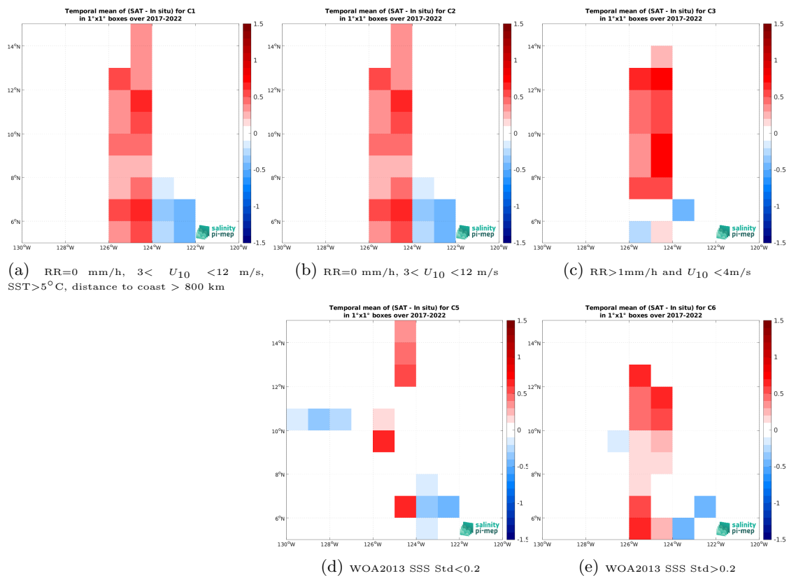
Figure 14: Temporal mean gridded over spatial boxes of size 1^\circ \times 1^\circ of \Delta\text{SSS} (SMOS SSS L3 v9 - 18 Days (CATDS-CEC-LOCEAN) - Sairdrone) for 5 different subdatasets corresponding to:RR=0 mm/h, 3 < U_{10} < 12 m/s, SST>5°C, distance to coast > 800 km (a), RR=0 mm/h, 3 < U_{10} < 12 m/s (b), RR>1mm/h and U_{10} < 4 m/s (c), WOA2013 SSS Std<0.2 (d), WOA2013 SSS Std>0.2 (e).
