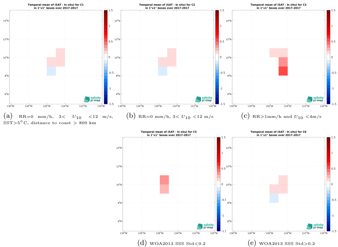
Figure 14: Temporal mean gridded over spatial boxes of size 1^\circ \times 1^\circ of \Delta SSS (SMOS SSS L3 v9 - 18 Days (CATDS-CEC-LOCEAN) - Saildrone (SPURS 2)) for 5 different subdatasets corresponding to:RR=0 mm/h, 3 < U_{10} < 12 m/s, SST >5^\circ C, distance to coast > 800 km (a), RR=0 mm/h, 3 < U_{10} < 12 m/s (b), RR >1 mm/h and U_{10} < 4 m/s (c), WOA2013 SSS Std <0.2 (d), WOA2013 SSS Std >0.2 (e).
