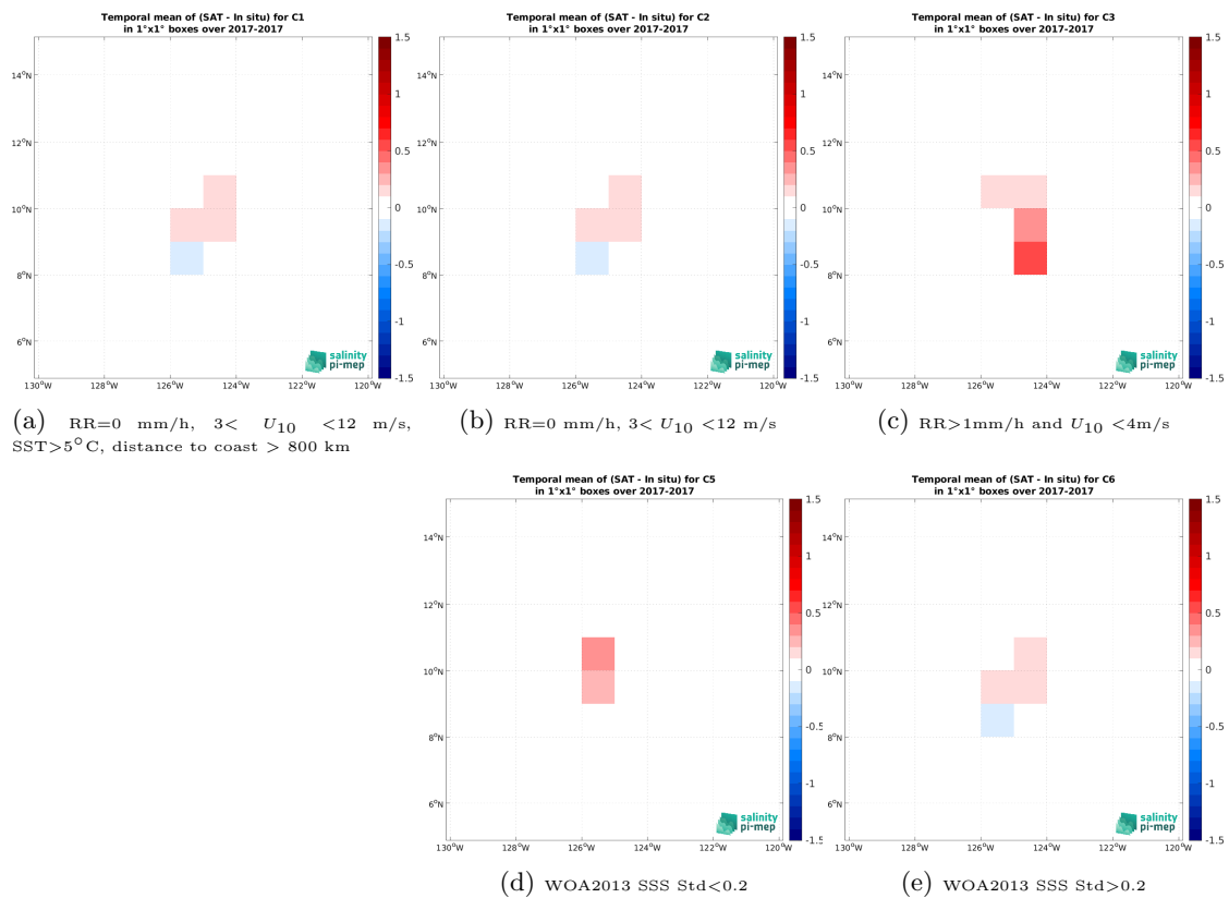
Figure 14: Temporal mean gridded over spatial boxes of size 1^\circ \times 1^\circ of \Delta\text{SSS} (SMOS SSS L3 v9 - 18 Days (CATDS-CEC-LOCEAN) - Sailability (SPURS 2)) for 5 different subdatasets corresponding to: RR=0 mm/h, 3 < U_{10} < 12 m/s, SST > 5°C, distance to coast > 800 km (a), RR=0 mm/h, 3 < U_{10} < 12 m/s (b), RR > 1mm/h and U_{10} < 4 m/s (c), WOA2013 SSS Std < 0.2 (d), WOA2013 SSS Std > 0.2 (e).
