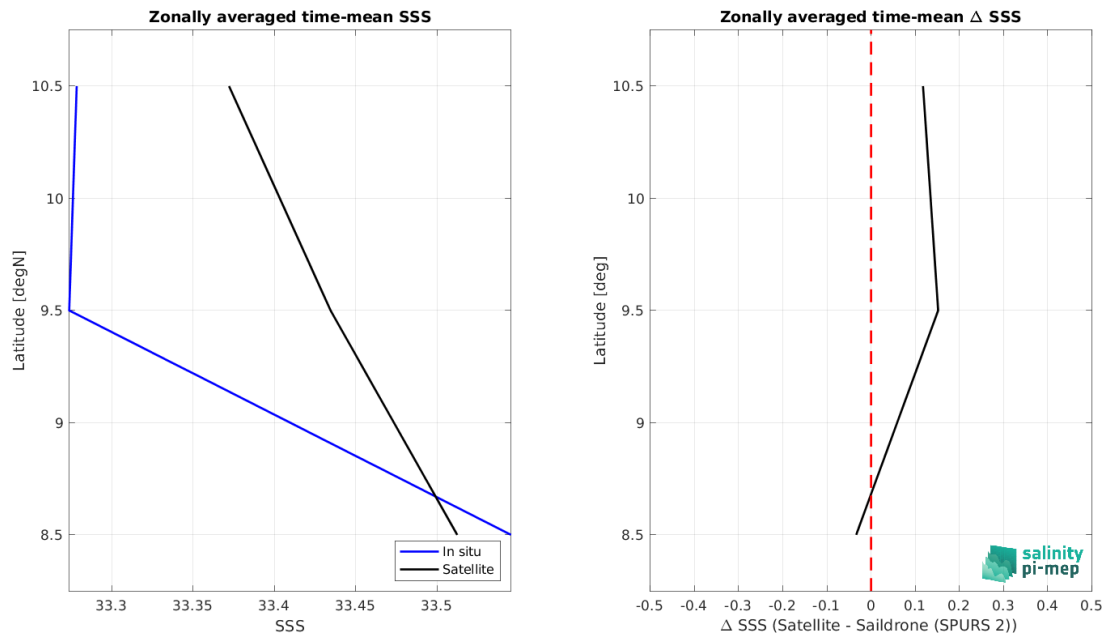
Figure 9: Left panel: Zonal mean SSS from SMOS SSS L3 v9 - 18 Days (CATDS-CEC-LOCEAN) satellite product (black) and from Sairdron (SPURS 2) (blue). Right panel: Zonal mean of \Delta SSS (Satellite - Sairdron (SPURS 2)) for all the collected Pi-MEP match-up pairs estimated over the full satellite product period.
