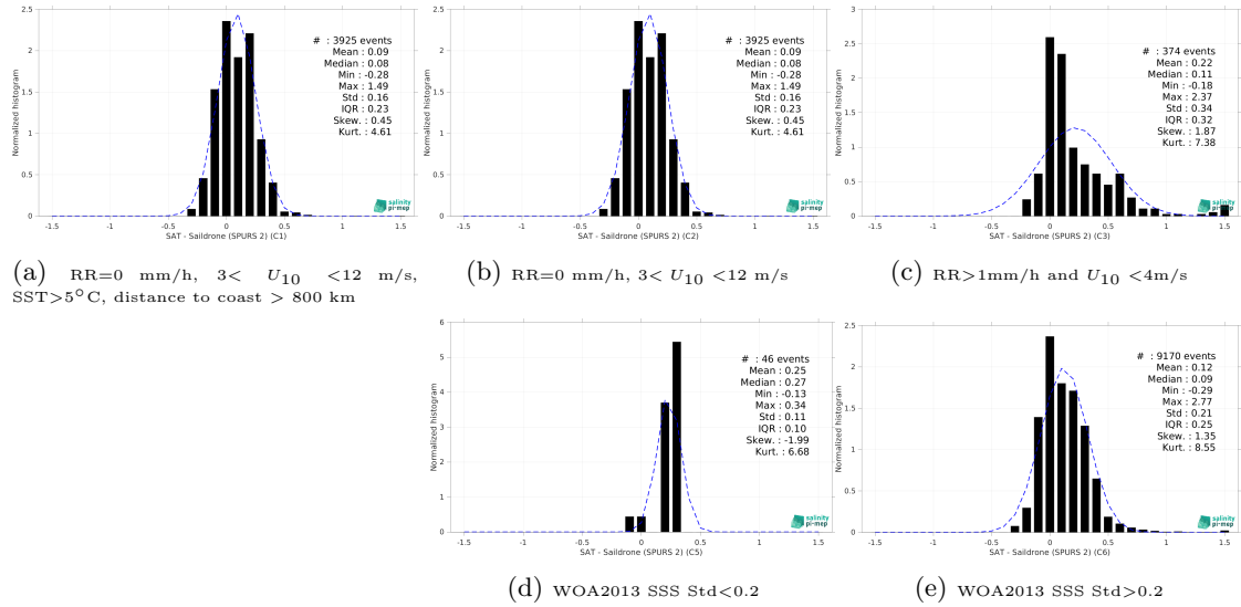
Figure 15: Normalized histogram of \Delta SSS (SMOS SSS L3 v9 - 18 Days (CATDS-CEC-LOCEAN) - Saildrone (SPURS 2)) for 5 different subdatasets corresponding to: RR=0 mm/h, 3 < U_{10} < 12 m/s, SST > 5°C, distance to coast > 800 km (a), RR=0 mm/h, 3 < U_{10} < 12 m/s (b), RR > 1mm/h and U_{10} < 4 m/s (c), WOA2013 SSS Std < 0.2 (d), WOA2013 SSS Std > 0.2 (e).
