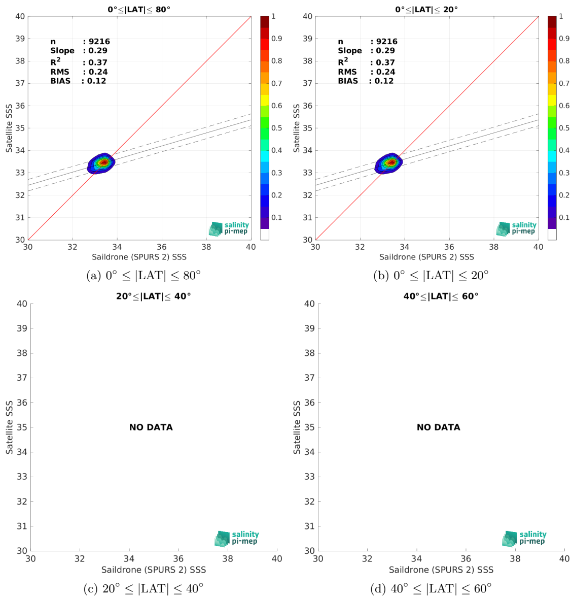
Figure 10: Contour maps of the concentration of SMOS SSS L3 v9 - 18 Days (CATDS-CEC-LOCEAN) SSS (y-axis) versus Saildrone (SPURS 2) SSS (x-axis) at match-up pairs for different latitude bands. For each plot, the red line shows x=y . The black thin and dashed lines indicate a linear fit through the data cloud and the \pm 95\% confidence levels, respectively. The number match-up pairs n , the slope and R^2 coefficient of the linear fit, the root mean square (RMS) and the mean bias between satellite and in situ data are indicated for each latitude band in each plots.
