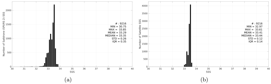
Figure 3: Histograms of SSS from Saildrone (SPURS 2) (a) and SMOS SSS L3 v9 - 18 Days (CATDS-CEC-LOCEAN) (b) considering all match-up pairs per bins of 0.1 over the SPURS 2 Pi-MEP region and for the full satellite product period.
