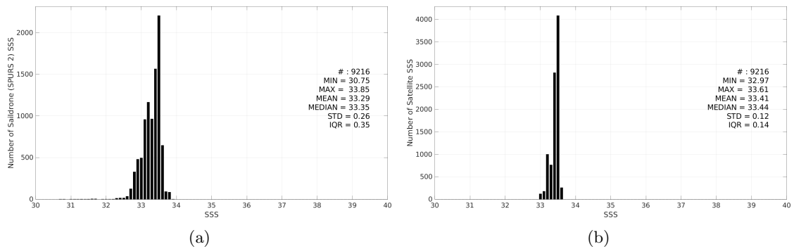
Figure 2: Histograms of SSS from Saildrone (SPURS 2) (a) and SMOS SSS L3 v9 - 18 Days (CATDS-CEC-LOCEAN) (b) considering all match-up pairs per bins of 0.1 over the SPURS 2 Pi-MEP region and for the full satellite product period.
