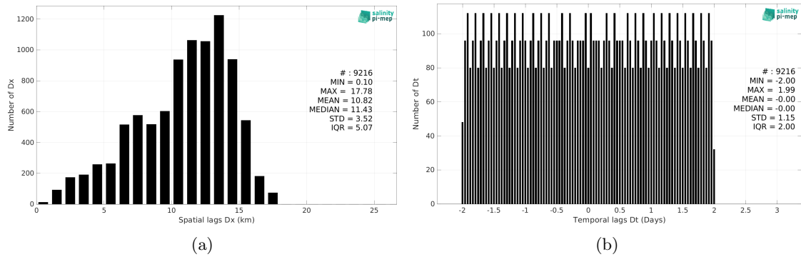
Figure 5: Histograms of the spatial (a) and temporal (b) lags between the location/time of the Saildrone (SPURS 2) measurement and the date of the corresponding SMOS SSS L3 v9 - 18 Days (CATDS-CEC-LOCEAN) SSS pixel.
