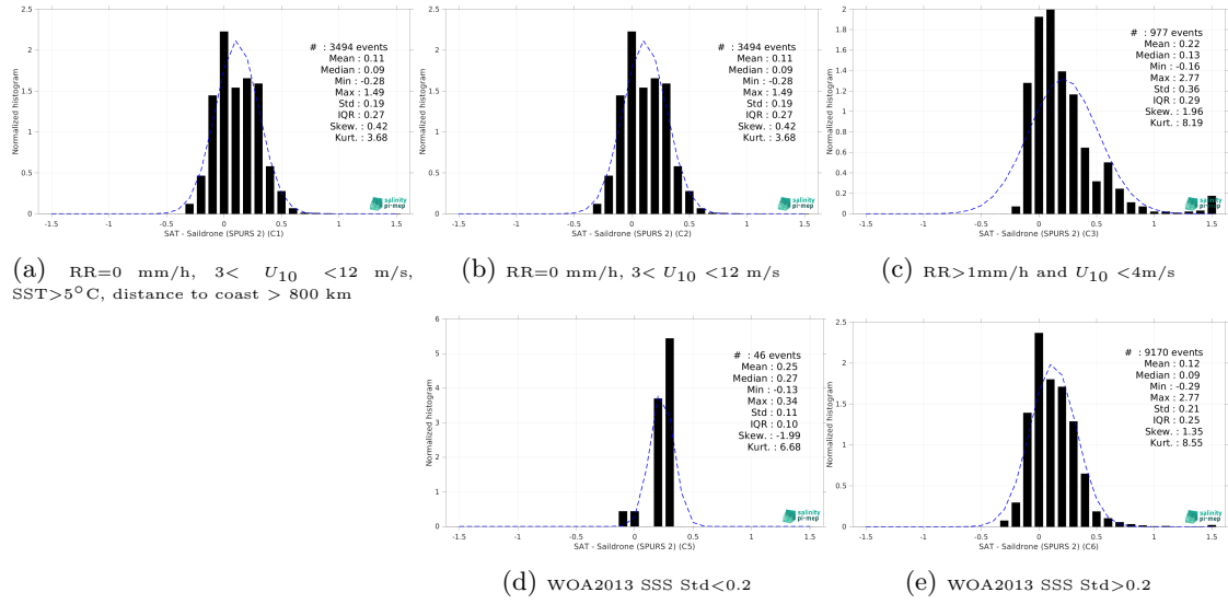
Figure 13: Normalized histogram of \Delta SSS (SMOS SSS L3 v9 - 18 Days (CATDS-CEC-LOCEAN) - Saildrone (SPURS 2)) for 5 different subdatasets corresponding to: RR=0 mm/h, 3 < U_{10} < 12 m/s, SST>5°C, distance to coast > 800 km (a), RR=0 mm/h, 3 < U_{10} < 12 m/s (b), RR>1mm/h and U_{10} < 4 m/s (c), WOA2013 SSS Std<0.2 (d), WOA2013 SSS Std>0.2 (e).
