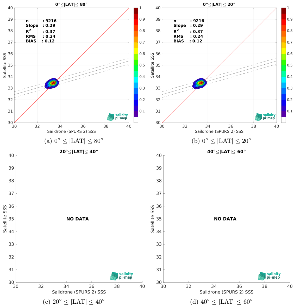
Figure 9: Contour maps of the concentration of SMOS SSS L3 v9 - 18 Days (CATDS-CEC-LOCEAN) SSS (y-axis) versus Saildrone (SPURS 2) SSS (x-axis) at match-up pairs for different latitude bands. For each plot, the red line shows x=y . The black thin and dashed lines indicate a linear fit through the data cloud and the \pm 95\% confidence levels, respectively. The number match-up pairs n , the slope and R^2 coefficient of the linear fit, the root mean square (RMS) and the mean bias between satellite and in situ data are indicated for each latitude band in each plots.
