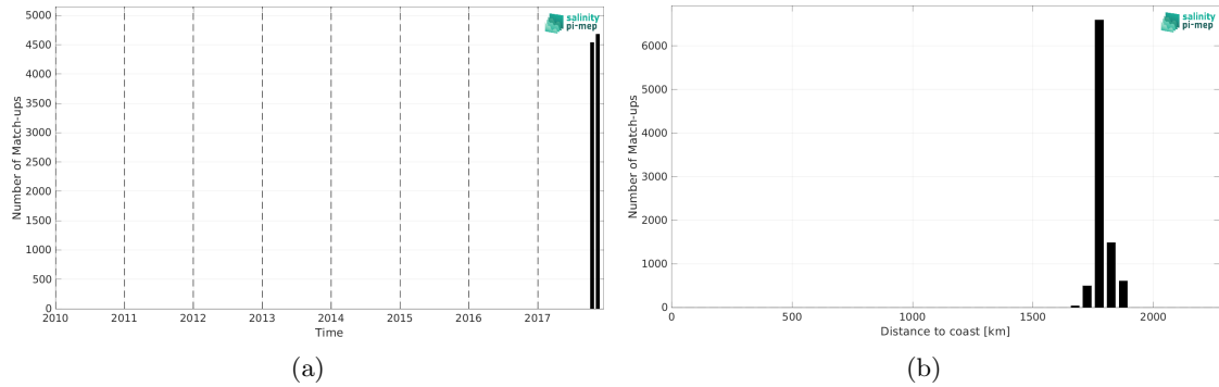
Figure 1: Number of match-ups between Saildrone (SPURS 2) and SMOS SSS L3 v9 - 18 Days (CATDS-CEC-LOCEAN) SSS as a function of time (a) and as function of the distance to coast (b) over the SPURS 2 Pi-MEP region and for the full satellite product period.
