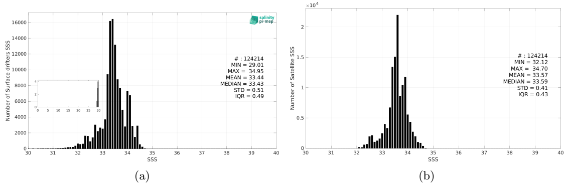
Figure 2: Histograms of SSS from Surface drifters (a) and SMOS SSS L3 v9 - 18 Days (CATDS-CEC-LOCEAN) (b) considering all match-up pairs per bins of 0.1 over the SPURS 2 Pi-MEP region and for the full satellite product period.
