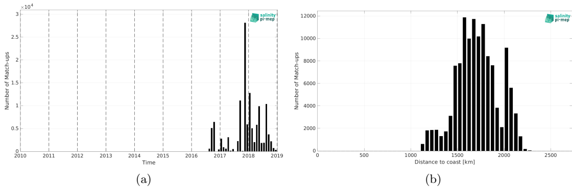
Figure 1: Number of match-ups between Surface drifters and SMOS SSS L3 v9 - 18 Days (CATDS-CEC-LOCEAN) SSS as a function of time (a) and as function of the distance to coast (b) over the SPURS 2 Pi-MEP region and for the full satellite product period.
