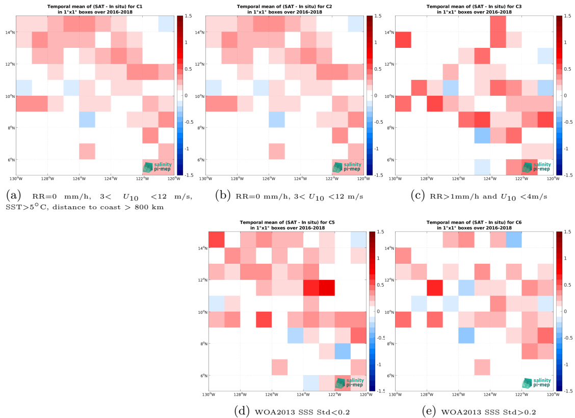
Figure 11: Temporal mean gridded over spatial boxes of size 1^\circ \times 1^\circ of \Delta\text{SSS} (SMOS SSS L3 v9 - 18 Days (CATDS-CEC-LOCEAN) - Surface drifters) for 5 different subdatasets corresponding to: RR=0 mm/h, 3 < U_{10} < 12 m/s, SST > 5^\circ\text{C} , distance to coast > 800 km (a), RR=0 mm/h, 3 < U_{10} < 12 m/s (b), RR > 1 mm/h and U_{10} < 4 m/s (c), WOA2013 SSS Std < 0.2 (d), WOA2013 SSS Std > 0.2 (e).
