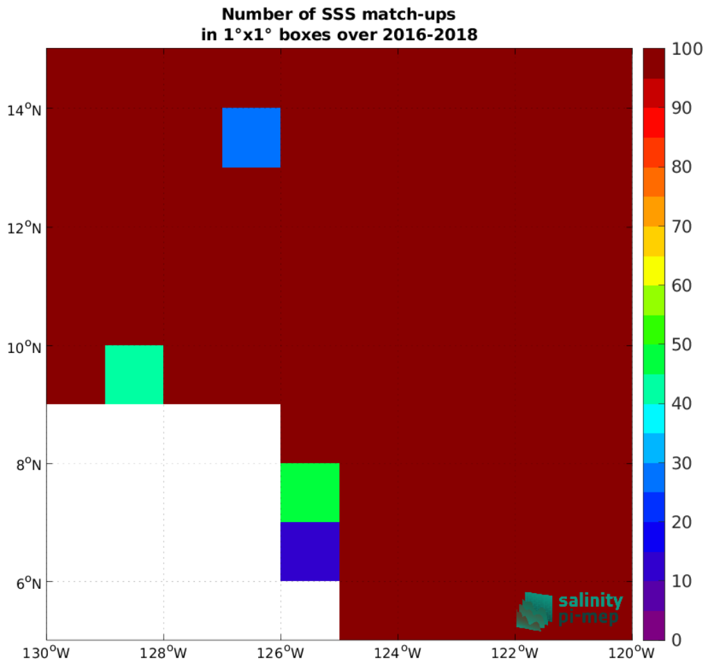
Figure 3: Number of SSS match-ups between Surface drifters SSS and the SMOS SSS L3 v9 - 18 Days (CATDS-CEC-LOCEAN) SSS product for the SPURS 2 Pi-MEP region over 1°x1° boxes and for the full satellite product period.
