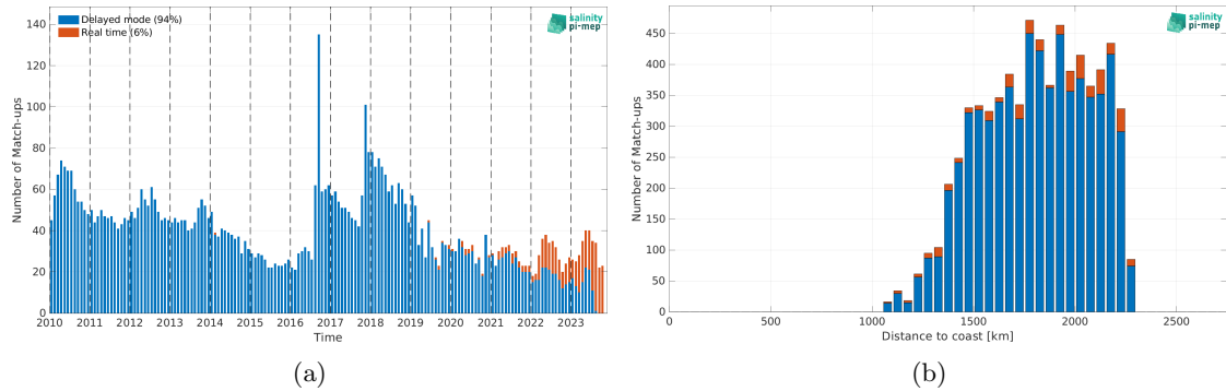
Figure 1: Number of match-ups between Argo and SMOS SSS L3 v9 - 18 Days (CATDS-CEC-LOCEAN) SSS as a function of time (a) and as function of the distance to coast (b) over the SPURS 2 Pi-MEP region and for the full satellite product period.
