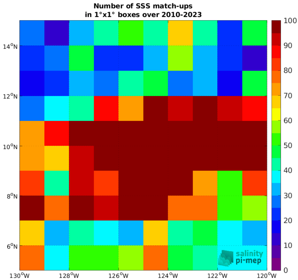
Figure 4: Number of SSS match-ups between Argo SSS and the SMOS SSS L3 v9 - 18 Days (CATDS-CEC-LOCEAN) SSS product for the SPURS 2 Pi-MEP region over 1°x1° boxes and for the full satellite product period.
