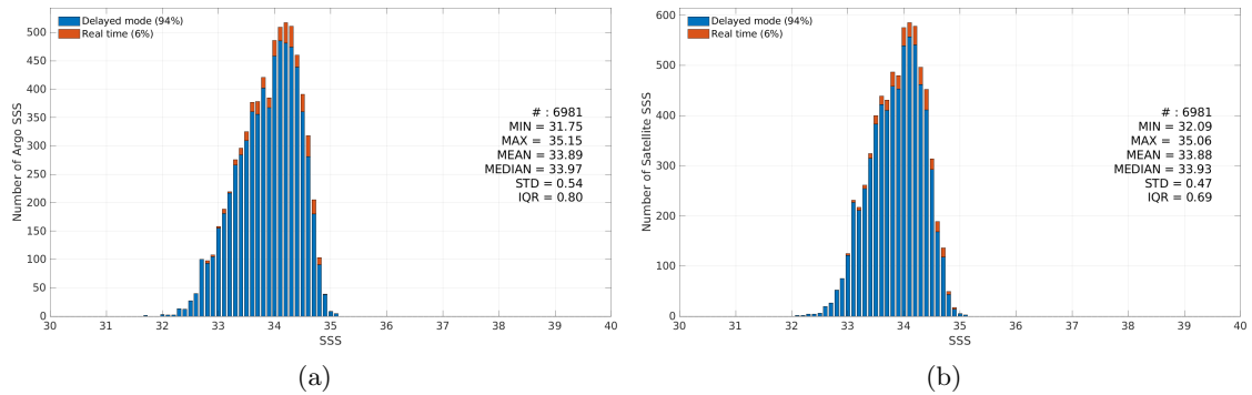
Figure 2: Histograms of SSS from Argo (a) and SMOS SSS L3 v9 - 18 Days (CATDS-CEC-LOCEAN) (b) considering all match-up pairs per bins of 0.1 over the SPURS 2 Pi-MEP region and for the full satellite product period.
