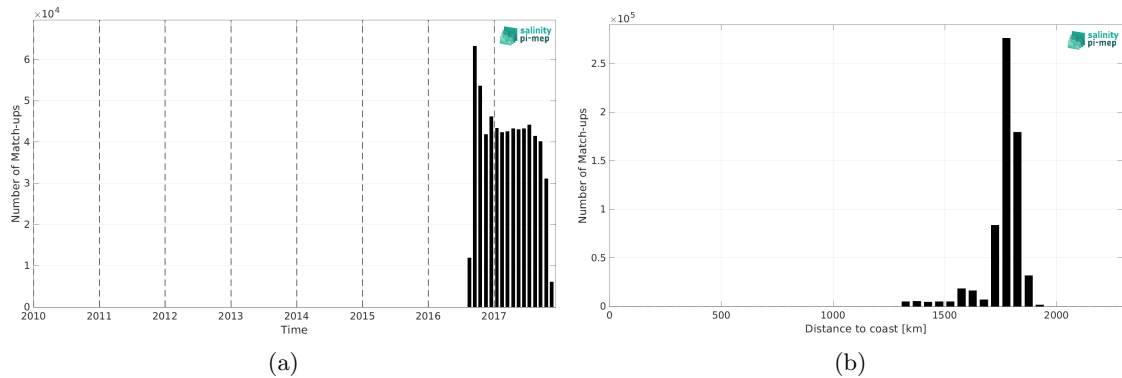
Figure 1: Number of match-ups between Waveglider (SPURS 2) and SMOS SSS L3 v8 - 9 Days (CATDS-CEC-LOCEAN) SSS as a function of time (a) and as function of the distance to coast (b) over the SPURS 2 Pi-MEP region and for the full satellite product period.
