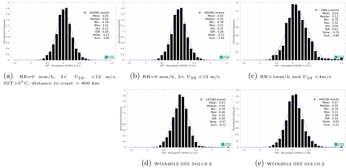
Figure 13: Normalized histogram of \Delta SSS (SMOS SSS L3 v8 - 9 Days (CATDS-CEC-LOCEAN) - Waveglider (SPURS 2)) for 5 different subdatasets corresponding to: RR=0 mm/h, 3 < U_{10} < 12 m/s, SST>5°C, distance to coast > 800 km (a), RR=0 mm/h, 3 < U_{10} < 12 m/s (b), RR>1mm/h and U_{10} < 4 m/s (c), WOA2013 SSS Std<0.2 (d), WOA2013 SSS Std>0.2 (e).
