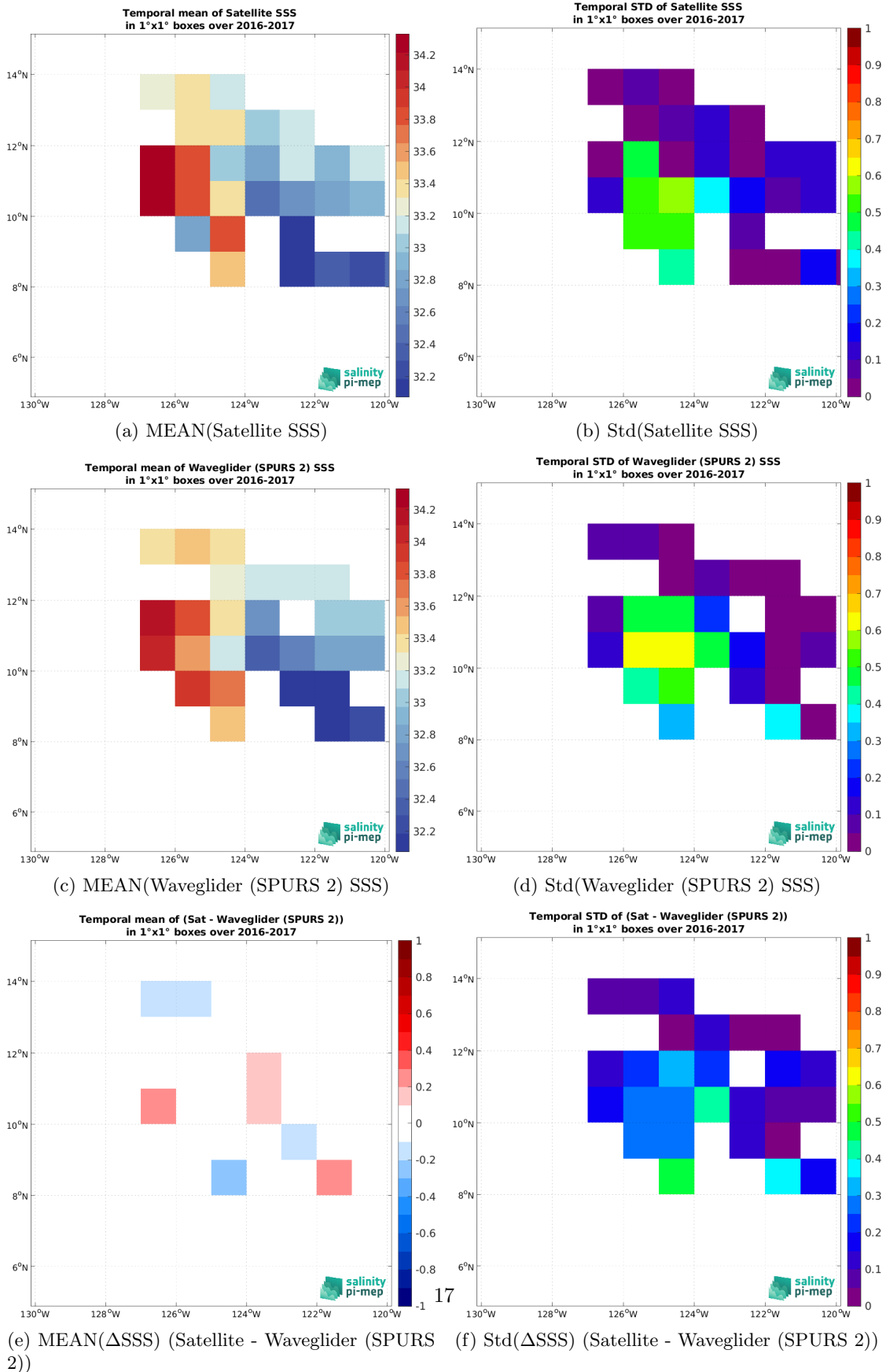
Figure 6: Temporal mean (left) and Std (right) of SSS from SMOS SSS L3 v8 - 9 Days (CATDS-CEC-LOCEAN) (top), Waveglider (SPURS 2) (middle), and of \Delta SSS (Satellite - Waveglider (SPURS 2)). Only match-up pairs are used to generate these maps.
