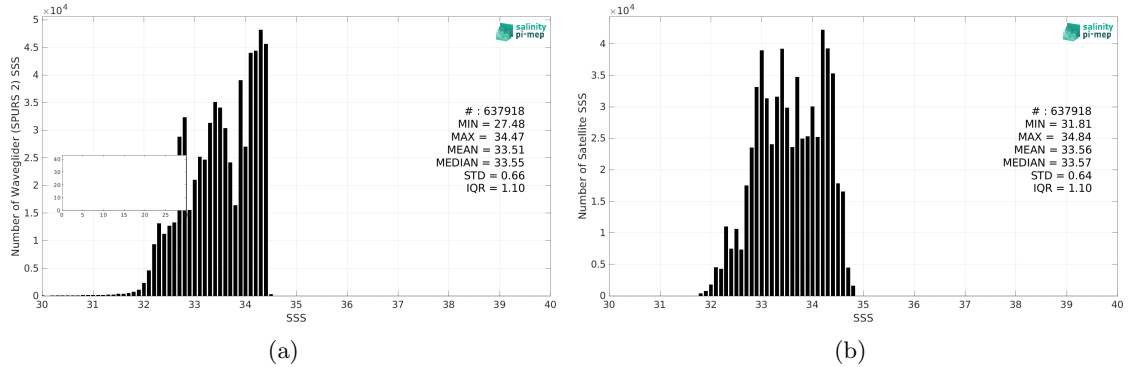
Figure 2: Histograms of SSS from Waveglider (SPURS 2) (a) and SMOS SSS L3 v8 - 9 Days (CATDS-CEC-LOCEAN) (b) considering all match-up pairs per bins of 0.1 over the SPURS 2 Pi-MEP region and for the full satellite product period.
