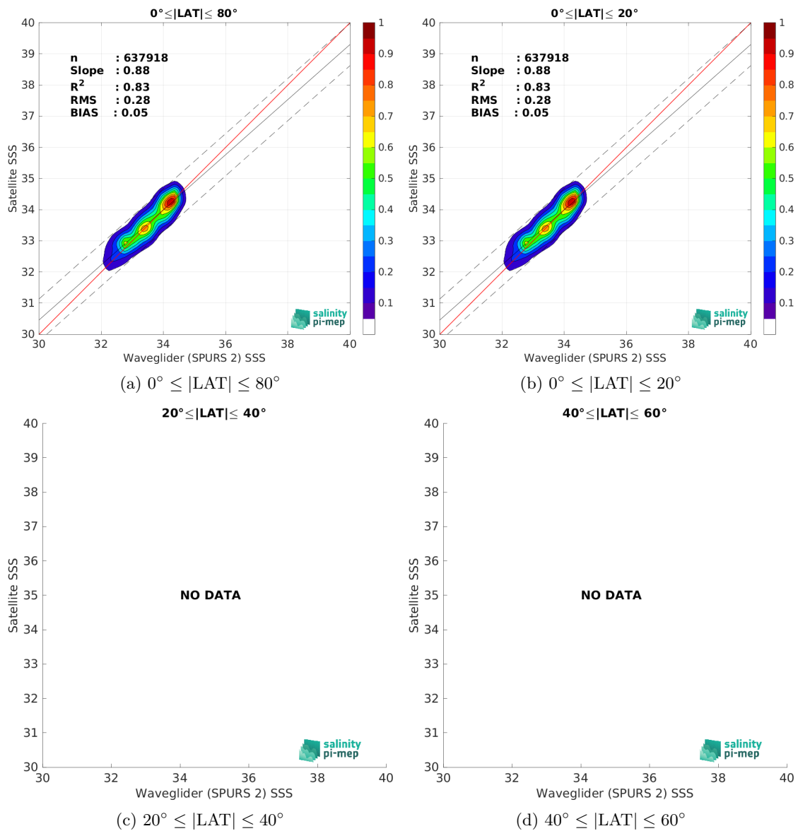
Figure 9: Contour maps of the concentration of SMOS SSS L3 v8 - 9 Days (CATDS-CEC-LOCEAN) SSS (y-axis) versus Waveglider (SPURS 2) SSS (x-axis) at match-up pairs for different latitude bands. For each plot, the red line shows x=y . The black thin and dashed lines indicate a linear fit through the data cloud and the \pm 95\% confidence levels, respectively. The number match-up pairs n , the slope and R^2 coefficient of the linear fit, the root mean square (RMS) and the mean bias between satellite and in situ data are indicated for each latitude band in each plots.
