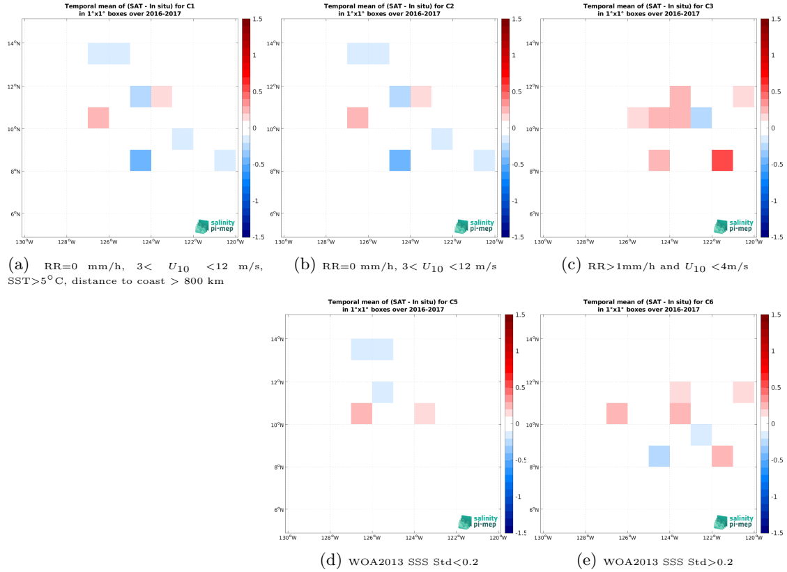
Figure 12: Temporal mean gridded over spatial boxes of size 1^{\circ}\times 1^{\circ} of \Delta\text{SSS} (SMOS SSS L3 v8 - 9 Days (CATDS-CEC-LOCEAN) - Waveglider (SPURS 2)) for 5 different subdatasets corresponding to:RR=0 mm/h, 3 < U_{10} < 12 m/s, SST >5^{\circ}\text{C} , distance to coast > 800 km (a), RR=0 mm/h, 3 < U_{10} < 12 m/s (b), RR >1 mm/h and U_{10} < 4 m/s (c), WOA2013 SSS Std <0.2 (d), WOA2013 SSS Std >0.2 (e).
