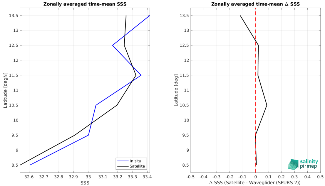
Figure 8: Left panel: Zonal mean SSS from SMOS SSS L3 v8 - 9 Days (CATDS-CEC-LOCEAN) satellite product (black) and from Waveglider (SPURS 2) (blue). Right panel: Zonal mean of \Delta SSS (Satellite - Waveglider (SPURS 2)) for all the collected Pi-MEP match-up pairs estimated over the full satellite product period.
