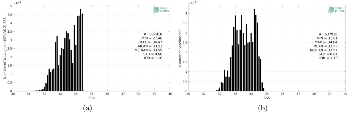
Figure 2: Histograms of SSS from Waveglider (SPURS 2) (a) and SMOS SSS L3 v8 - 9 Days (CATDS-CECOS-LOCEAN) (b) considering all match-up pairs per bins of 0.1 over the SPURS 2 Pi-MEP region and for the full satellite product period.
