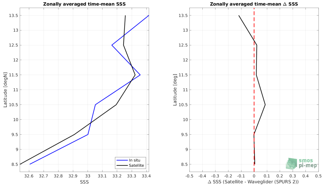
Figure 8: Left panel: Zonal mean SSS from SMOS SSS L3 v8 - 9 Days (CATDS-CECOS-LOCEAN) satellite product (black) and from Waveglider (SPURS 2) (blue). Right panel: Zonal mean of \Delta SSS (Satellite - Waveglider (SPURS 2)) for all the collected Pi-MEP match-up pairs estimated over the full satellite product period.
