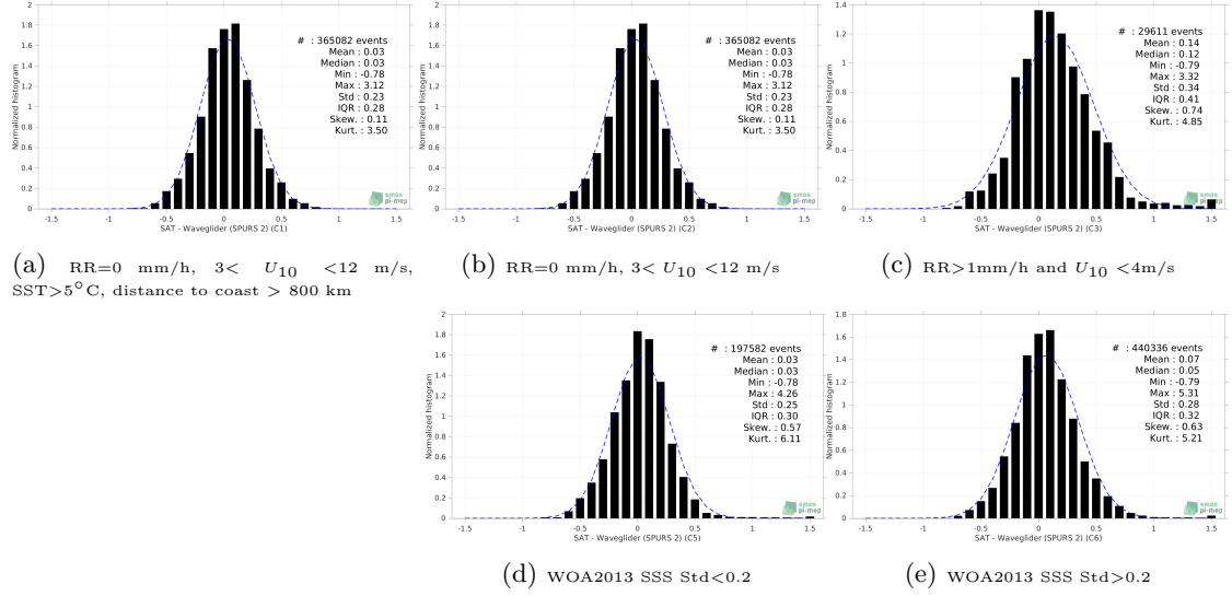
Figure 13: Normalized histogram of \Delta SSS (SMOS SSS L3 v8 - 9 Days (CATDS-CECOS-LOCEAN) - Waveglider (SPURS 2)) for 5 different subdatasets corresponding to: RR=0 mm/h, 3 < U_{10} < 12 m/s, SST > 5°C, distance to coast > 800 km (a), RR=0 mm/h, 3 < U_{10} < 12 m/s (b), RR > 1mm/h and U_{10} < 4 m/s (c), WOA2013 SSS Std < 0.2 (d), WOA2013 SSS Std > 0.2 (e).
