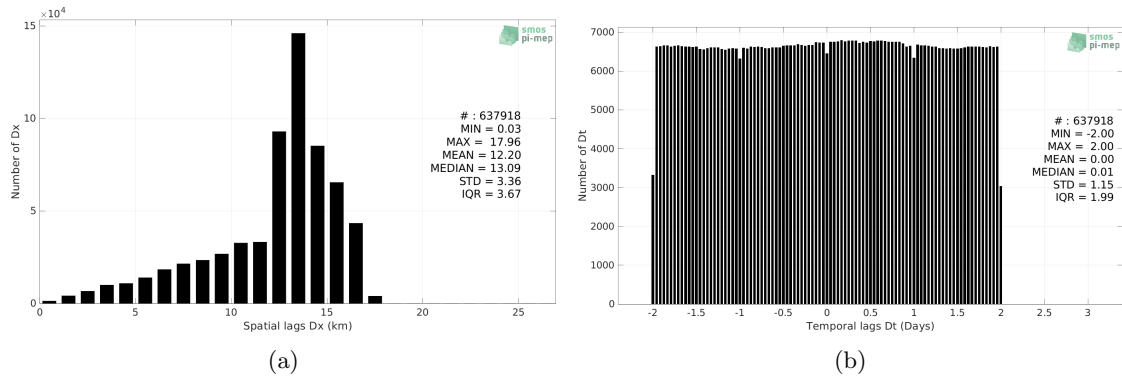
Figure 5: Histograms of the spatial (a) and temporal (b) lags between the location/time of the Waveglider (SPURS 2) measurement and the date of the corresponding SMOS SSS L3 v8 - 9 Days (CATDS-CECOS-LOCEAN) SSS pixel.
