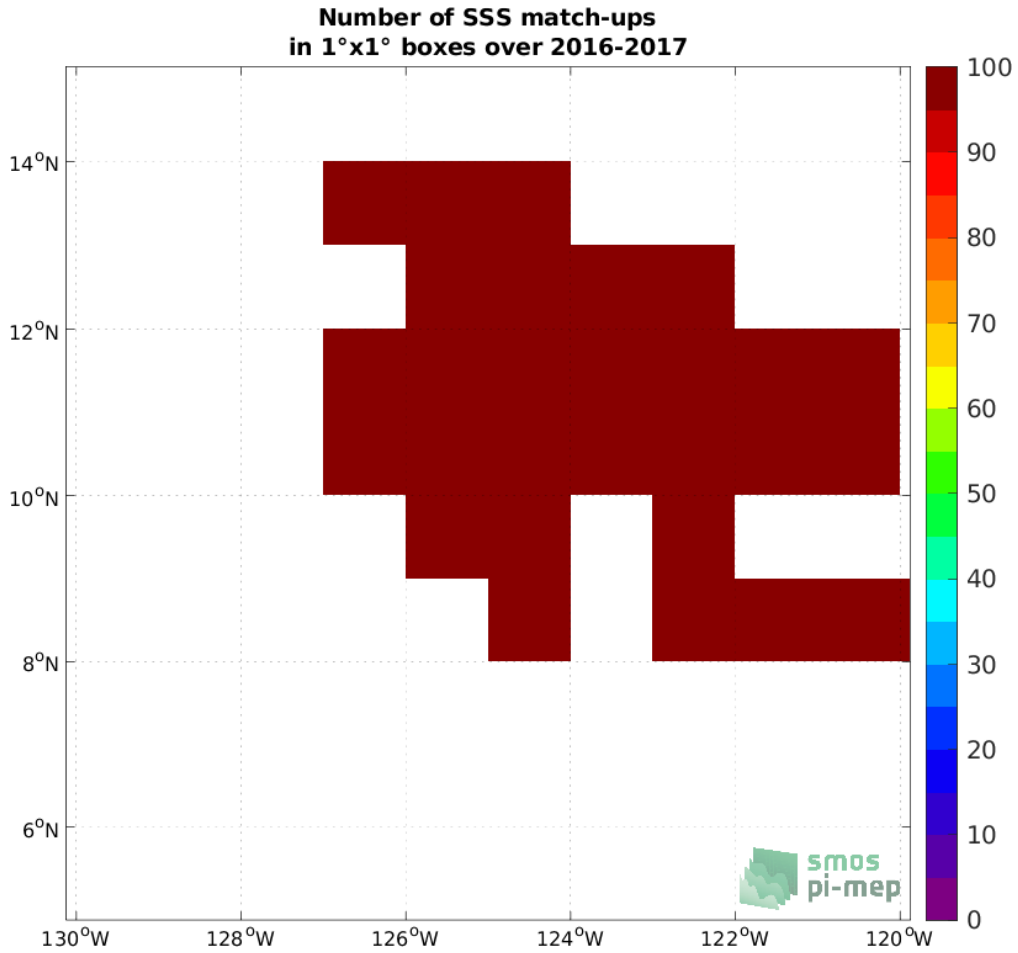
Figure 4: Number of SSS match-ups between Waveglider (SPURS 2) SSS and the SMOS SSS L3 v8 - 9 Days (CATDS-CECOS-LOCEAN) SSS product for the SPURS 2 Pi-MEP region over 1°x1° boxes and for the full satellite product period.
