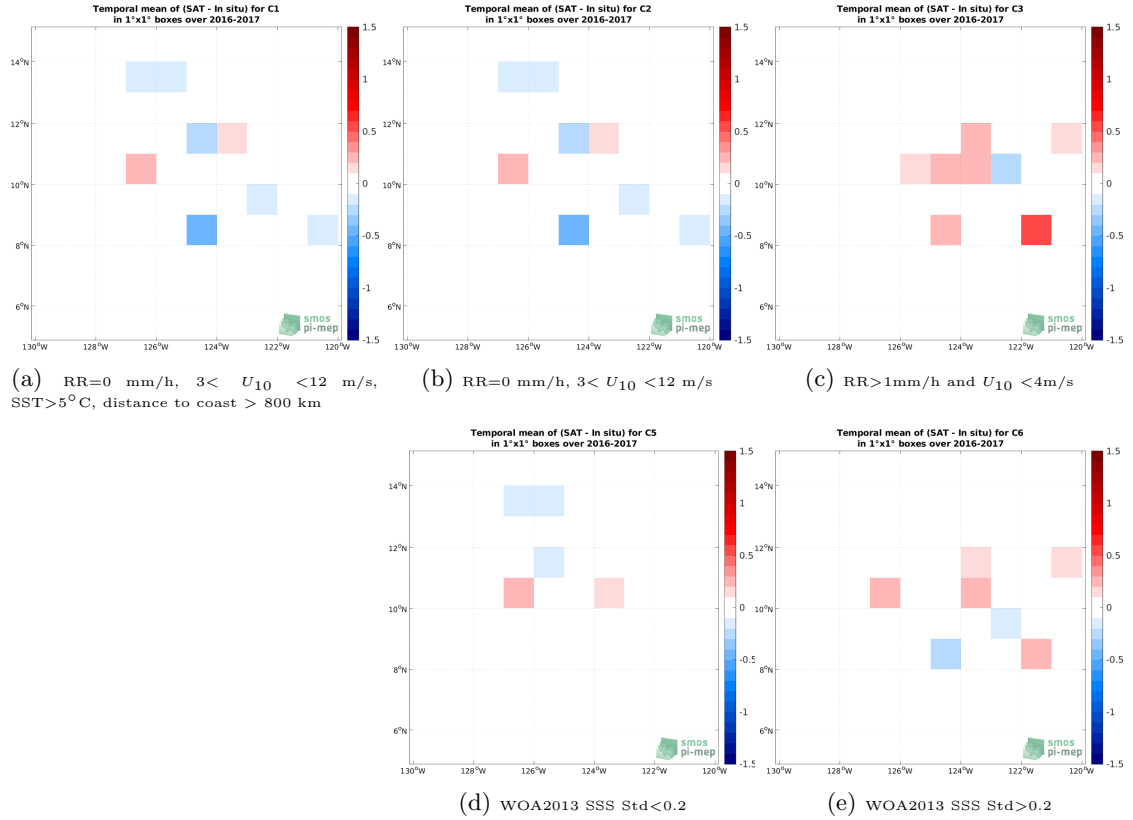
Figure 12: Temporal mean gridded over spatial boxes of size 1^{\circ}\times 1^{\circ} of \Delta\text{SSS} (SMOS SSS L3 v8 - 9 Days (CATDS-CECOS-LOCEAN) - Waveglider (SPURS 2)) for 5 different subdatasets corresponding to:RR=0 mm/h, 3 < U_{10} < 12 m/s, SST >5^{\circ}\text{C} , distance to coast > 800 km (a), RR=0 mm/h, 3 < U_{10} < 12 m/s (b), RR >1 mm/h and U_{10} < 4 m/s (c), WOA2013 SSS Std <0.2 (d), WOA2013 SSS Std >0.2 (e).
