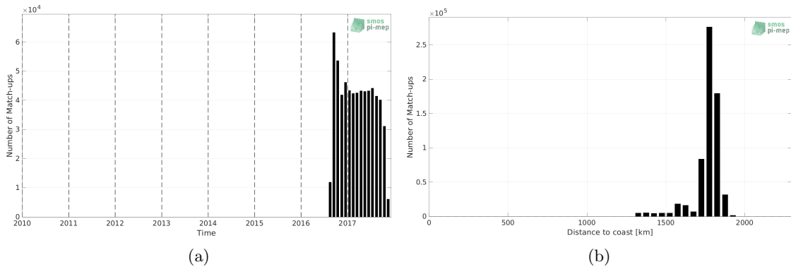
Figure 1: Number of match-ups between Waveglider (SPURS 2) and SMOS SSS L3 v8 - 9 Days (CATDS-CECOS-LOCEAN) SSS as a function of time (a) and as function of the distance to coast (b) over the SPURS 2 Pi-MEP region and for the full satellite product period.
