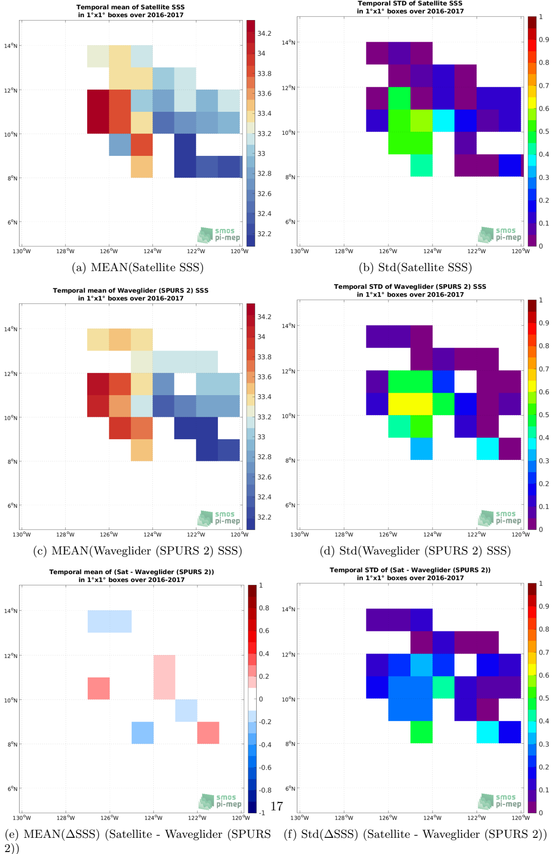
Figure 6: Temporal mean (left) and Std (right) of SSS from SMOS SSS L3 v8 - 9 Days (CATDS-CECOS-LOCEAN) (top), Waveglider (SPURS 2) (middle), and of \Delta SSS (Satellite - Waveglider (SPURS 2)). Only match-up pairs are used to generate these maps.
