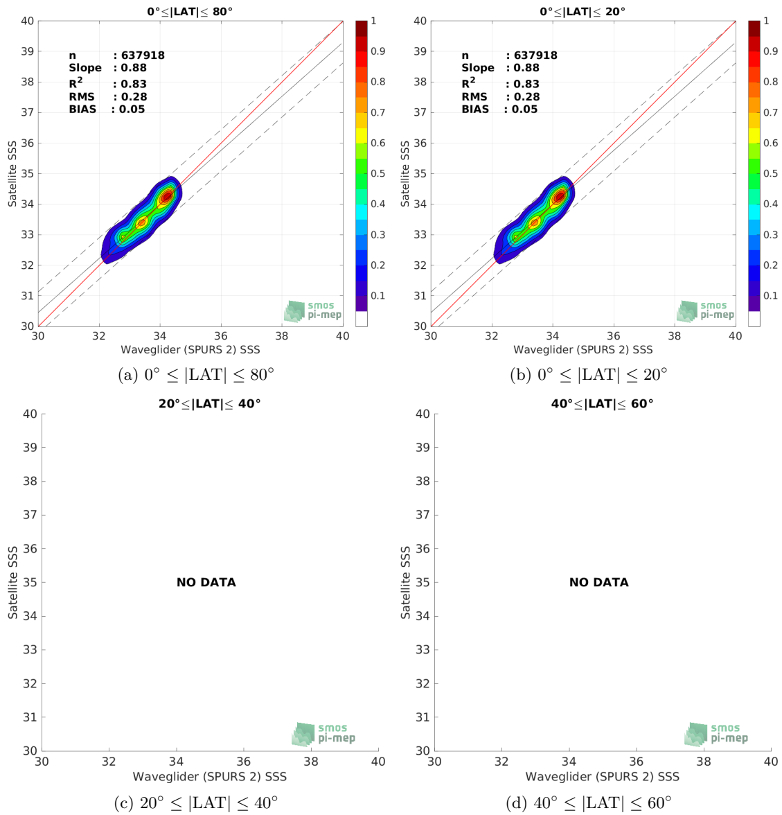
Figure 9: Contour maps of the concentration of SMOS SSS L3 v8 - 9 Days (CATDS-CECOS-LOCEAN) SSS (y-axis) versus Waveglider (SPURS 2) SSS (x-axis) at match-up pairs for different latitude bands. For each plot, the red line shows x=y . The black thin and dashed lines indicate a linear fit through the data cloud and the \pm 95\% confidence levels, respectively. The number match-up pairs n , the slope and R^2 coefficient of the linear fit, the root mean square (RMS) and the mean bias between satellite and in situ data are indicated for each latitude band in each plots.
