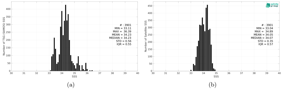
Figure 2: Histograms of SSS from TSG (SAMOS) (a) and SMOS SSS L3 v8 - 9 Days (CATDS-CEC-LOCEAN) (b) considering all match-up pairs per bins of 0.1 over the SPURS 2 Pi-MEP region and for the full satellite product period.
