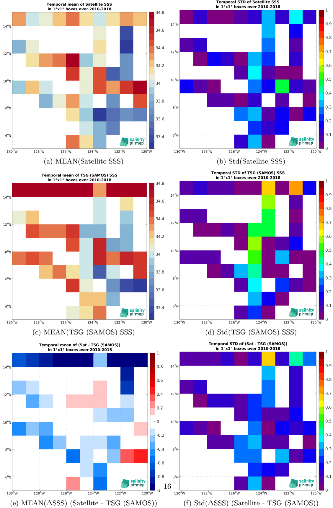
Figure 6: Temporal mean (left) and Std (right) of SSS from SMOS SSS L3 v8 - 9 Days (CATDS-CEC-LOCEAN) (top), TSG (SAMOS) (middle), and of \Delta SSS (Satellite - TSG (SAMOS)). Only match-up pairs are used to generate these maps.
