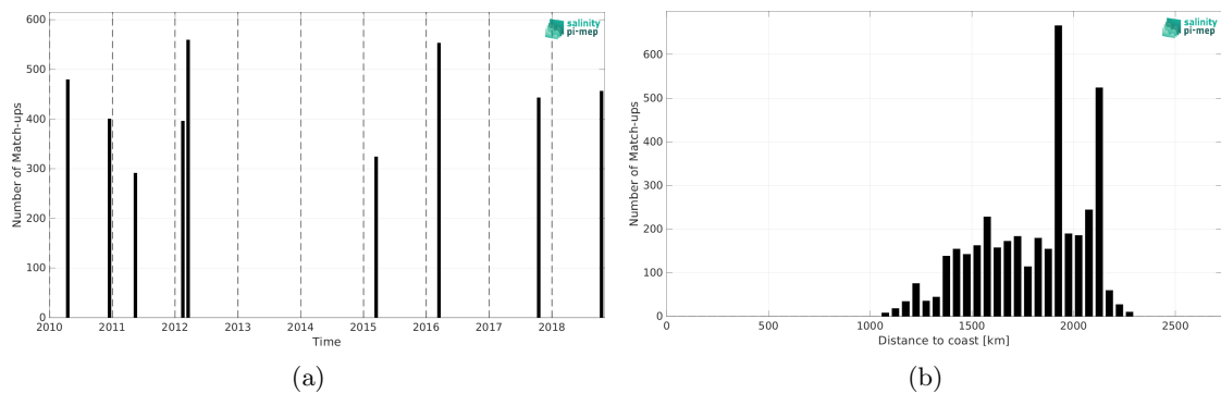
Figure 1: Number of match-ups between TSG (SAMOS) and SMOS SSS L3 v8 - 9 Days (CATDS-CEC-LOCEAN) SSS as a function of time (a) and as function of the distance to coast (b) over the SPURS 2 Pi-MEP region and for the full satellite product period.
