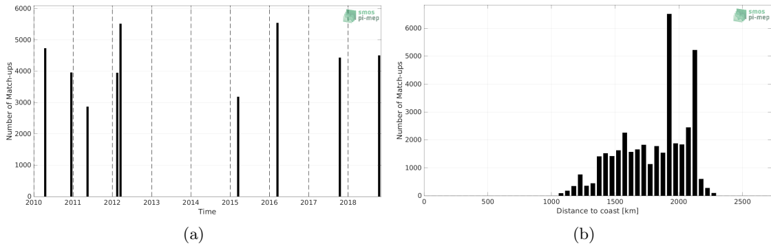
Figure 1: Number of match-ups between TSG (SAMOS) and SMOS SSS L3 v8 - 9 Days (CATDS-CECOS-LOCEAN) SSS as a function of time (a) and as function of the distance to coast (b) over the SPURS 2 Pi-MEP region and for the full satellite product period.
