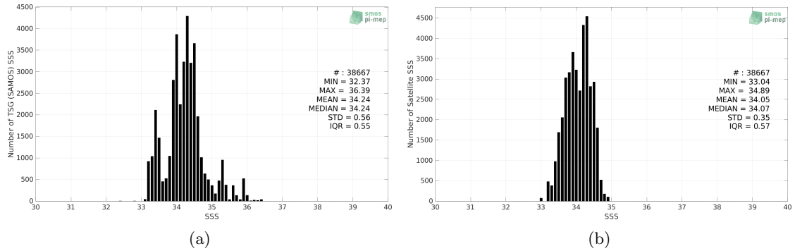
Figure 2: Histograms of SSS from TSG (SAMOS) (a) and SMOS SSS L3 v8 - 9 Days (CATDS-CECOS-LOCEAN) (b) considering all match-up pairs per bins of 0.1 over the SPURS 2 Pi-MEP region and for the full satellite product period.
