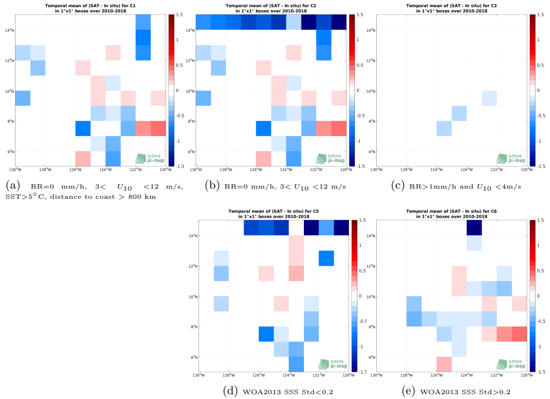
Figure 12: Temporal mean gridded over spatial boxes of size 1^{\circ}\times 1^{\circ} of \Delta\text{SSS} (SMOS SSS L3 v8 - 9 Days (CATDS-CECOS-LOCEAN) - TSG (SAMOS)) for 5 different subdatasets corresponding to:RR=0 mm/h, 3 < U_{10} < 12 m/s, SST > 5^{\circ}\text{C} , distance to coast > 800 km (a), RR=0 mm/h, 3 < U_{10} < 12 m/s (b), RR > 1 mm/h and U_{10} < 4 m/s (c), WOA2013 SSS Std < 0.2 (d), WOA2013 SSS Std > 0.2 (e).
