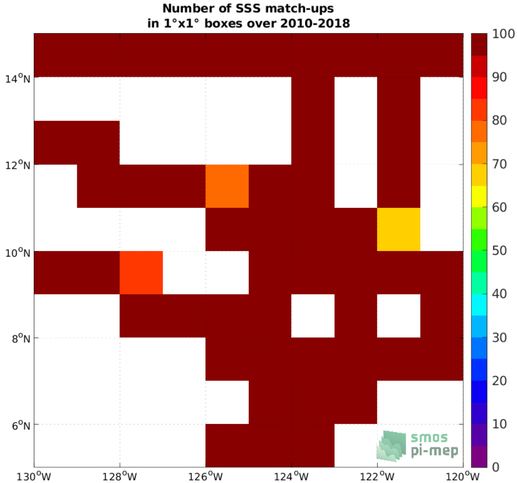
Figure 4: Number of SSS match-ups between TSG (SAMOS) SSS and the SMOS SSS L3 v8 - 9 Days (CATDS-CECOS-LOCEAN) SSS product for the SPURS 2 Pi-MEP region over 1^\circ \times 1^\circ boxes and for the full satellite product period.
