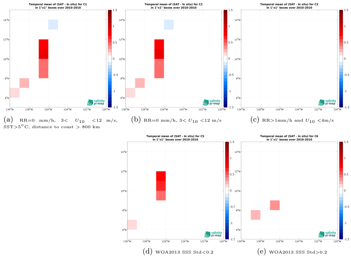
Figure 12: Temporal mean gridded over spatial boxes of size 1^\circ \times 1^\circ of \Delta SSS (SMOS SSS L3 v8 - 9 Days (CATDS-CEC-LOCEAN) - TSG (GOSUD-Sailing-ship)) for 5 different subdatasets corresponding to: RR=0 mm/h, 3 < U_{10} < 12 m/s, SST > 5°C, distance to coast > 800 km (a), RR=0 mm/h, 3 < U_{10} < 12 m/s (b), RR > 1mm/h and U_{10} < 4 m/s (c), WOA2013 SSS Std < 0.2 (d), WOA2013 SSS Std > 0.2 (e).
