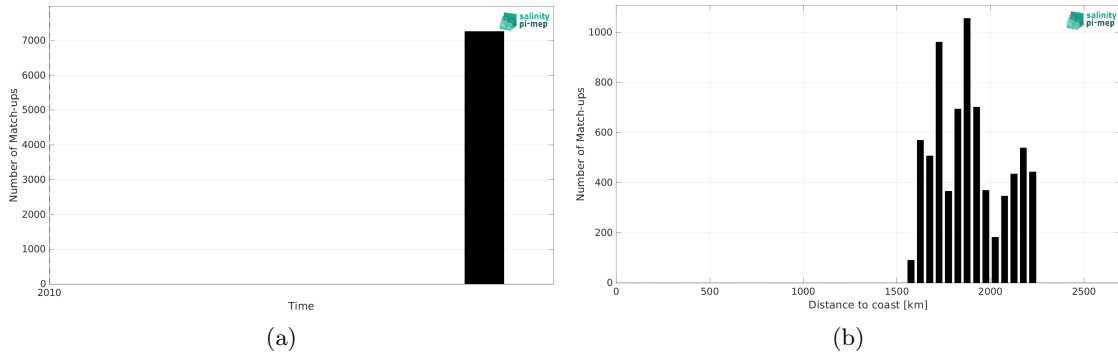
Figure 1: Number of match-ups between TSG (GOSUD-Sailing-ship) and SMOS SSS L3 v8 - 9 Days (CATDS-CEC-LOCEAN) SSS as a function of time (a) and as function of the distance to coast (b) over the SPURS 2 Pi-MEP region and for the full satellite product period.
