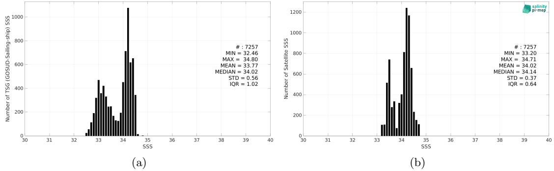
Figure 2: Histograms of SSS from TSG (GOSUD-Sailing-ship) (a) and SMOS SSS L3 v8 - 9 Days (CATDS-CEC-LOCEAN) (b) considering all match-up pairs per bins of 0.1 over the SPURS 2 Pi-MEP region and for the full satellite product period.
