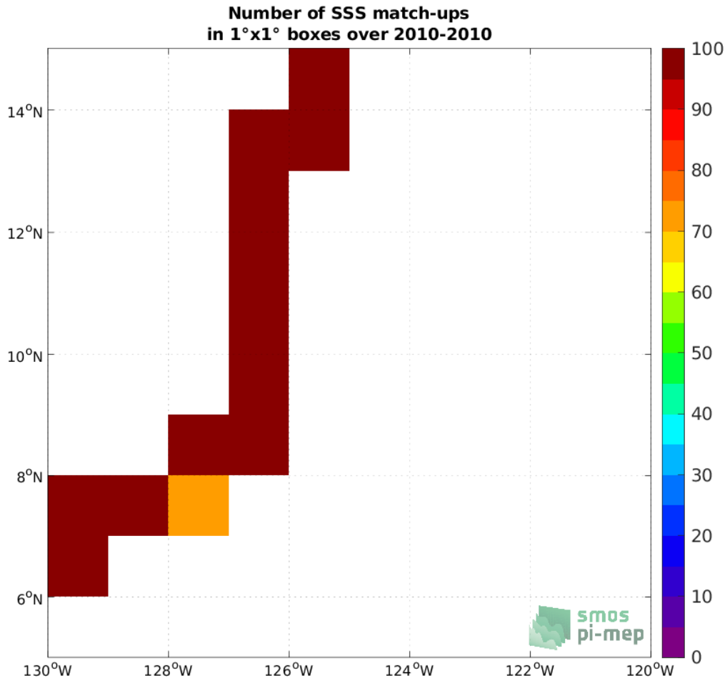
Figure 4: Number of SSS match-ups between TSG (GOSUD-Sailing-ship) SSS and the SMOS SSS L3 v8 - 9 Days (CATDS-CECOS-LOCEAN) SSS product for the SPURS 2 Pi-MEP region over 1^\circ \times 1^\circ boxes and for the full satellite product period.
