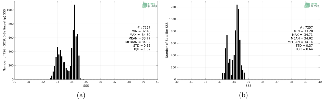
Figure 2: Histograms of SSS from TSG (GOSUD-Sailing-ship) (a) and SMOS SSS L3 v8 - 9 Days (CATDS-CECOS-LOCEAN) (b) considering all match-up pairs per bins of 0.1 over the SPURS 2 Pi-MEP region and for the full satellite product period.
