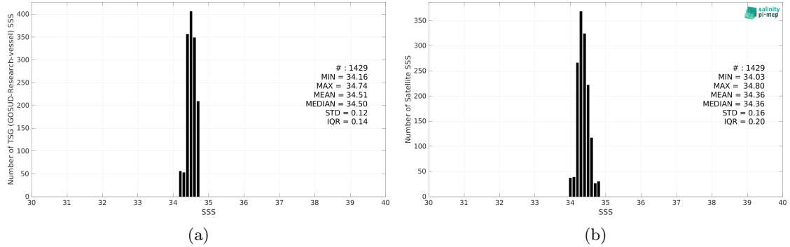
Figure 2: Histograms of SSS from TSG (GOSUD-Research-vessel) (a) and SMOS SSS L3 v8 - 9 Days (CATDS-CEC-LOCEAN) (b) considering all match-up pairs per bins of 0.1 over the SPURS 2 Pi-MEP region and for the full satellite product period.
