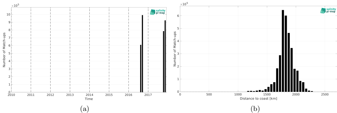
Figure 1: Number of match-ups between Salinity Snake (SPURS 2) and SMOS SSS L3 v8 - 9 Days (CATDS-CEC-LOCEAN) SSS as a function of time (a) and as function of the distance to coast (b) over the SPURS 2 Pi-MEP region and for the full satellite product period.
