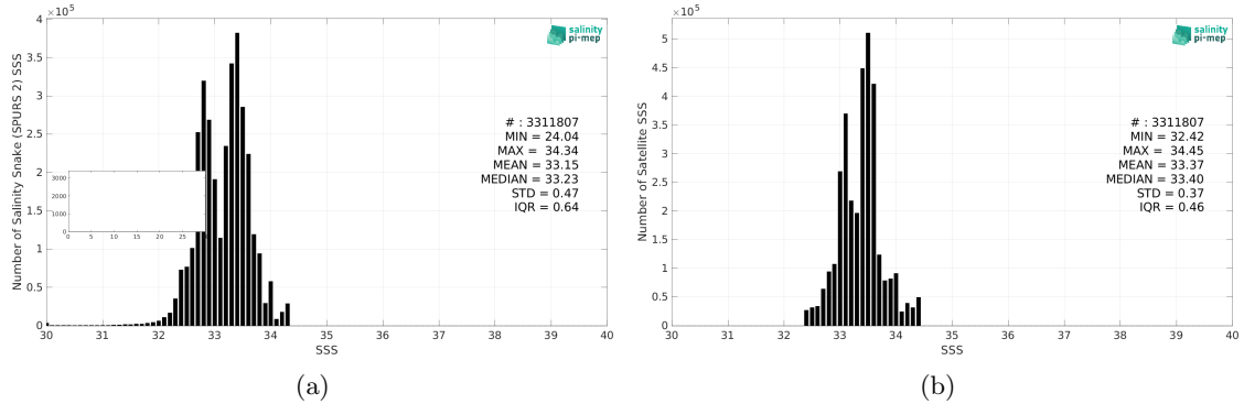
Figure 2: Histograms of SSS from Salinity Snake (SPURS 2) (a) and SMOS SSS L3 v8 - 9 Days (CATDS-CEC-LOCEAN) (b) considering all match-up pairs per bins of 0.1 over the SPURS 2 Pi-MEP region and for the full satellite product period.
