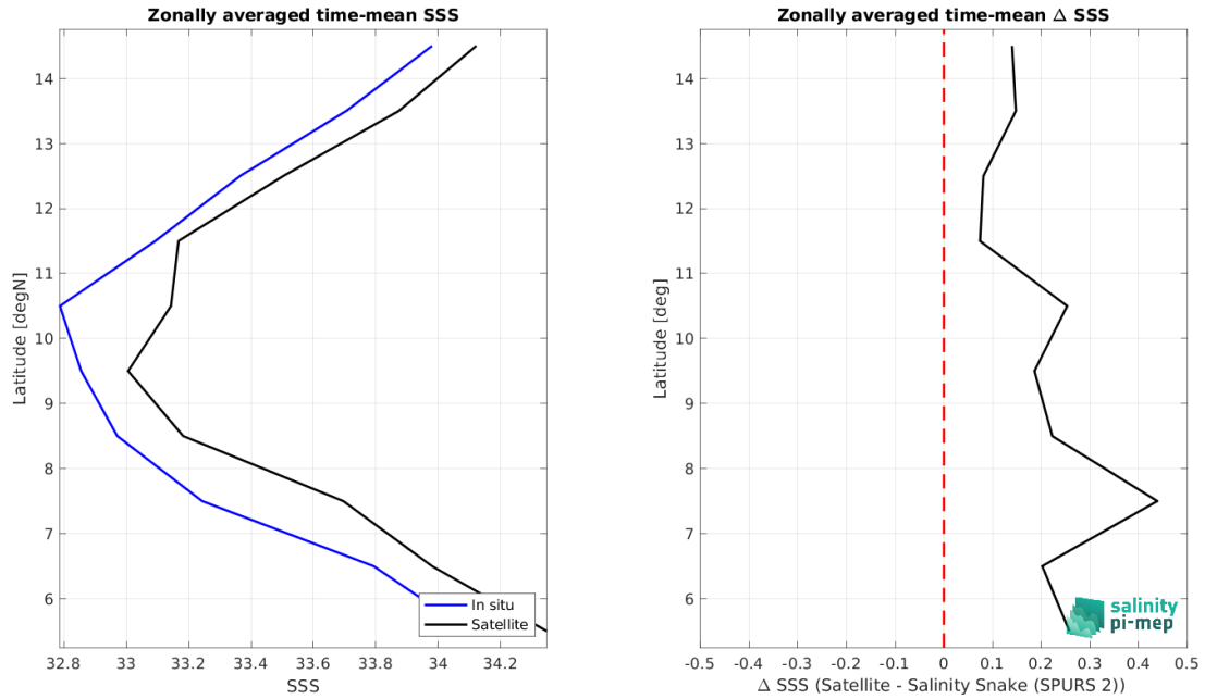
Figure 8: Left panel: Zonal mean SSS from SMOS SSS L3 v8 - 9 Days (CATDS-CEC-LOCEAN) satellite product (black) and from Salinity Snake (SPURS 2) (blue). Right panel: Zonal mean of \Delta SSS (Satellite - Salinity Snake (SPURS 2)) for all the collected Pi-MEP match-up pairs estimated over the full satellite product period.
