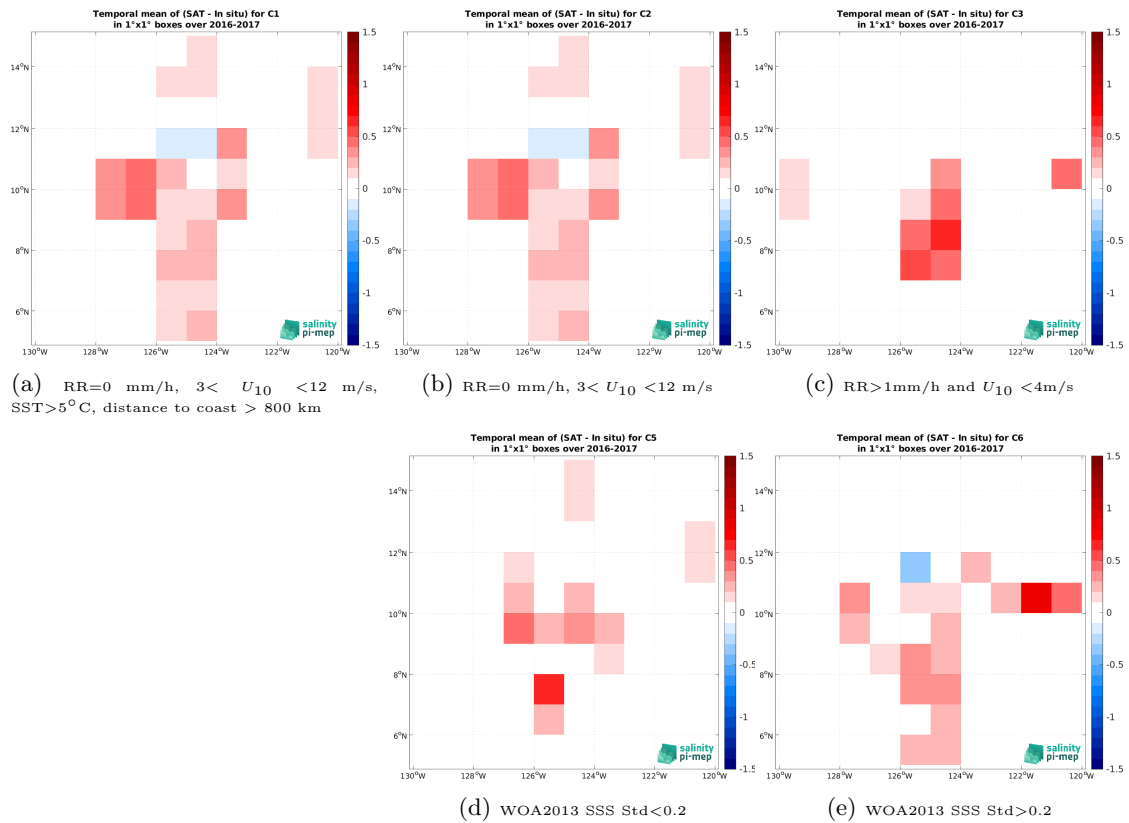
Figure 12: Temporal mean gridded over spatial boxes of size 1^\circ \times 1^\circ of \Delta SSS (SMOS SSS L3 v8 - 9 Days (CATDS-CEC-LOCEAN) - Salinity Snake (SPURS 2)) for 5 different subdatasets corresponding to:RR=0 mm/h, 3 < U_{10} < 12 m/s, SST>5°C, distance to coast > 800 km (a), RR=0 mm/h, 3 < U_{10} < 12 m/s (b), RR>1mm/h and U_{10} < 4 m/s (c), WOA2013 SSS Std<0.2 (d), WOA2013 SSS Std>0.2 (e).
