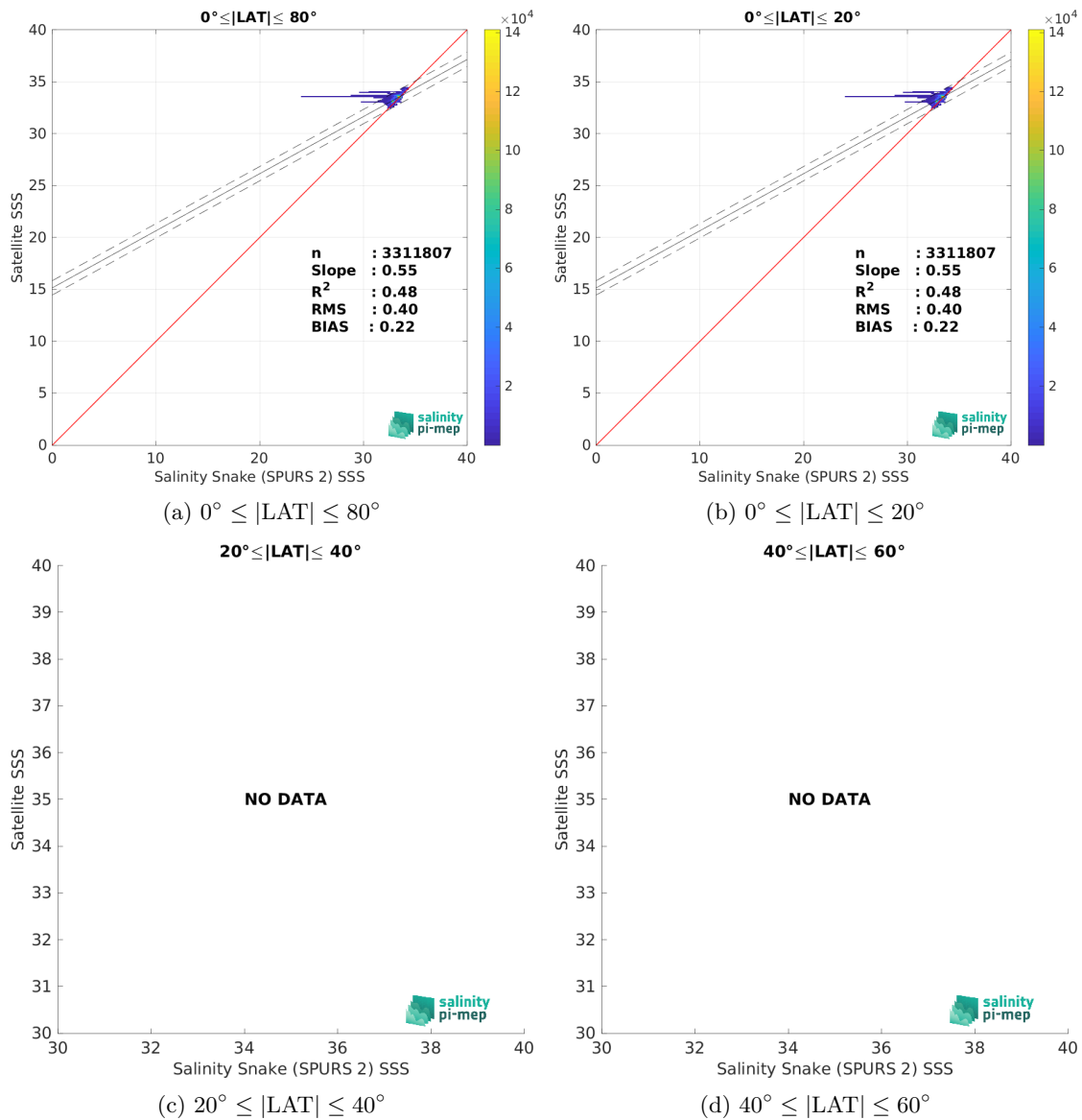
Figure 9: Contour maps of the concentration of SMOS SSS L3 v8 - 9 Days (CATDS-CEC-LOCEAN) SSS (y-axis) versus Salinity Snake (SPURS 2) SSS (x-axis) at match-up pairs for different latitude bands. For each plot, the red line shows x=y . The black thin and dashed lines indicate a linear fit through the data cloud and the \pm 95\% confidence levels, respectively. The number match-up pairs n , the slope and R^2 coefficient of the linear fit, the root mean square (RMS) and the mean bias between satellite and in situ data are indicated for each latitude band in each plots.
