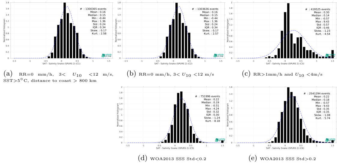
Figure 13: Normalized histogram of \Delta SSS (SMOS SSS L3 v8 - 9 Days (CATDS-CEC-LOCEAN) - Salinity Snake (SPURS 2)) for 5 different subdatasets corresponding to: RR=0 mm/h, 3 < U_{10} < 12 m/s, SST > 5°C, distance to coast > 800 km (a), RR=0 mm/h, 3 < U_{10} < 12 m/s (b), RR > 1mm/h and U_{10} < 4 m/s (c), WOA2013 SSS Std < 0.2 (d), WOA2013 SSS Std > 0.2 (e).
