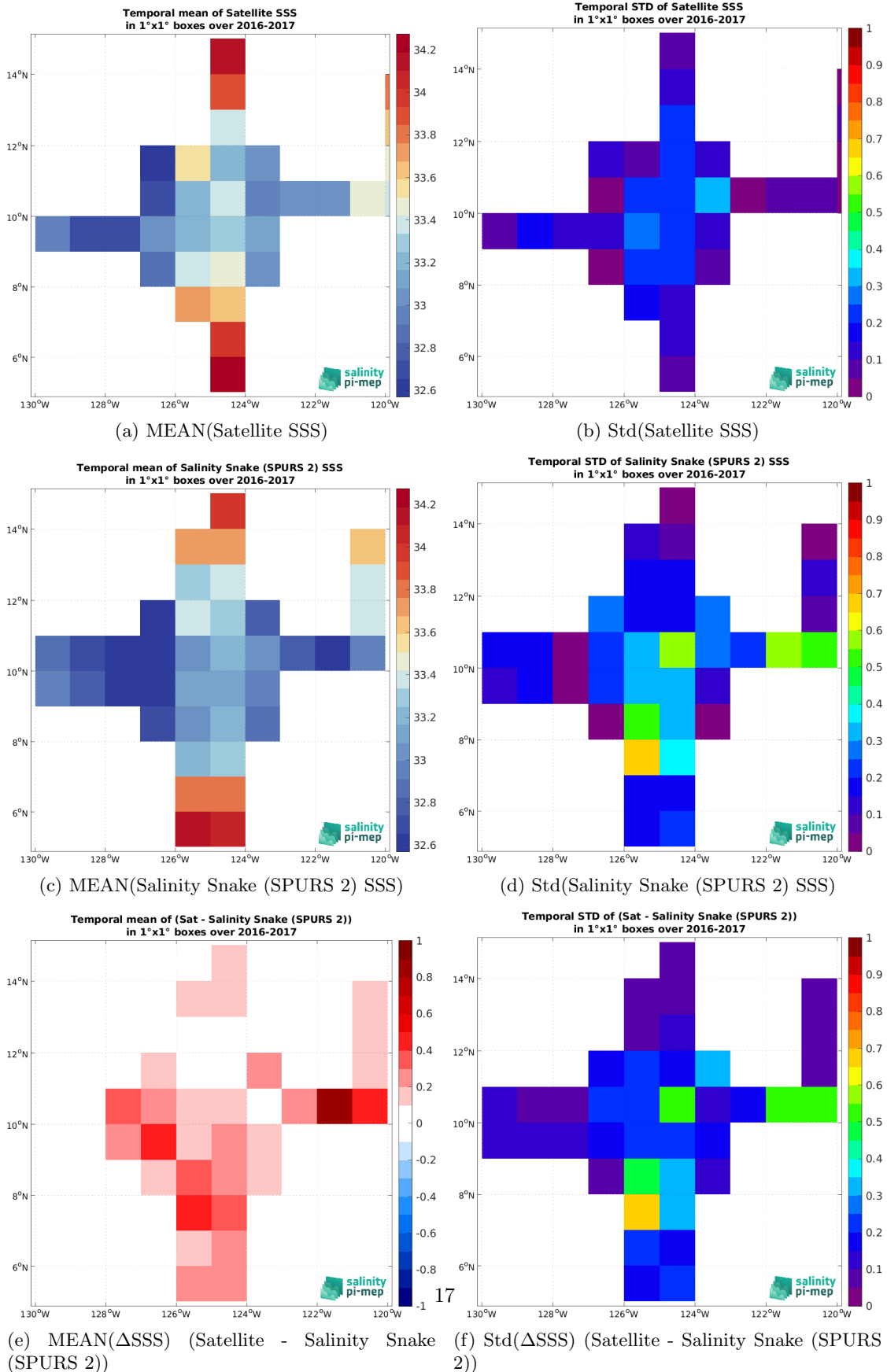
Figure 6: Temporal mean (left) and Std (right) of SSS from SMOS SSS L3 v8 - 9 Days (CATDS-CEC-LOCEAN) (top), Salinity Snake (SPURS 2) (middle), and of \Delta SSS (Satellite - Salinity Snake (SPURS 2)). Only match-up pairs are used to generate these maps.
