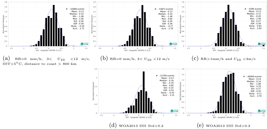
Figure 13: Normalized histogram of \Delta SSS (SMOS SSS L3 v8 - 9 Days (CATDS-CEC-LOCEAN) - Seaglider (SPURS 2)) for 5 different subdatasets corresponding to: RR=0 mm/h, 3 < U_{10} < 12 m/s, SST>5°C, distance to coast > 800 km (a), RR=0 mm/h, 3 < U_{10} < 12 m/s (b), RR>1mm/h and U_{10} < 4 m/s (c), WOA2013 SSS Std<0.2 (d), WOA2013 SSS Std>0.2 (e).
