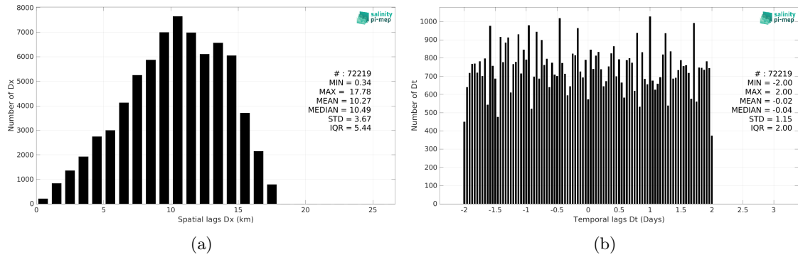
Figure 5: Histograms of the spatial (a) and temporal (b) lags between the location/time of the Seaglider (SPURS 2) measurement and the date of the corresponding SMOS SSS L3 v8 - 9 Days (CATDS-CEC-LOCEAN) SSS pixel.
