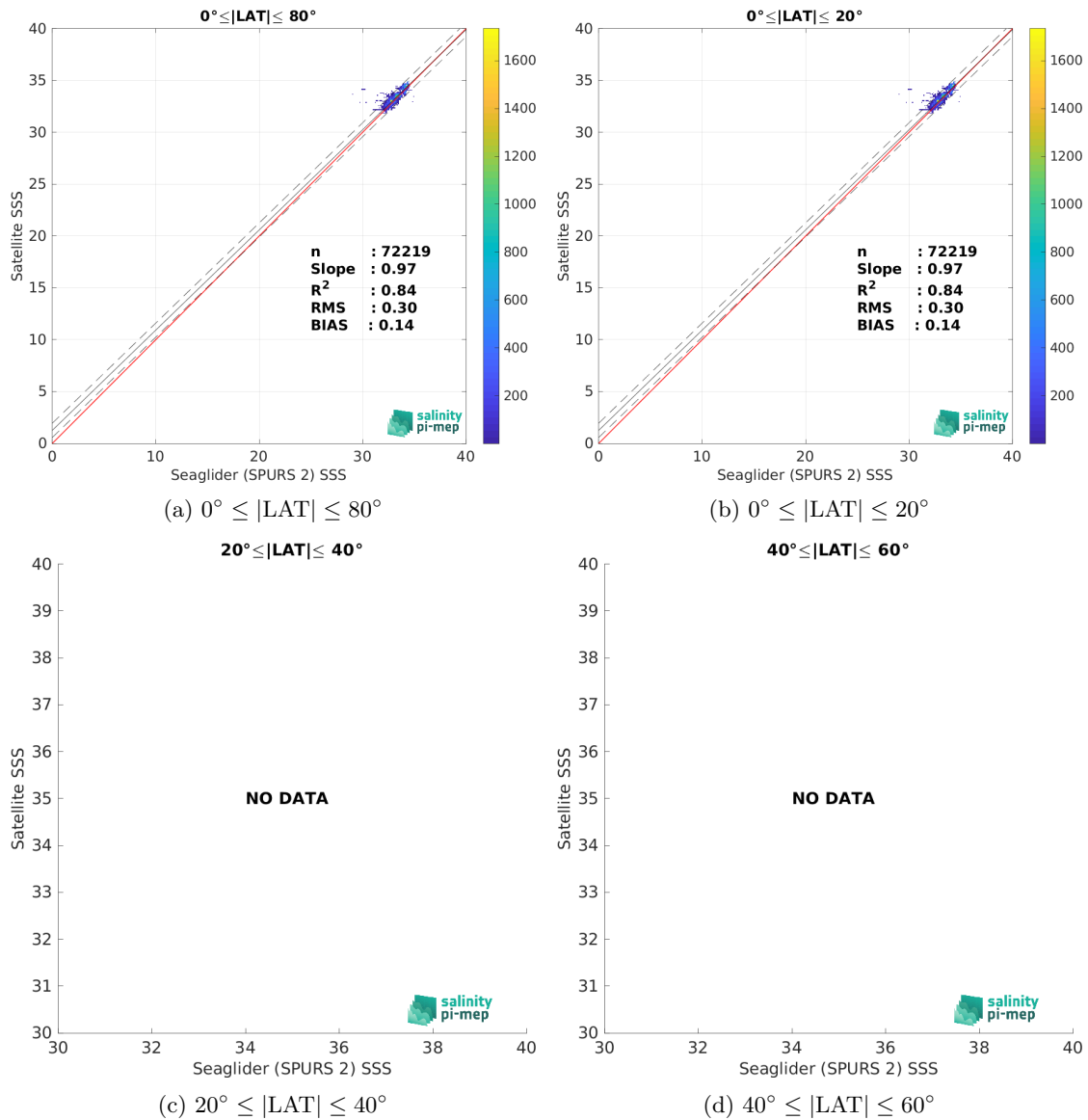
Figure 9: Contour maps of the concentration of SMOS SSS L3 v8 - 9 Days (CATDS-CEC-LOCEAN) SSS (y-axis) versus Seaglider (SPURS 2) SSS (x-axis) at match-up pairs for different latitude bands. For each plot, the red line shows x=y . The black thin and dashed lines indicate a linear fit through the data cloud and the \pm 95\% confidence levels, respectively. The number match-up pairs n , the slope and R^2 coefficient of the linear fit, the root mean square (RMS) and the mean bias between satellite and in situ data are indicated for each latitude band in each plots.
