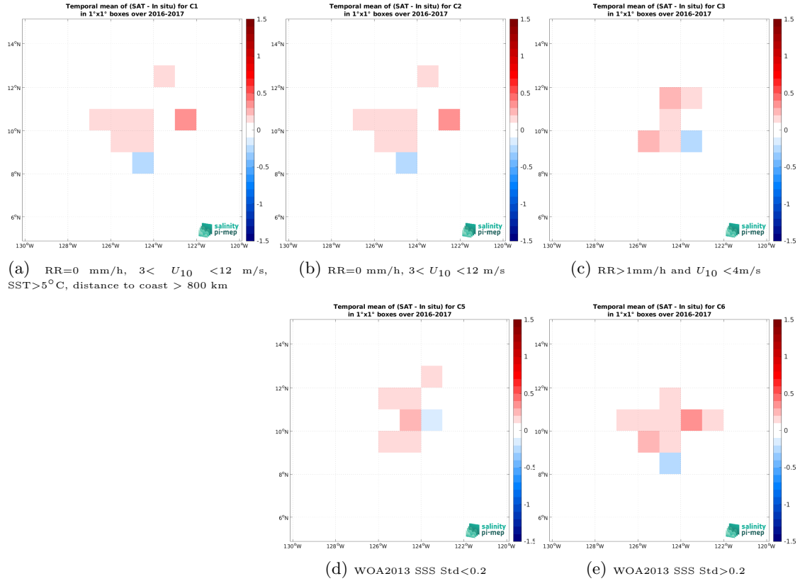
Figure 12: Temporal mean gridded over spatial boxes of size 1^{\circ}\times 1^{\circ} of \Delta\text{SSS} (SMOS SSS L3 v8 - 9 Days (CATDS-CEC-LOCEAN) - Seaglider (SPURS 2)) for 5 different subdatasets corresponding to:RR=0 mm/h, 3 < U_{10} < 12 m/s, SST > 5^{\circ}\text{C} , distance to coast > 800 km (a), RR=0 mm/h, 3 < U_{10} < 12 m/s (b), RR > 1 mm/h and U_{10} < 4 m/s (c), WOA2013 SSS Std < 0.2 (d), WOA2013 SSS Std > 0.2 (e).
