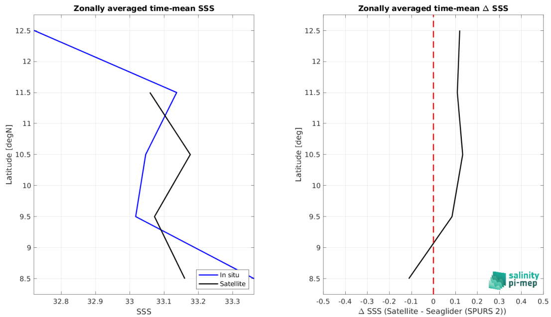
Figure 8: Left panel: Zonal mean SSS from SMOS SSS L3 v8 - 9 Days (CATDS-CEC-LOCEAN) satellite product (black) and from Seaglider (SPURS 2) (blue). Right panel: Zonal mean of \Delta SSS (Satellite - Seaglider (SPURS 2)) for all the collected Pi-MEP match-up pairs estimated over the full satellite product period.
