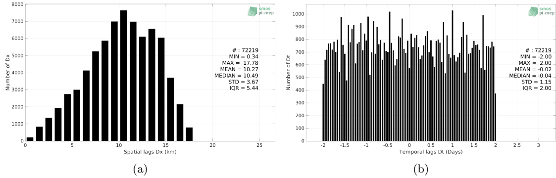
Figure 5: Histograms of the spatial (a) and temporal (b) lags between the location/time of the Seaglider (SPURS 2) measurement and the date of the corresponding SMOS SSS L3 v8 - 9 Days (CATDS-CECOS-LOCEAN) SSS pixel.
