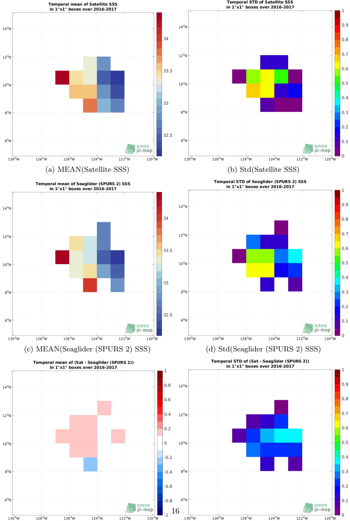
Figure 6: Temporal mean (left) and Std (right) of SSS from SMOS SSS L3 v8 - 9 Days (CATDS-CECOS-LOCEAN) (top), Seaglider (SPURS 2) (middle), and of \Delta SSS (Satellite - Seaglider (SPURS 2)). Only match-up pairs are used to generate these maps.
