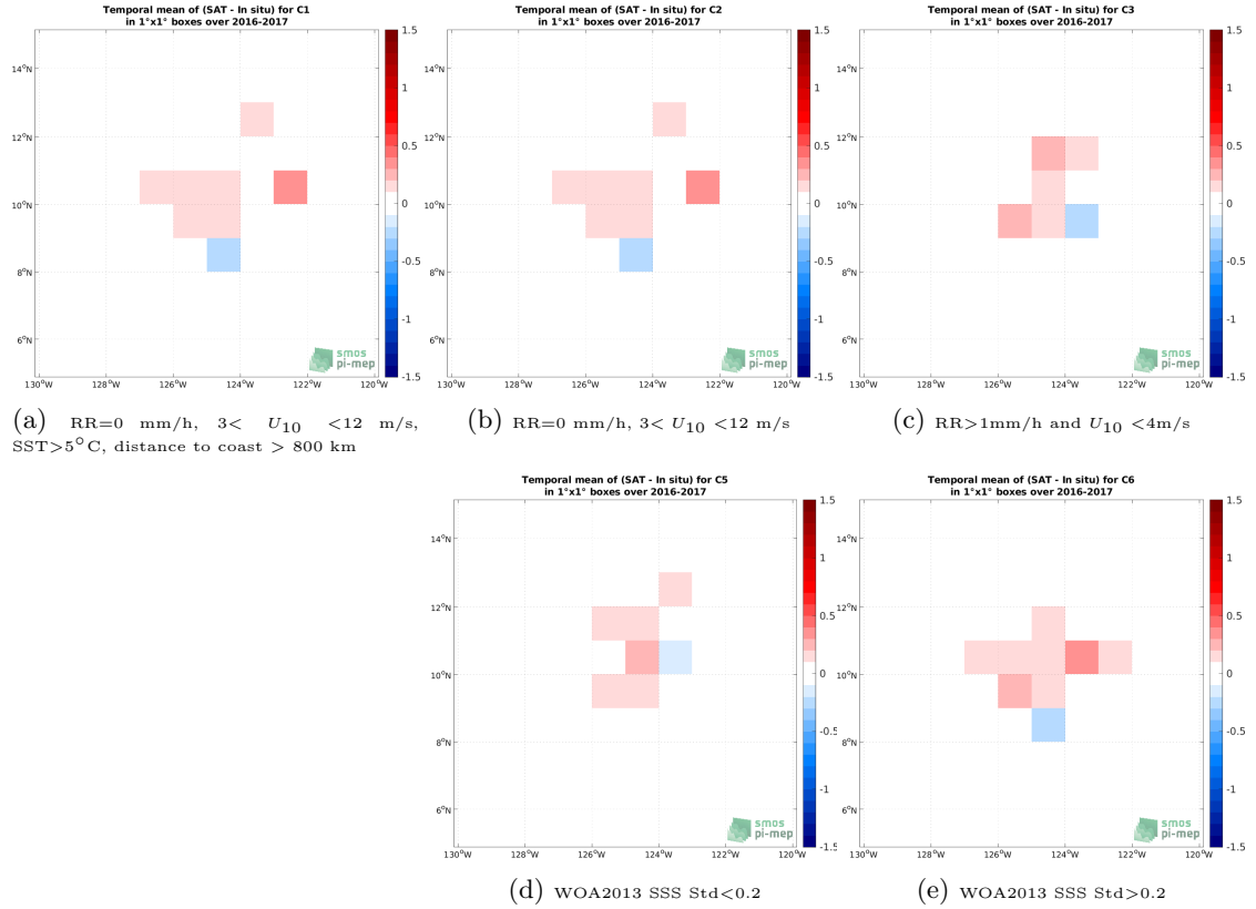
Figure 12: Temporal mean gridded over spatial boxes of size 1^{\circ}\times 1^{\circ} of \Delta\text{SSS} (SMOS SSS L3 v8 - 9 Days (CATDS-CECOS-LOCEAN) - Seaglider (SPURS 2)) for 5 different subdatasets corresponding to:RR=0 mm/h, 3 < U_{10} < 12 m/s, SST >5^{\circ}\text{C} , distance to coast > 800 km (a), RR=0 mm/h, 3 < U_{10} < 12 m/s (b), RR >1 mm/h and U_{10} < 4 m/s (c), WOA2013 SSS Std <0.2 (d), WOA2013 SSS Std >0.2 (e).
