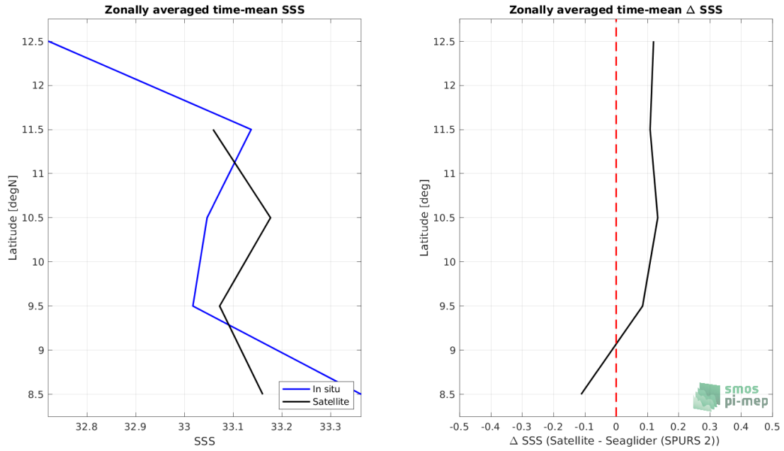
Figure 8: Left panel: Zonal mean SSS from SMOS SSS L3 v8 - 9 Days (CATDS-CECOS-LOCEAN) satellite product (black) and from Seaglider (SPURS 2) (blue). Right panel: Zonal mean of \Delta SSS (Satellite - Seaglider (SPURS 2)) for all the collected Pi-MEP match-up pairs estimated over the full satellite product period.
