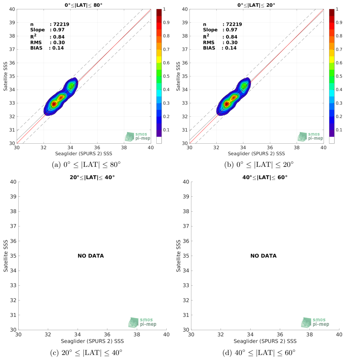
Figure 9: Contour maps of the concentration of SMOS SSS L3 v8 - 9 Days (CATDS-CECOS-LOCEAN) SSS (y-axis) versus Seaglider (SPURS 2) SSS (x-axis) at match-up pairs for different latitude bands. For each plot, the red line shows x=y . The black thin and dashed lines indicate a linear fit through the data cloud and the \pm 95\% confidence levels, respectively. The number match-up pairs n , the slope and R^2 coefficient of the linear fit, the root mean square (RMS) and the mean bias between satellite and in situ data are indicated for each latitude band in each plots.
