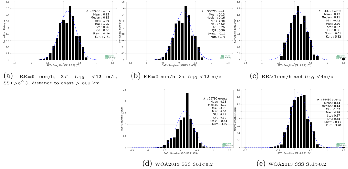
Figure 13: Normalized histogram of \Delta SSS (SMOS SSS L3 v8 - 9 Days (CATDS-CECOS-LOCEAN) - Seaglider (SPURS 2)) for 5 different subdatasets corresponding to: RR=0 mm/h, 3 < U_{10} < 12 m/s, SST > 5°C, distance to coast > 800 km (a), RR=0 mm/h, 3 < U_{10} < 12 m/s (b), RR > 1mm/h and U_{10} < 4 m/s (c), WOA2013 SSS Std < 0.2 (d), WOA2013 SSS Std > 0.2 (e).
