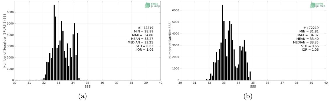
Figure 2: Histograms of SSS from Seaglider (SPURS 2) (a) and SMOS SSS L3 v8 - 9 Days (CATDS-CECOS-LOCEAN) (b) considering all match-up pairs per bins of 0.1 over the SPURS 2 Pi-MEP region and for the full satellite product period.
