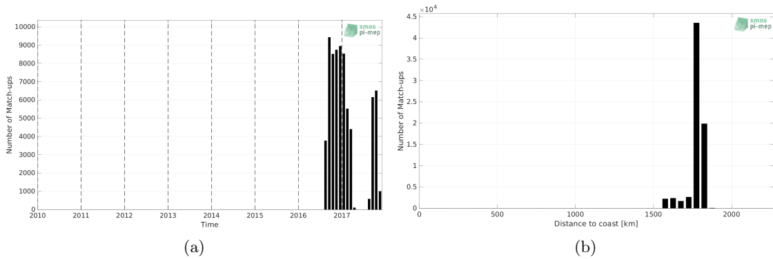
Figure 1: Number of match-ups between Seaglider (SPURS 2) and SMOS SSS L3 v8 - 9 Days (CATDS-CECOS-LOCEAN) SSS as a function of time (a) and as function of the distance to coast (b) over the SPURS 2 Pi-MEP region and for the full satellite product period.
