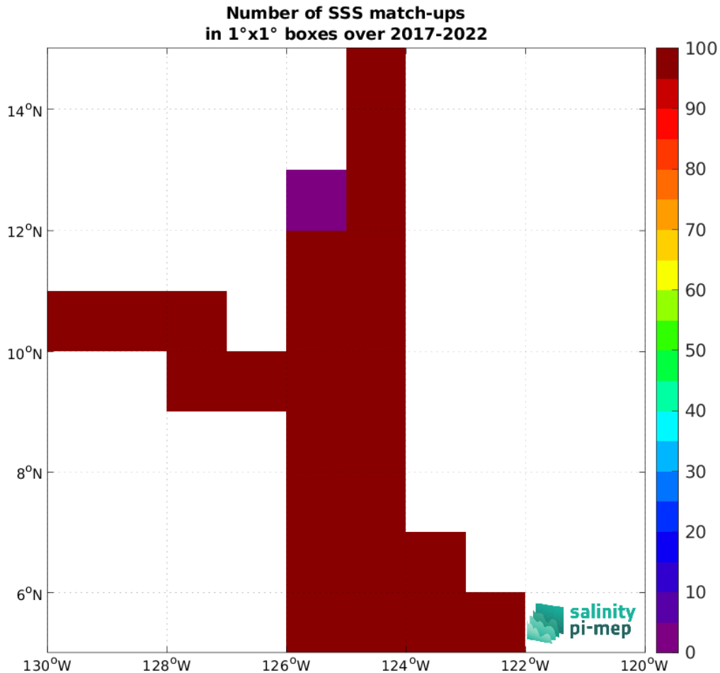
Figure 4: Number of SSS match-ups between Saildrone SSS and the SMOS SSS L3 v8 - 9 Days (CATDS-CEC-LOCEAN) SSS product for the SPURS 2 Pi-MEP region over 1^\circ \times 1^\circ boxes and for the full satellite product period.
