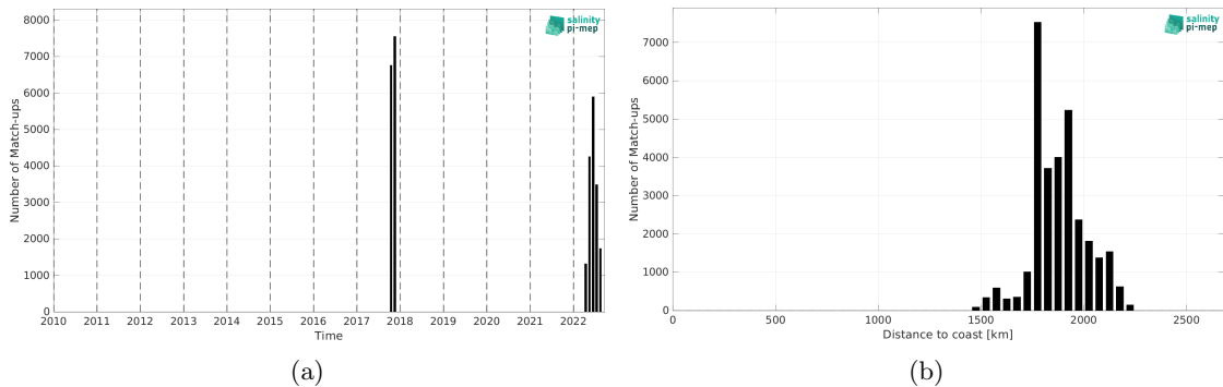
Figure 1: Number of match-ups between Saildrone and SMOS SSS L3 v8 - 9 Days (CATDS-CEC-LOCEAN) SSS as a function of time (a) and as function of the distance to coast (b) over the SPURS 2 Pi-MEP region and for the full satellite product period.
