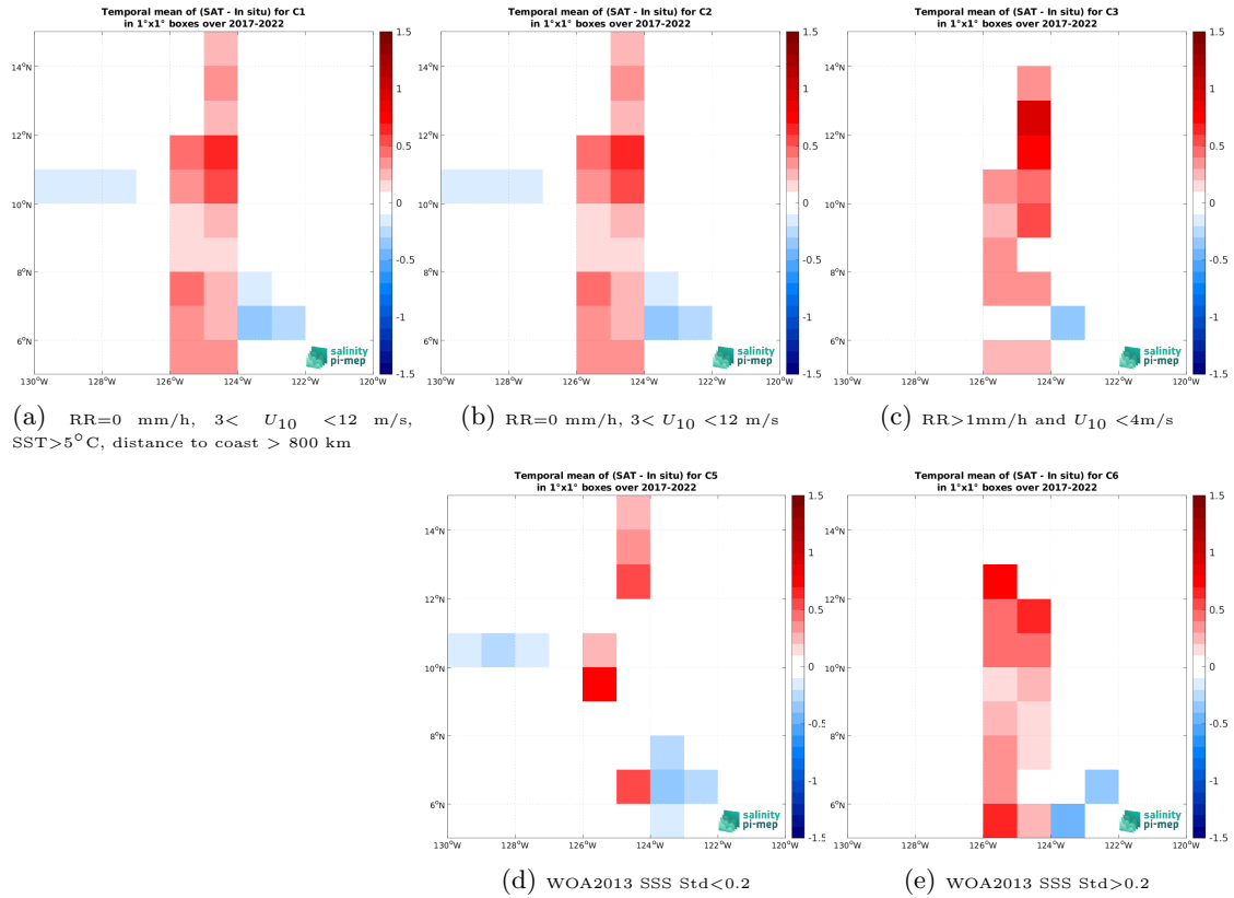
Figure 12: Temporal mean gridded over spatial boxes of size 1^\circ \times 1^\circ of \Delta SSS (SMOS SSS L3 v8 - 9 Days (CATDS-CEC-LOCEAN) - Saildrone) for 5 different subdatasets corresponding to:RR=0 mm/h, 3 < U_{10} < 12 m/s, SST >5^\circ\text{C} , distance to coast > 800 km (a), RR=0 mm/h, 3 < U_{10} < 12 m/s (b), RR >1 mm/h and U_{10} < 4 m/s (c), WOA2013 SSS Std <0.2 (d), WOA2013 SSS Std >0.2 (e).
