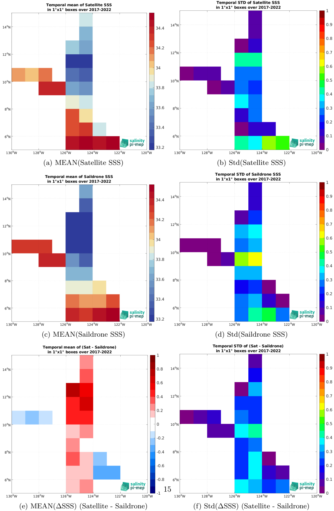
Figure 6: Temporal mean (left) and Std (right) of SSS from SMOS SSS L3 v8 - 9 Days (CATDS-CEC-LOCEAN) (top), Saildrone (middle), and of \Delta SSS (Satellite - Saildrone). Only match-up pairs are used to generate these maps.
