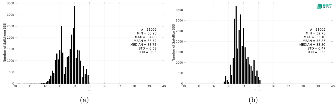
Figure 2: Histograms of SSS from Saildrone (a) and SMOS SSS L3 v8 - 9 Days (CATDS-CEC-LOCEAN) (b) considering all match-up pairs per bins of 0.1 over the SPURS 2 Pi-MEP region and for the full satellite product period.
