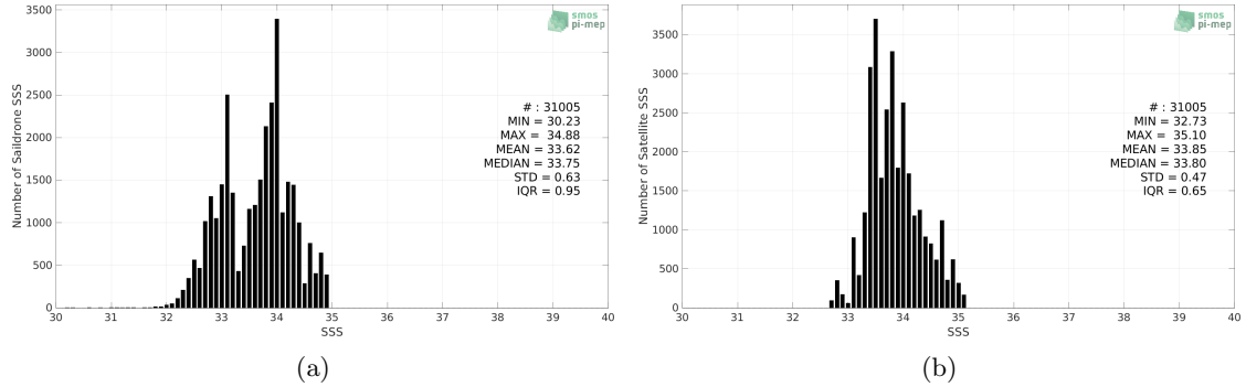
Figure 2: Histograms of SSS from Saildrone (a) and SMOS SSS L3 v8 - 9 Days (CATDS-CECOS-LOCEAN) (b) considering all match-up pairs per bins of 0.1 over the SPURS 2 Pi-MEP region and for the full satellite product period.
