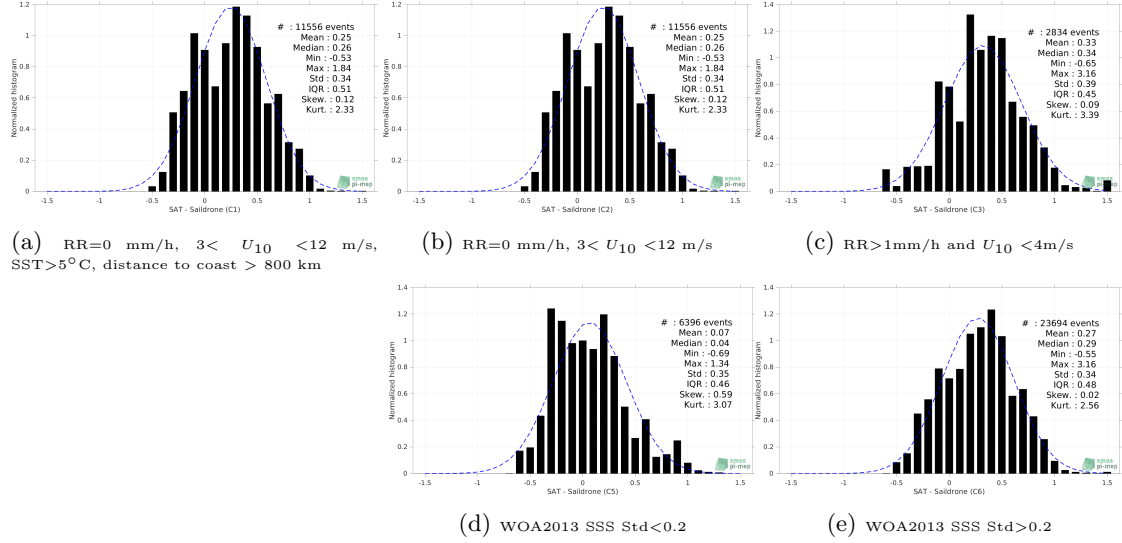
Figure 13: Normalized histogram of \Delta SSS (SMOS SSS L3 v8 - 9 Days (CATDS-CECOS-LOCEAN) - Saildrone) for 5 different subdatasets corresponding to: RR=0 mm/h, 3 < U_{10} < 12 m/s, SST>5°C, distance to coast > 800 km (a), RR=0 mm/h, 3 < U_{10} < 12 m/s (b), RR>1mm/h and U_{10} < 4 m/s (c), WOA2013 SSS Std<0.2 (d), WOA2013 SSS Std>0.2 (e).
