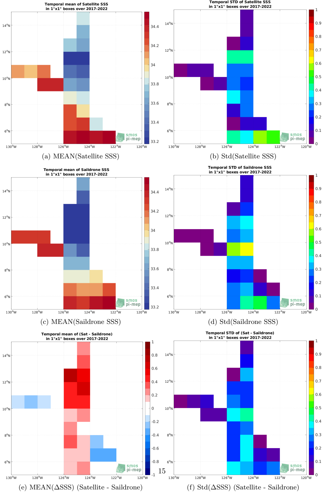
Figure 6: Temporal mean (left) and Std (right) of SSS from SMOS SSS L3 v8 - 9 Days (CATDS-CECOS-LOCEAN) (top), Saildrone (middle), and of \Delta SSS (Satellite - Saildrone). Only match-pairs are used to generate these maps.
