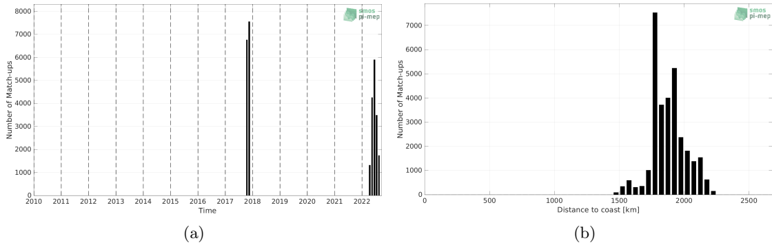
Figure 1: Number of match-ups between Saildrone and SMOS SSS L3 v8 - 9 Days (CATDS-CECOS-LOCEAN) SSS as a function of time (a) and as function of the distance to coast (b) over the SPURS 2 Pi-MEP region and for the full satellite product period.
