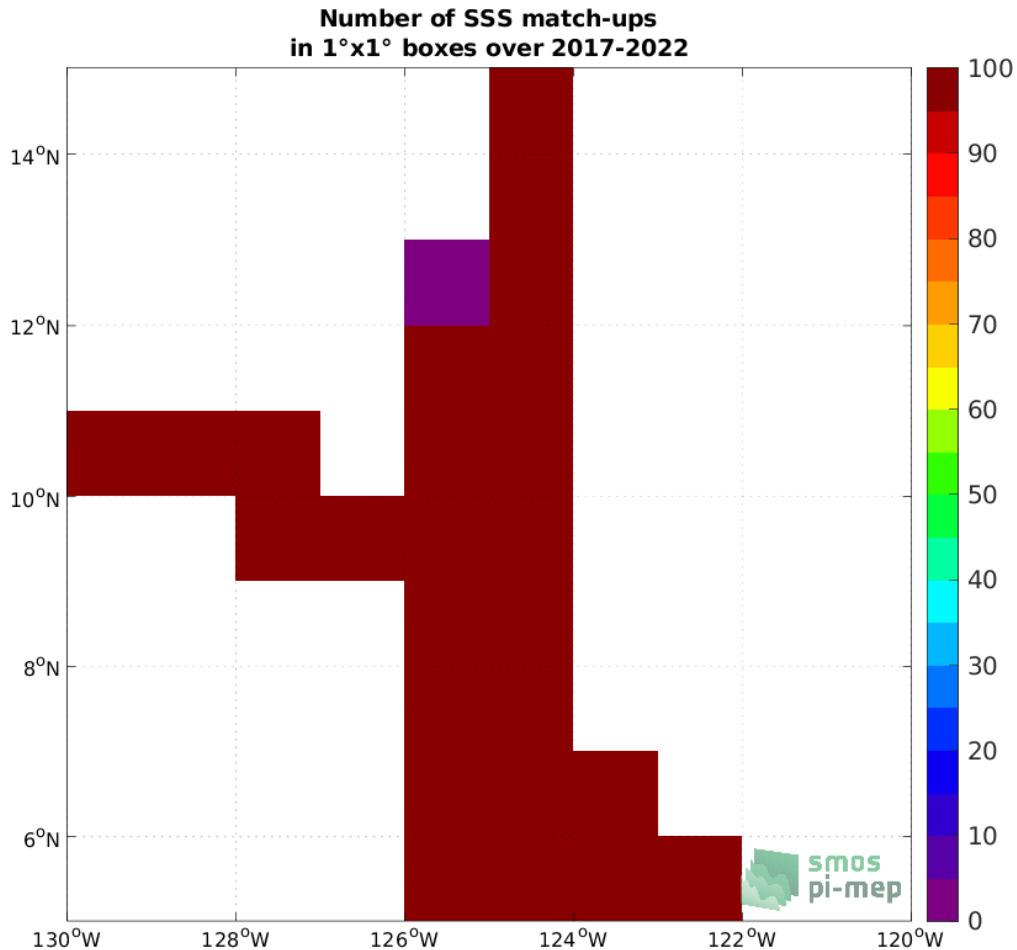
Figure 4: Number of SSS match-ups between Saildrone SSS and the SMOS SSS L3 v8 - 9 Days (CATDS-CECOS-LOCEAN) SSS product for the SPURS 2 Pi-MEP region over 1^\circ \times 1^\circ boxes and for the full satellite product period.
