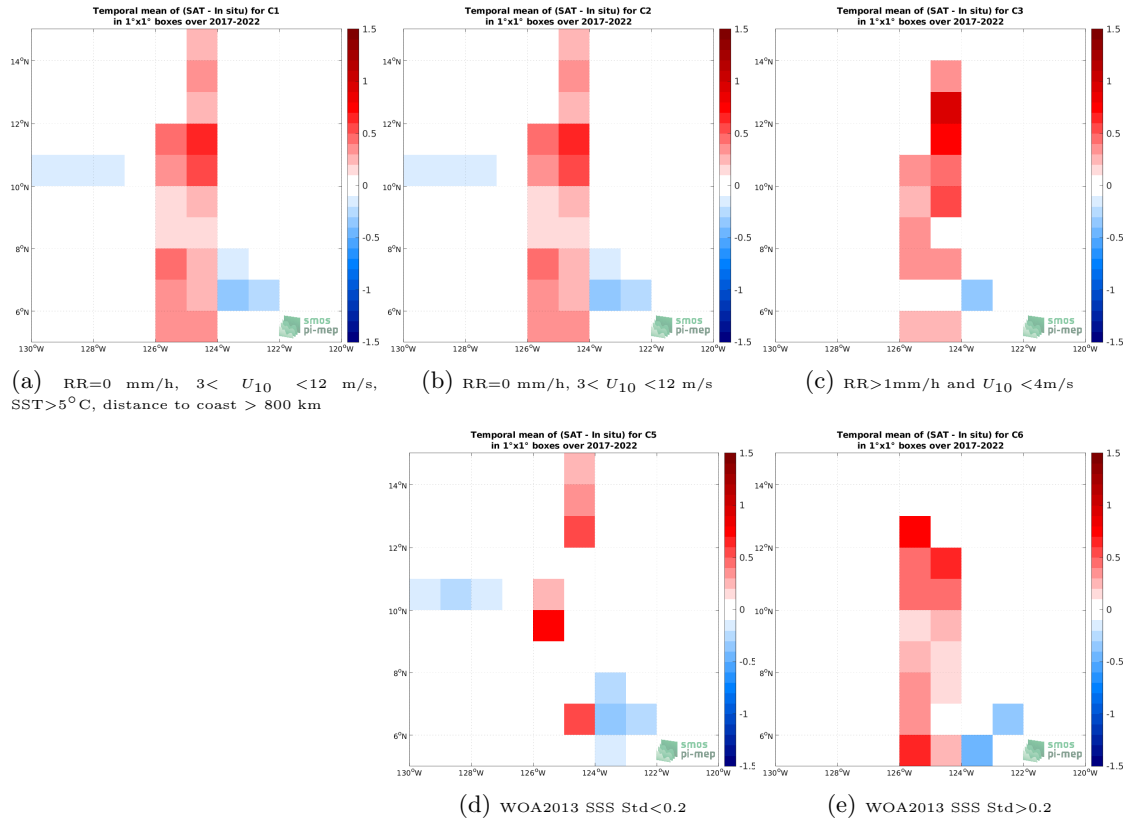
Figure 12: Temporal mean gridded over spatial boxes of size 1^\circ \times 1^\circ of \Delta SSS (SMOS SSS L3 v8 - 9 Days (CATDS-CECOS-LOCEAN) - Saildrone) for 5 different subdatasets corresponding to:RR=0 mm/h, 3 < U_{10} < 12 m/s, SST >5^\circ\text{C} , distance to coast > 800 km (a), RR=0 mm/h, 3 < U_{10} < 12 m/s (b), RR >1 mm/h and U_{10} < 4 m/s (c), WOA2013 SSS Std <0.2 (d), WOA2013 SSS Std >0.2 (e).
