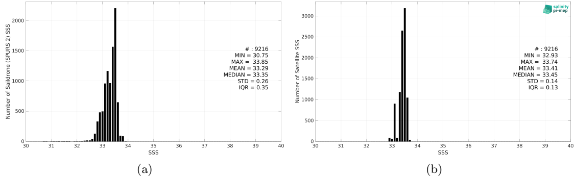
Figure 2: Histograms of SSS from Saildrone (SPURS 2) (a) and SMOS SSS L3 v8 - 9 Days (CATDS-CEC-LOCEAN) (b) considering all match-up pairs per bins of 0.1 over the SPURS 2 Pi-MEP region and for the full satellite product period.
