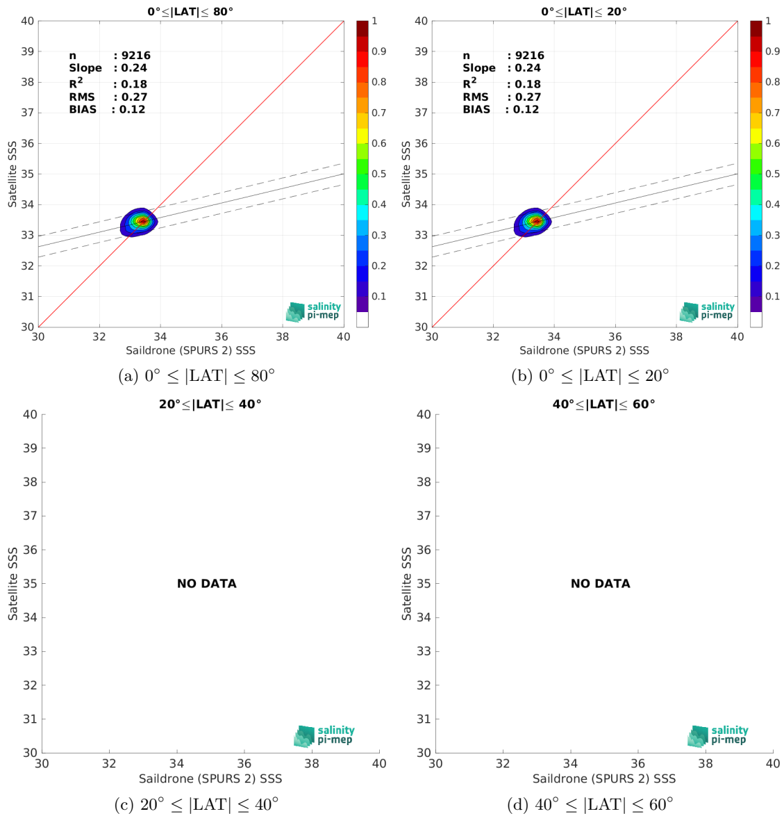
Figure 9: Contour maps of the concentration of SMOS SSS L3 v8 - 9 Days (CATDS-CEC-LOCEAN) SSS (y-axis) versus Saildrone (SPURS 2) SSS (x-axis) at match-up pairs for different latitude bands. For each plot, the red line shows x=y . The black thin and dashed lines indicate a linear fit through the data cloud and the \pm 95\% confidence levels, respectively. The number match-up pairs n , the slope and R^2 coefficient of the linear fit, the root mean square (RMS) and the mean bias between satellite and in situ data are indicated for each latitude band in each plots.
