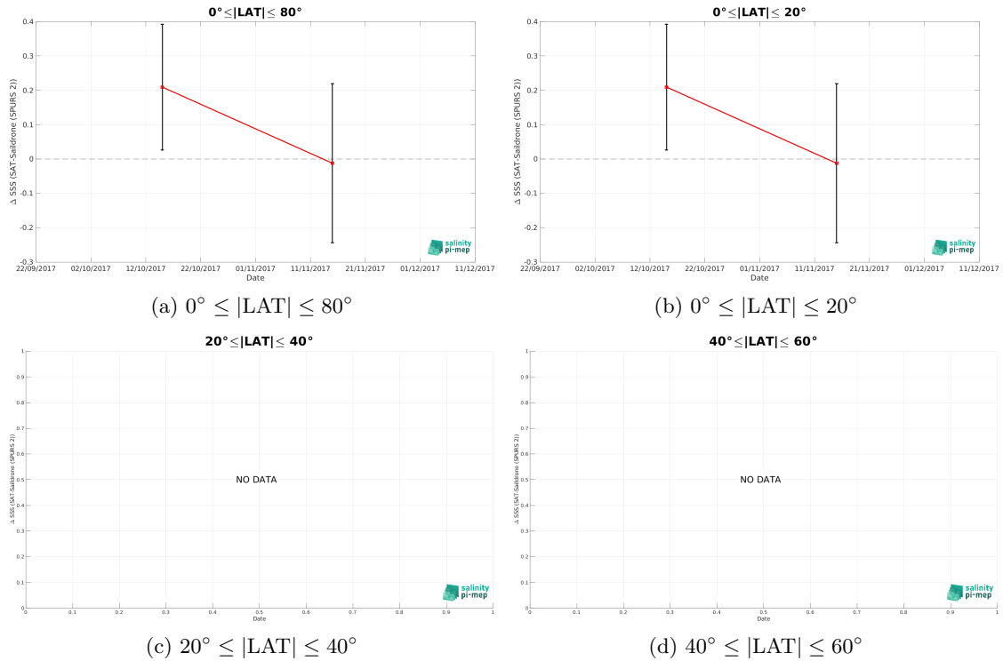
Figure 10: Monthly median (red curves) of \Delta SSS (Satellite - Sairdron (SPURS 2)) and \pm 1 Std (black vertical thick bars) as function of time for all the collected Pi-MEP match-up pairs estimated over the SPURS 2 Pi-MEP region and for the full satellite product period are shown for different latitude bands: (a) 80^{\circ}\text{S}-80^{\circ}\text{N} , (b) 20^{\circ}\text{S}-20^{\circ}\text{N} , (c) 40^{\circ}\text{S}-20^{\circ}\text{S} and 20^{\circ}\text{N}-40^{\circ}\text{N} and (d) 60^{\circ}\text{S}-40^{\circ}\text{S} and 40^{\circ}\text{N}-60^{\circ}\text{N} .
