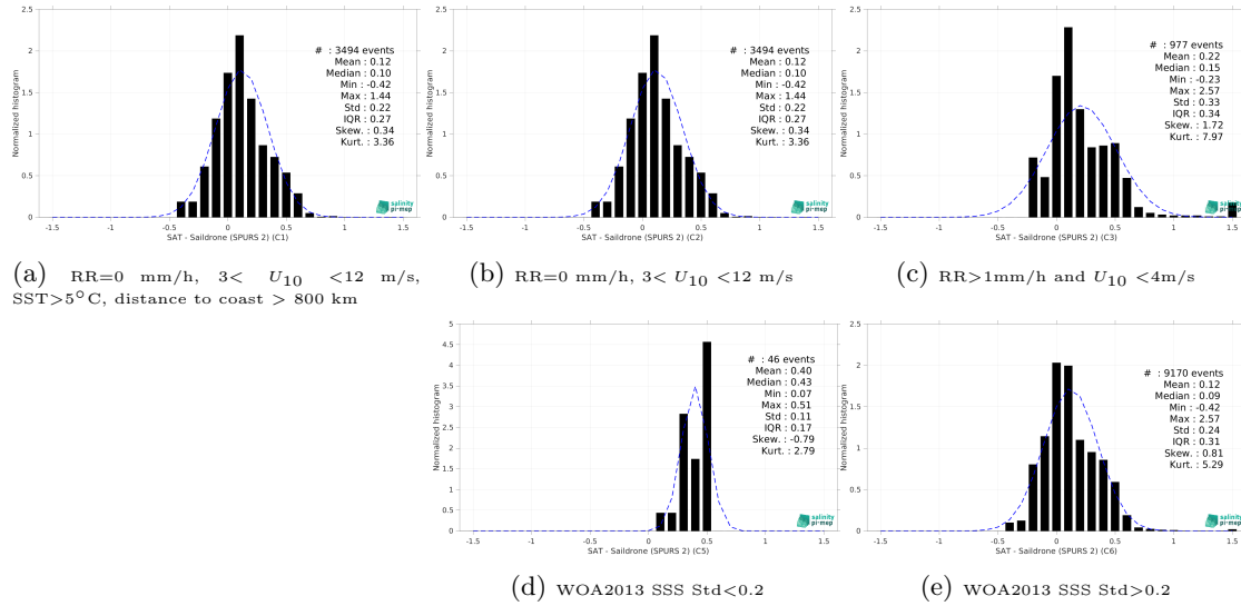
Figure 13: Normalized histogram of \Delta SSS (SMOS SSS L3 v8 - 9 Days (CATDS-CEC-LOCEAN) - Saildrone (SPURS 2)) for 5 different subdatasets corresponding to: RR=0 mm/h, 3 < U_{10} < 12 m/s, SST > 5°C, distance to coast > 800 km (a), RR=0 mm/h, 3 < U_{10} < 12 m/s (b), RR > 1mm/h and U_{10} < 4 m/s (c), WOA2013 SSS Std < 0.2 (d), WOA2013 SSS Std > 0.2 (e).
