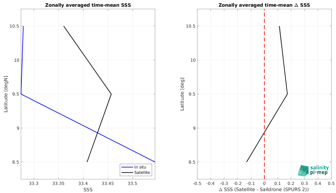
Figure 8: Left panel: Zonal mean SSS from SMOS SSS L3 v8 - 9 Days (CATDS-CEC-LOCEAN) satellite product (black) and from Sairdron (SPURS 2) (blue). Right panel: Zonal mean of \Delta SSS (Satellite - Sairdron (SPURS 2)) for all the collected Pi-MEP match-up pairs estimated over the full satellite product period.
