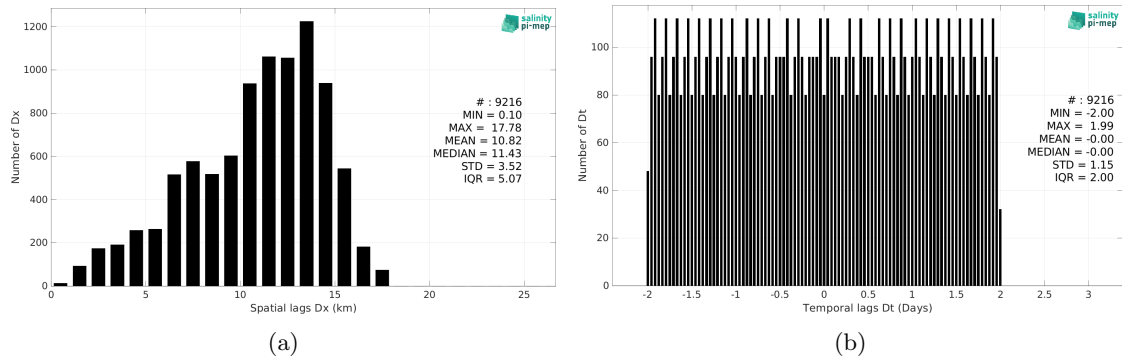
Figure 5: Histograms of the spatial (a) and temporal (b) lags between the location/time of the Saildrone (SPURS 2) measurement and the date of the corresponding SMOS SSS L3 v8 - 9 Days (CATDS-CEC-LOCEAN) SSS pixel.
