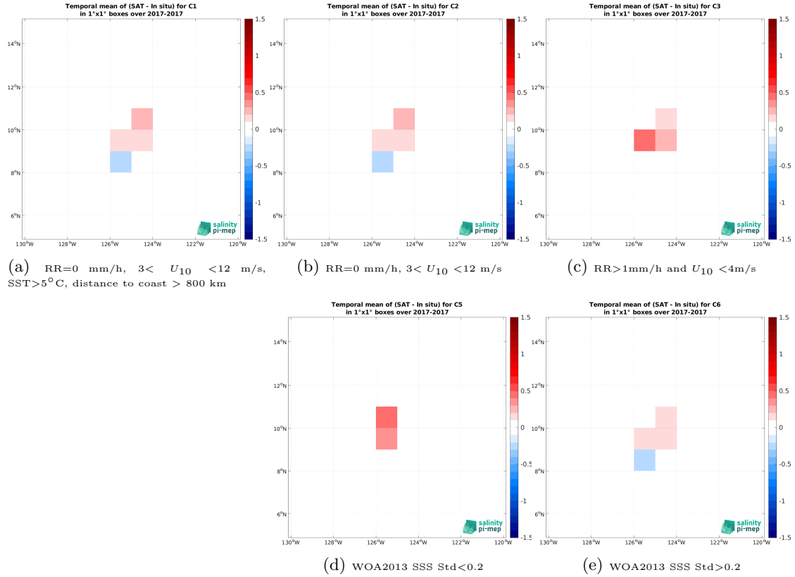
Figure 12: Temporal mean gridded over spatial boxes of size 1^{\circ}\times 1^{\circ} of \Delta\text{SSS} (SMOS SSS L3 v8 - 9 Days (CATDS-CEC-LOCEAN) - Saildrone (SPURS 2)) for 5 different subdatasets corresponding to:RR=0 mm/h, 3 < U_{10} < 12 m/s, SST >5^{\circ}\text{C} , distance to coast > 800 km (a), RR=0 mm/h, 3 < U_{10} < 12 m/s (b), RR >1 mm/h and U_{10} < 4 m/s (c), WOA2013 SSS Std <0.2 (d), WOA2013 SSS Std >0.2 (e).
