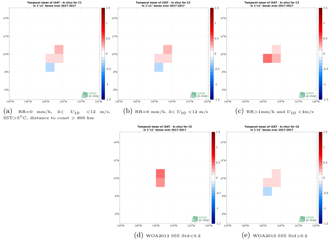
Figure 12: Temporal mean gridded over spatial boxes of size 1^{\circ}\times 1^{\circ} of \Delta\text{SSS} (SMOS SSS L3 v8 - 9 Days (CATDS-CECOS-LOCEAN) - Saildrone (SPURS 2)) for 5 different subdatasets corresponding to:RR=0 mm/h, 3 < U_{10} < 12 m/s, SST >5^{\circ}\text{C} , distance to coast > 800 km (a), RR=0 mm/h, 3 < U_{10} < 12 m/s (b), RR >1 mm/h and U_{10} < 4 m/s (c), WOA2013 SSS Std <0.2 (d), WOA2013 SSS Std >0.2 (e).
