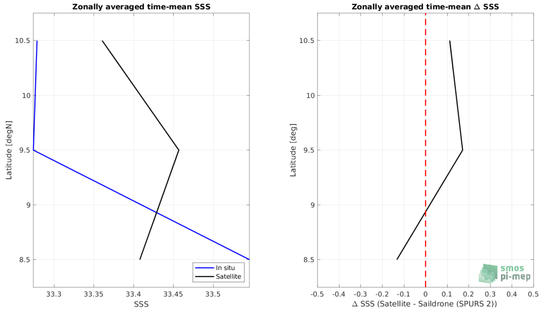
Figure 8: Left panel: Zonal mean SSS from SMOS SSS L3 v8 - 9 Days (CATDS-CECOS-LOCEAN) satellite product (black) and from Sairdrone (SPURS 2) (blue). Right panel: Zonal mean of \Delta SSS (Satellite - Sairdrone (SPURS 2)) for all the collected Pi-MEP match-up pairs estimated over the full satellite product period.
