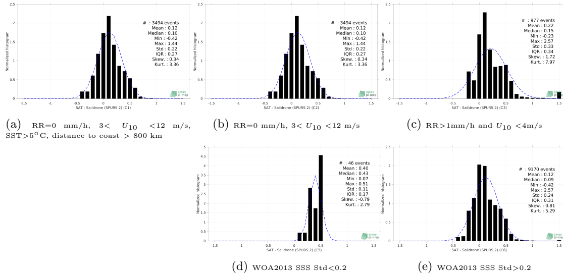
Figure 13: Normalized histogram of \Delta SSS (SMOS SSS L3 v8 - 9 Days (CATDS-CECOS-LOCEAN) - Saildrone (SPURS 2)) for 5 different subdatasets corresponding to: RR=0 mm/h, 3 < U_{10} < 12 m/s, SST>5°C, distance to coast > 800 km (a), RR=0 mm/h, 3 < U_{10} < 12 m/s (b), RR>1mm/h and U_{10} < 4 m/s (c), WOA2013 SSS Std<0.2 (d), WOA2013 SSS Std>0.2 (e).
