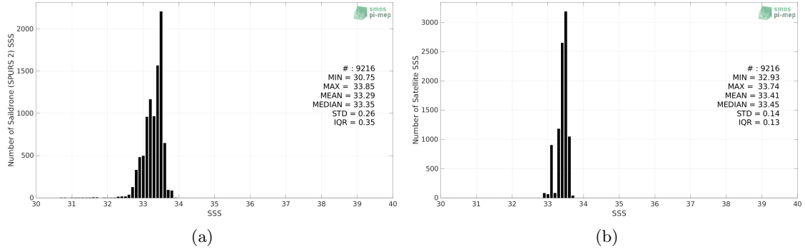
Figure 2: Histograms of SSS from Saifdrone (SPURS 2) (a) and SMOS SSS L3 v8 - 9 Days (CATDS-CECOS-LOCEAN) (b) considering all match-up pairs per bins of 0.1 over the SPURS 2 Pi-MEP region and for the full satellite product period.
