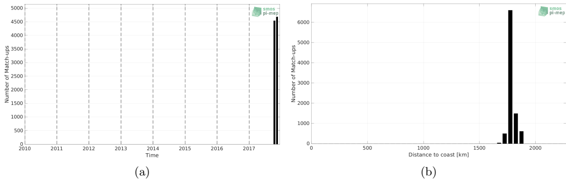
Figure 1: Number of match-ups between Saildrone (SPURS 2) and SMOS SSS L3 v8 - 9 Days (CATDS-CECOS-LOCEAN) SSS as a function of time (a) and as function of the distance to coast (b) over the SPURS 2 Pi-MEP region and for the full satellite product period.
