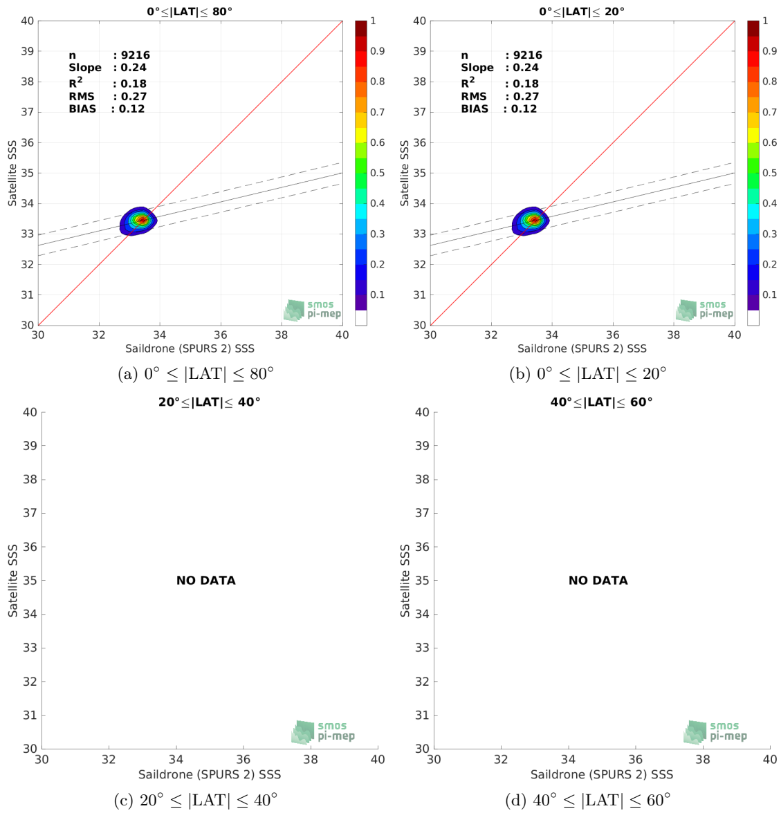
Figure 9: Contour maps of the concentration of SMOS SSS L3 v8 - 9 Days (CATDS-CECOS-LOCEAN) SSS (y-axis) versus Saildrone (SPURS 2) SSS (x-axis) at match-up pairs for different latitude bands. For each plot, the red line shows x=y . The black thin and dashed lines indicate a linear fit through the data cloud and the \pm 95\% confidence levels, respectively. The number match-up pairs n , the slope and R^2 coefficient of the linear fit, the root mean square (RMS) and the mean bias between satellite and in situ data are indicated for each latitude band in each plots.
