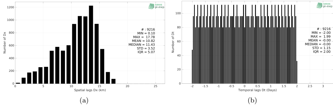
Figure 5: Histograms of the spatial (a) and temporal (b) lags between the location/time of the Saildrone (SPURS 2) measurement and the date of the corresponding SMOS SSS L3 v8 - 9 Days (CATDS-CECOS-LOCEAN) SSS pixel.
