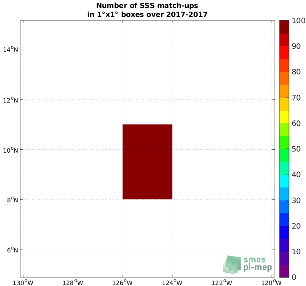
Figure 4: Number of SSS match-ups between Saildrone (SPURS 2) SSS and the SMOS SSS L3 v8 - 9 Days (CATDS-CECOS-LOCEAN) SSS product for the SPURS 2 Pi-MEP region over 1^\circ \times 1^\circ boxes and for the full satellite product period.
