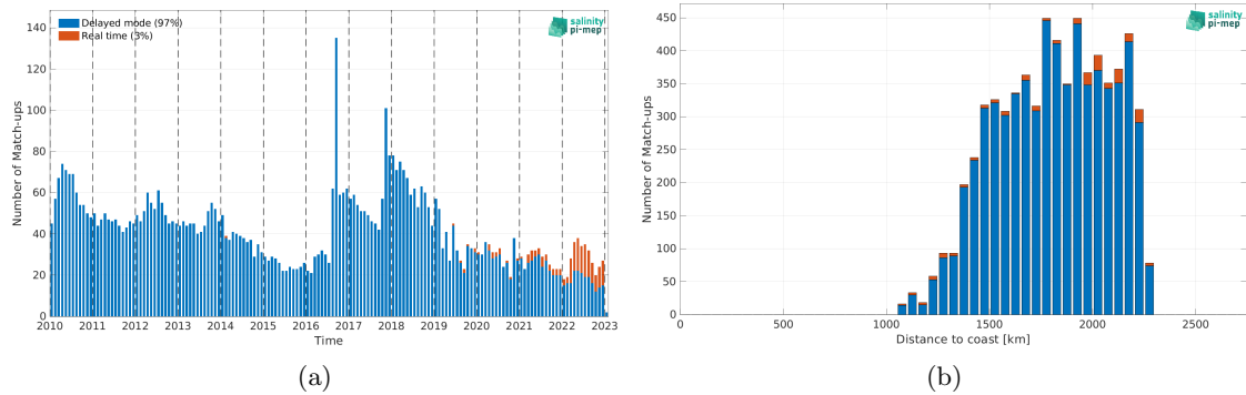
Figure 1: Number of match-ups between Argo and SMOS SSS L3 v8 - 9 Days (CATDS-CEC-LOCEAN) SSS as a function of time (a) and as function of the distance to coast (b) over the SPURS 2 Pi-MEP region and for the full satellite product period.
