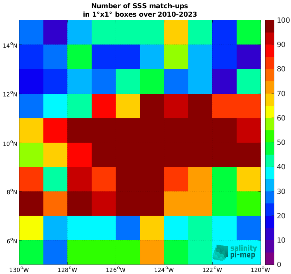
Figure 4: Number of SSS match-ups between Argo SSS and the SMOS SSS L3 v8 - 9 Days (CATDS-CEC-LOCEAN) SSS product for the SPURS 2 Pi-MEP region over 1°x1° boxes and for the full satellite product period.
