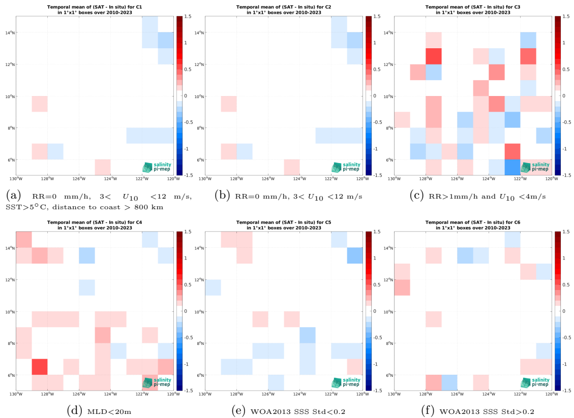
Figure 12: Temporal mean gridded over spatial boxes of size 1^\circ \times 1^\circ of \Delta SSS (SMOS SSS L3 v8 - 9 Days (CATDS-CEC-LOCEAN) - Argo) for 6 different subdatasets corresponding to:RR=0 mm/h, 3 < U_{10} < 12 m/s, SST >5^\circ C, distance to coast > 800 km (a), RR=0 mm/h, 3 < U_{10} < 12 m/s (b), RR >1 mm/h and U_{10} < 4 m/s (c),MLD <20 m (d),WOA2013 SSS Std <0.2 (e),WOA2013 SSS Std >0.2 (f).
