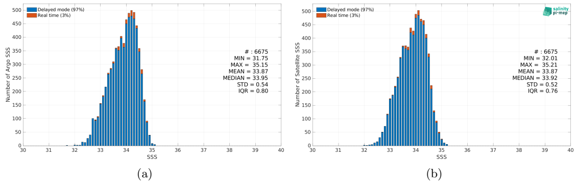
Figure 2: Histograms of SSS from Argo (a) and SMOS SSS L3 v8 - 9 Days (CATDS-CEC-LOCEAN) (b) considering all match-up pairs per bins of 0.1 over the SPURS 2 Pi-MEP region and for the full satellite product period.
