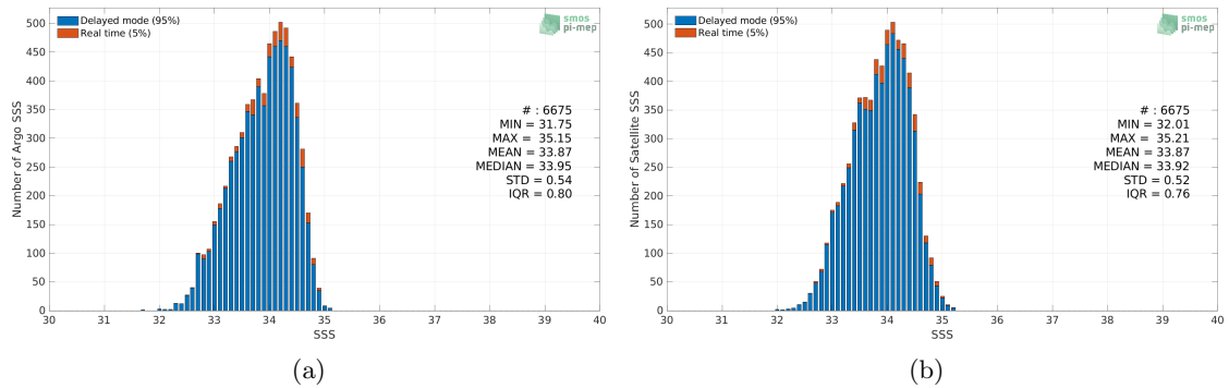
Figure 2: Histograms of SSS from Argo (a) and SMOS SSS L3 v8 - 9 Days (CATDS-CECOS-LOCEAN) (b) considering all match-up pairs per bins of 0.1 over the SPURS 2 Pi-MEP region and for the full satellite product period.
