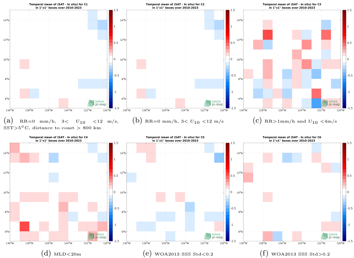
Figure 12: Temporal mean gridded over spatial boxes of size 1^\circ \times 1^\circ of \Delta SSS (SMOS SSS L3 v8 - 9 Days (CATDS-CECOS-LOCEAN) - Argo) for 6 different subdatasets corresponding to:RR=0 mm/h, 3 < U_{10} < 12 m/s, SST >5^\circ C, distance to coast > 800 km (a), RR=0 mm/h, 3 < U_{10} < 12 m/s (b), RR >1 mm/h and U_{10} < 4 m/s (c),MLD <20 m (d),WOA2013 SSS Std <0.2 (e),WOA2013 SSS Std >0.2 (f).
