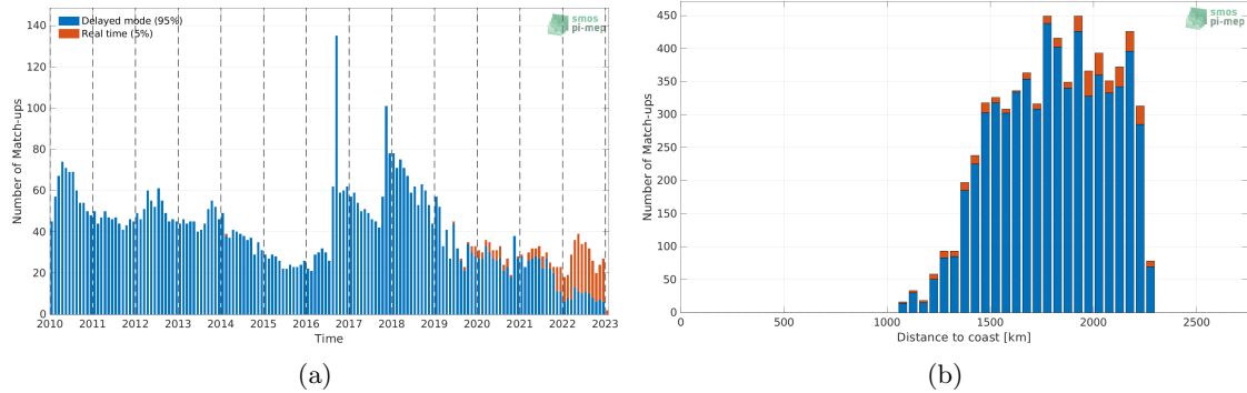
Figure 1: Number of match-ups between Argo and SMOS SSS L3 v8 - 9 Days (CATDS-CECOS-LOCEAN) SSS as a function of time (a) and as function of the distance to coast (b) over the SPURS 2 Pi-MEP region and for the full satellite product period.
