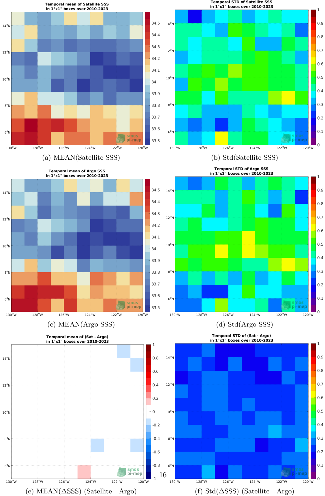
Figure 6: Temporal mean (left) and Std (right) of SSS from SMOS SSS L3 v8 - 9 Days (CATDS-CECOS-LOCEAN) (top), Argo (middle), and of \Delta SSS (Satellite - Argo). Only match-up pairs are used to generate these maps.
