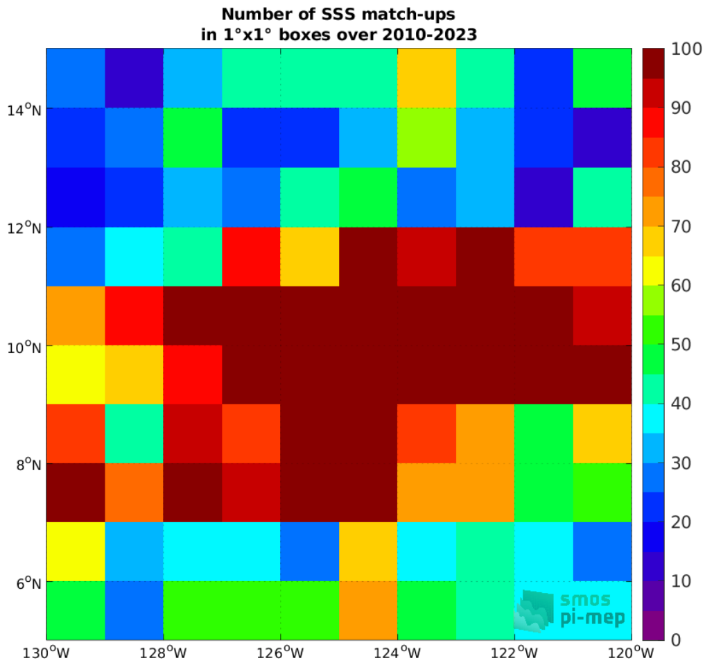
Figure 4: Number of SSS match-ups between Argo SSS and the SMOS SSS L3 v8 - 9 Days (CATDS-CECOS-LOCEAN) SSS product for the SPURS 2 Pi-MEP region over 1°x1° boxes and for the full satellite product period.
