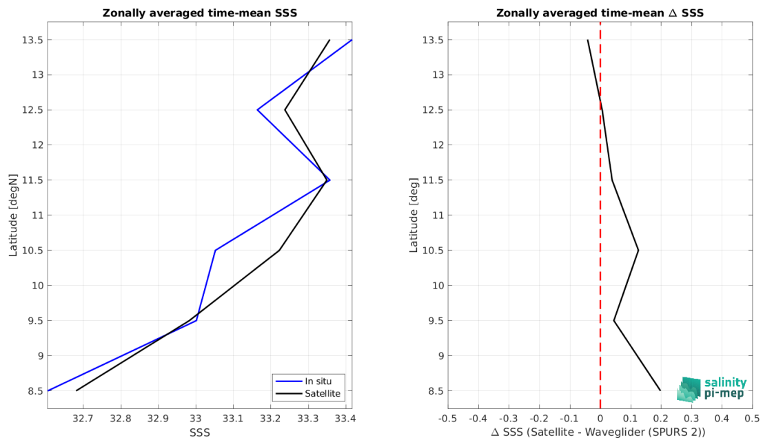
Figure 8: Left panel: Zonal mean SSS from SMOS SSS L3 v8 - 18 Days (CATDS-CEC-LOCEAN) satellite product (black) and from Waveglider (SPURS 2) (blue). Right panel: Zonal mean of \Delta SSS (Satellite - Waveglider (SPURS 2)) for all the collected Pi-MEP match-up pairs estimated over the full satellite product period.
