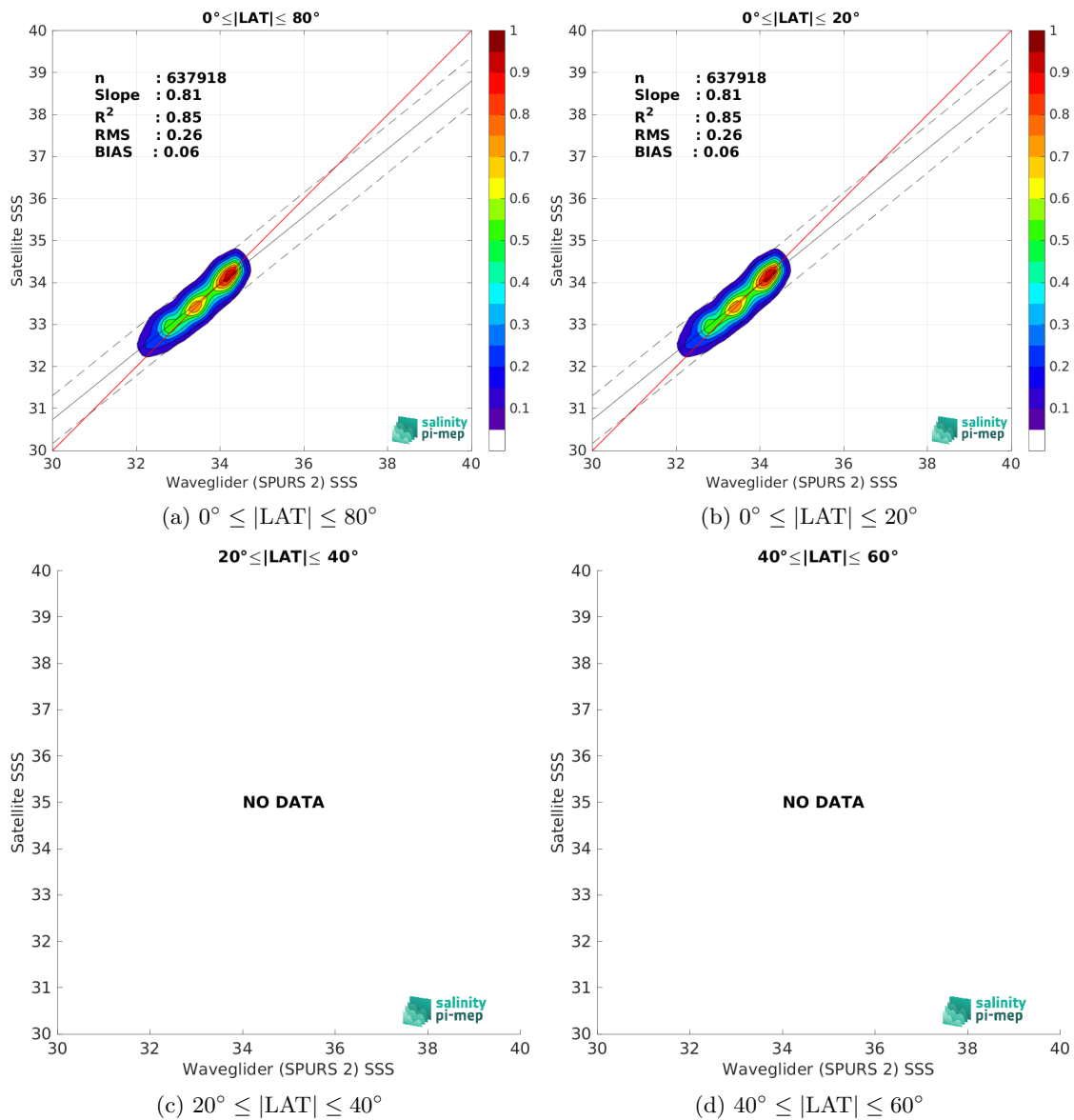
Figure 9: Contour maps of the concentration of SMOS SSS L3 v8 - 18 Days (CATDS-CEC-LOCEAN) SSS (y-axis) versus Waveglider (SPURS 2) SSS (x-axis) at match-up pairs for different latitude bands. For each plot, the red line shows x=y . The black thin and dashed lines indicate a linear fit through the data cloud and the \pm 95\% confidence levels, respectively. The number match-up pairs n , the slope and R^2 coefficient of the linear fit, the root mean square (RMS) and the mean bias between satellite and in situ data are indicated for each latitude band in each plots.
