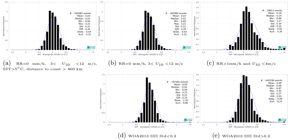
Figure 13: Normalized histogram of \Delta SSS (SMOS SSS L3 v8 - 18 Days (CATDS-CEC-LOCEAN) - Waveglider (SPURS 2)) for 5 different subdatasets corresponding to: RR=0 mm/h, 3 < U_{10} < 12 m/s, SST>5°C, distance to coast > 800 km (a), RR=0 mm/h, 3 < U_{10} < 12 m/s (b), RR>1mm/h and U_{10} < 4 m/s (c), WOA2013 SSS Std<0.2 (d), WOA2013 SSS Std>0.2 (e).
