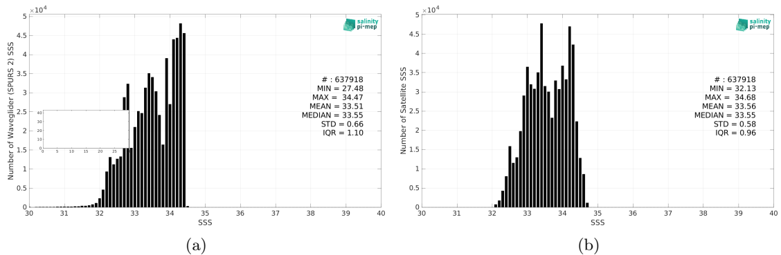
Figure 2: Histograms of SSS from Waveglider (SPURS 2) (a) and SMOS SSS L3 v8 - 18 Days (CATDS-CEC-LOCEAN) (b) considering all match-up pairs per bins of 0.1 over the SPURS 2 Pi-MEP region and for the full satellite product period.
