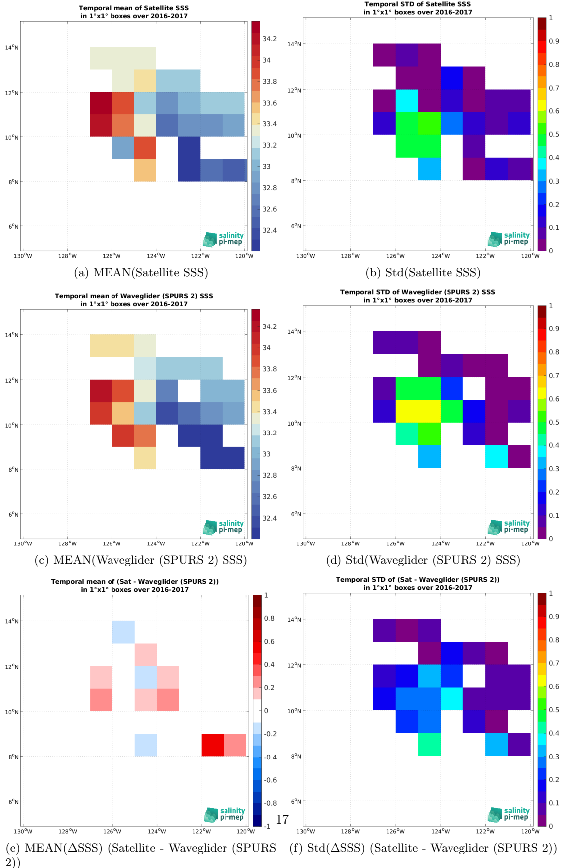
Figure 6: Temporal mean (left) and Std (right) of SSS from SMOS SSS L3 v8 - 18 Days (CATDS-CEC-LOCEAN) (top), Waveglider (SPURS 2) (middle), and of \Delta SSS (Satellite - Waveglider (SPURS 2)). Only match-up pairs are used to generate these maps.
