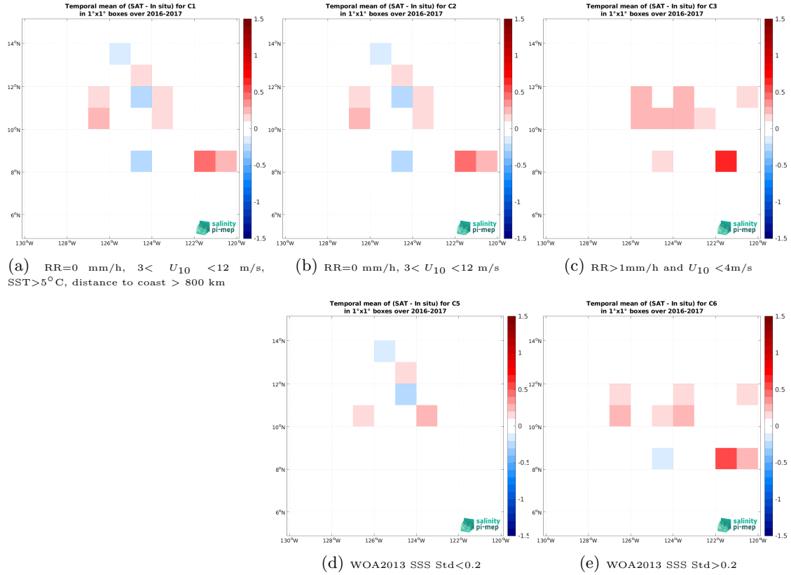
Figure 12: Temporal mean gridded over spatial boxes of size 1^{\circ}\times 1^{\circ} of \Delta\text{SSS} (SMOS SSS L3 v8 - 18 Days (CATDS-CEC-LOCEAN) - Waveglider (SPURS 2)) for 5 different subdatasets corresponding to: RR=0 mm/h, 3 < U_{10} < 12 m/s, SST > 5^{\circ}\text{C} , distance to coast > 800 km (a), RR=0 mm/h, 3 < U_{10} < 12 m/s (b), RR > 1 mm/h and U_{10} < 4 m/s (c), WOA2013 SSS Std < 0.2 (d), WOA2013 SSS Std > 0.2 (e).
