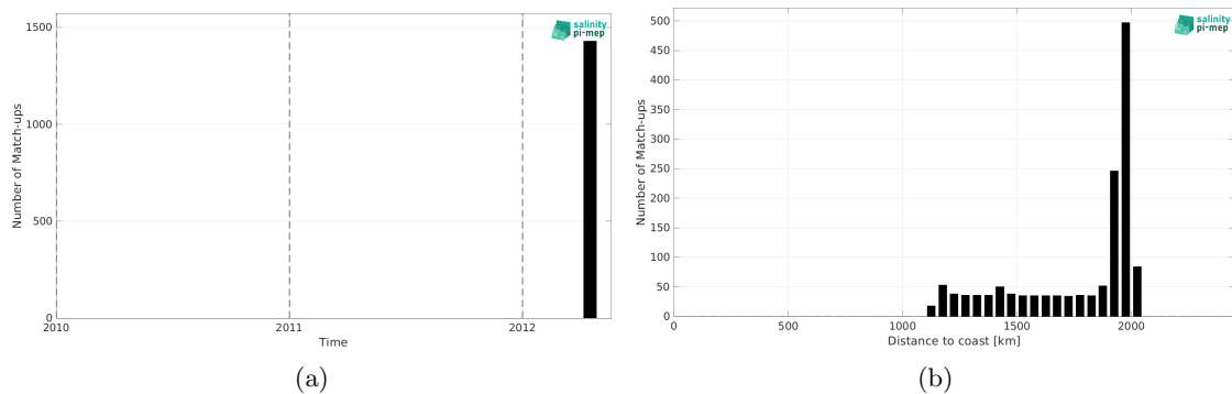
Figure 1: Number of match-ups between TSG (GOSUD-Research-vessel) and SMOS SSS L3 v8 - 18 Days (CATDS-CEC-LOCEAN) SSS as a function of time (a) and as function of the distance to coast (b) over the SPURS 2 Pi-MEP region and for the full satellite product period.
