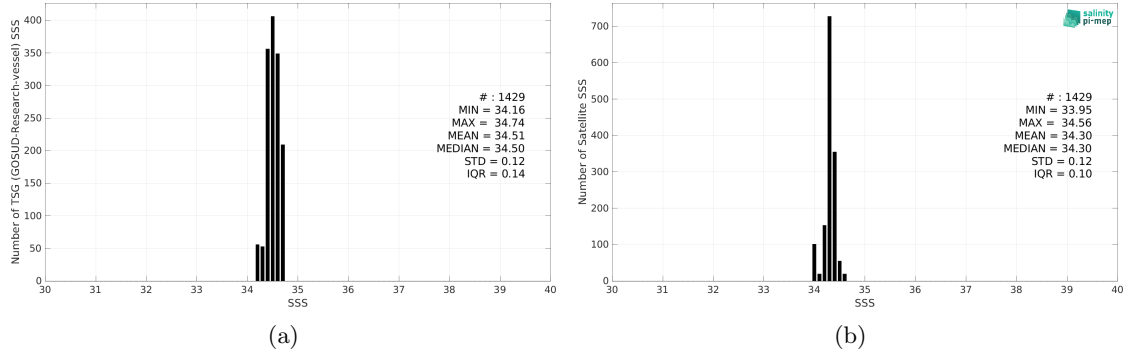
Figure 2: Histograms of SSS from TSG (GOSUD-Research-vessel) (a) and SMOS SSS L3 v8 - 18 Days (CATDS-CEC-LOCEAN) (b) considering all match-up pairs per bins of 0.1 over the SPURS 2 Pi-MEP region and for the full satellite product period.
