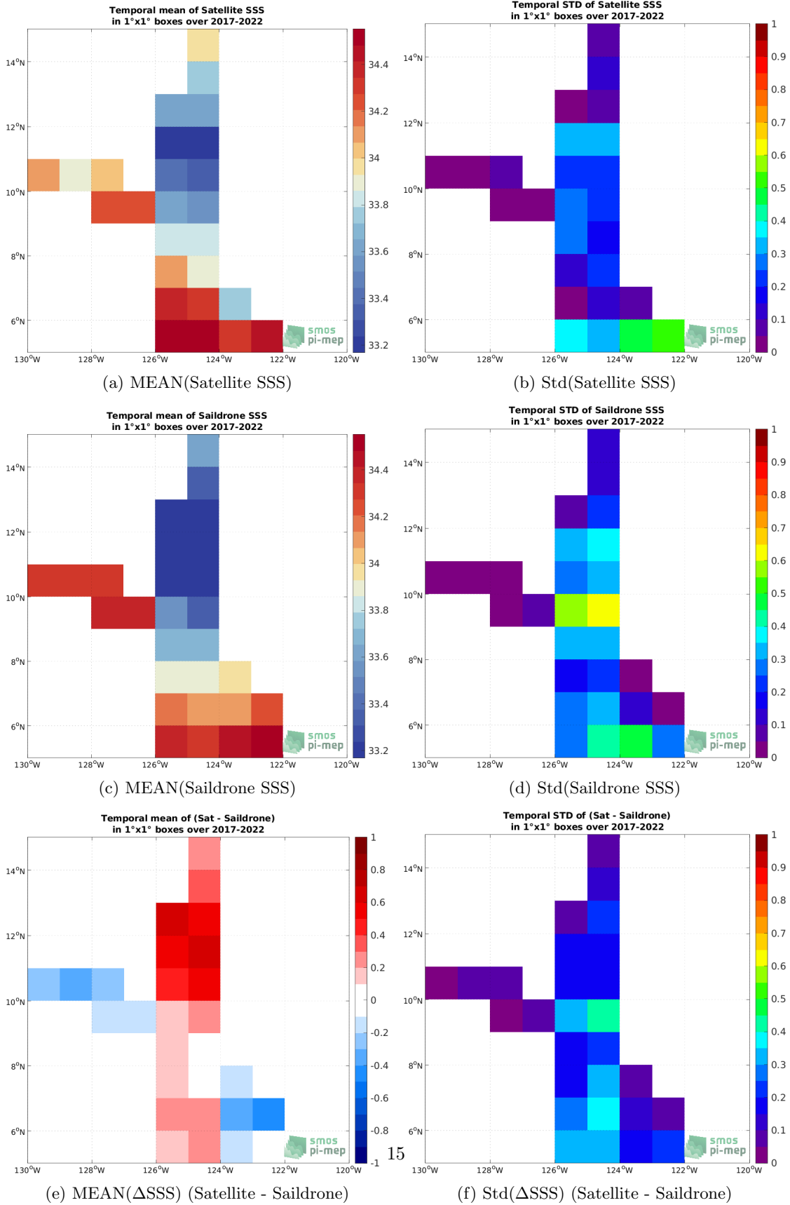
Figure 6: Temporal mean (left) and Std (right) of SSS from SMOS SSS L3 v8 - 18 Days (CATDS-CECOS-LOCEAN) (top), Saildrone (middle), and of \Delta SSS (Satellite - Saildrone). Only match-pairs are used to generate these maps.
