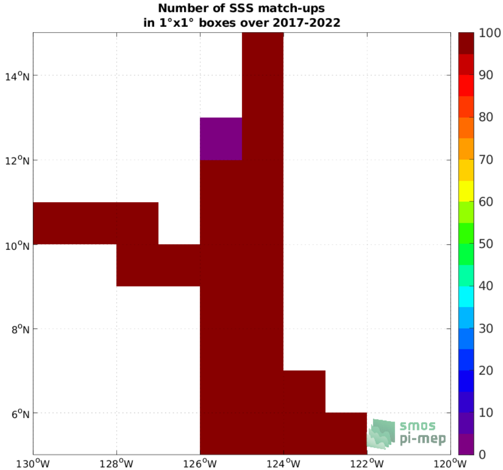
Figure 4: Number of SSS match-ups between Saildrone SSS and the SMOS SSS L3 v8 - 18 Days (CATDS-CECOS-LOCEAN) SSS product for the SPURS 2 Pi-MEP region over 1^\circ \times 1^\circ boxes and for the full satellite product period.
