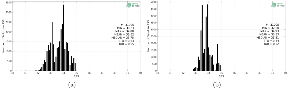
Figure 2: Histograms of SSS from Saildrone (a) and SMOS SSS L3 v8 - 18 Days (CATDS-CECOS-LOCEAN) (b) considering all match-up pairs per bins of 0.1 over the SPURS 2 Pi-MEP region and for the full satellite product period.
