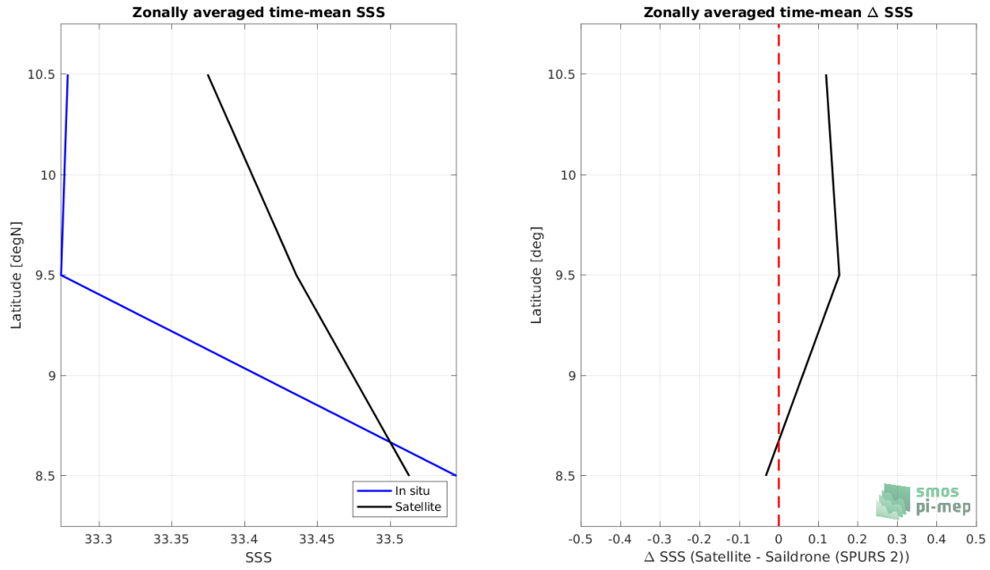
Figure 8: Left panel: Zonal mean SSS from SMOS SSS L3 v8 - 18 Days (CATDS-CECOS-LOCEAN) satellite product (black) and from Sairdrone (SPURS 2) (blue). Right panel: Zonal mean of \Delta SSS (Satellite - Sairdrone (SPURS 2)) for all the collected Pi-MEP match-up pairs estimated over the full satellite product period.
