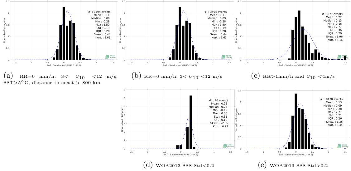
Figure 13: Normalized histogram of \Delta SSS (SMOS SSS L3 v8 - 18 Days (CATDS-CECOS-LOCEAN) - Saildrone (SPURS 2)) for 5 different subdatasets corresponding to: RR=0 mm/h, 3 < U_{10} < 12 m/s, SST>5°C, distance to coast > 800 km (a), RR=0 mm/h, 3 < U_{10} < 12 m/s (b), RR>1mm/h and U_{10} < 4 m/s (c), WOA2013 SSS Std<0.2 (d), WOA2013 SSS Std>0.2 (e).
