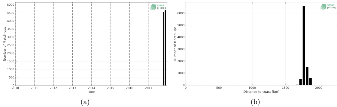
Figure 1: Number of match-ups between Saildrone (SPURS 2) and SMOS SSS L3 v8 - 18 Days (CATDS-CECOS-LOCEAN) SSS as a function of time (a) and as function of the distance to coast (b) over the SPURS 2 Pi-MEP region and for the full satellite product period.
