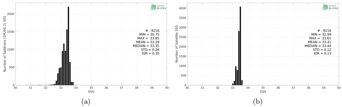
Figure 2: Histograms of SSS from Saildrone (SPURS 2) (a) and SMOS SSS L3 v8 - 18 Days (CATDS-CECOS-LOCEAN) (b) considering all match-up pairs per bins of 0.1 over the SPURS 2 Pi-MEP region and for the full satellite product period.
