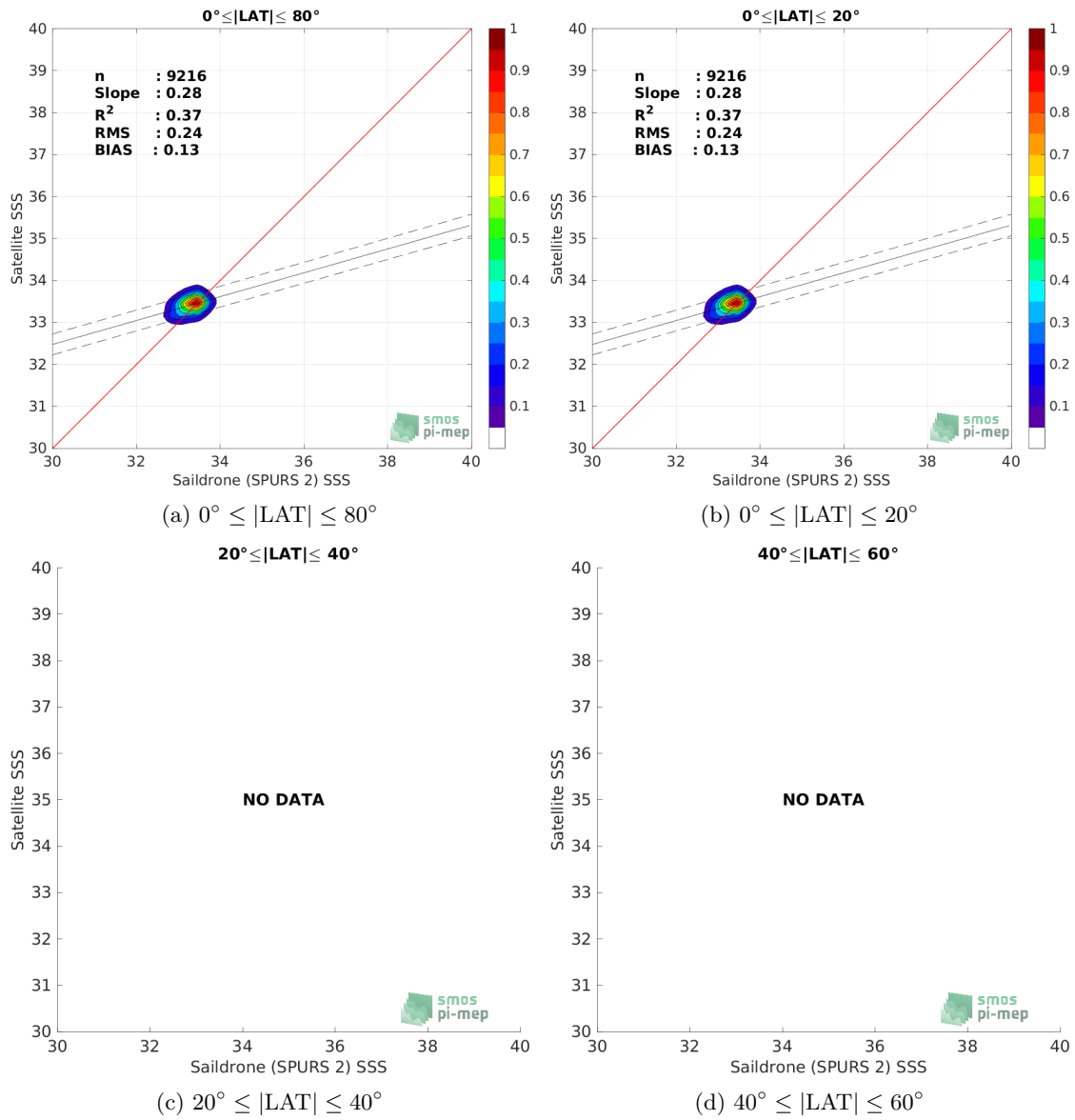
Figure 9: Contour maps of the concentration of SMOS SSS L3 v8 - 18 Days (CATDS-CECOS-LOCEAN) SSS (y-axis) versus Saildrone (SPURS 2) SSS (x-axis) at match-up pairs for different latitude bands. For each plot, the red line shows x=y . The black thin and dashed lines indicate a linear fit through the data cloud and the \pm 95\% confidence levels, respectively. The number match-up pairs n , the slope and R^2 coefficient of the linear fit, the root mean square (RMS) and the mean bias between satellite and in situ data are indicated for each latitude band in each plots.
