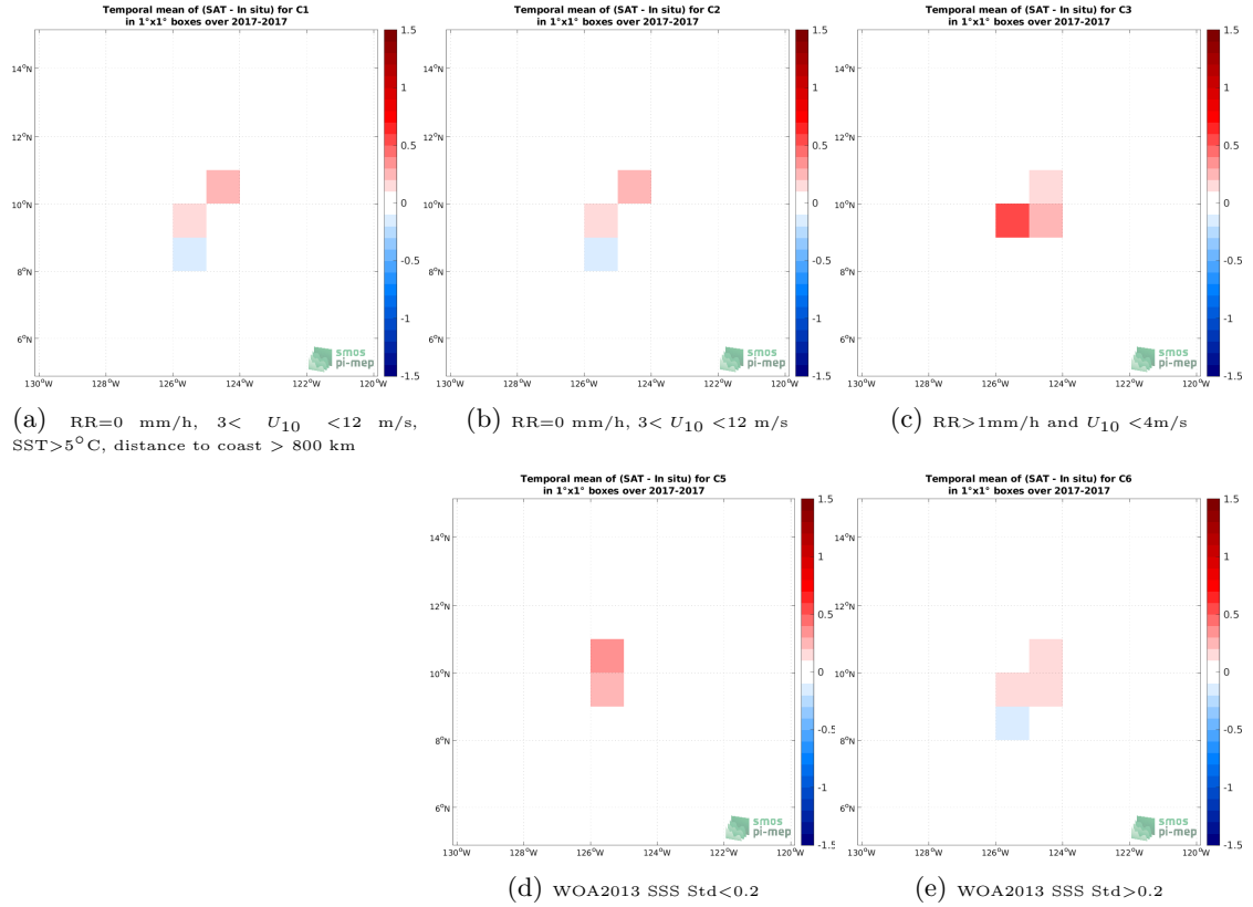
Figure 12: Temporal mean gridded over spatial boxes of size 1^{\circ}\times 1^{\circ} of \Delta\text{SSS} (SMOS SSS L3 v8 - 18 Days (CATDS-CECOS-LOCEAN) - Saildrone (SPURS 2)) for 5 different subdatasets corresponding to:RR=0 mm/h, 3 < U_{10} < 12 m/s, SST > 5^{\circ}\text{C} , distance to coast > 800 km (a), RR=0 mm/h, 3 < U_{10} < 12 m/s (b), RR > 1 mm/h and U_{10} < 4 m/s (c), WOA2013 SSS Std < 0.2 (d), WOA2013 SSS Std > 0.2 (e).
