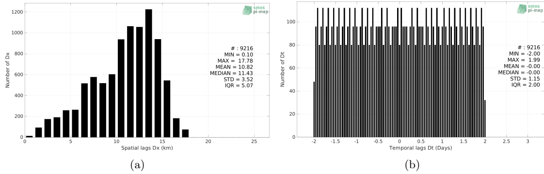
Figure 5: Histograms of the spatial (a) and temporal (b) lags between the location/time of the Saildrone (SPURS 2) measurement and the date of the corresponding SMOS SSS L3 v8 - 18 Days (CATDS-CECOS-LOCEAN) SSS pixel.
