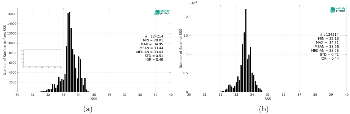
Figure 2: Histograms of SSS from Surface drifters (a) and SMOS SSS L3 v8 - 18 Days (CATDS-CEC-LOCEAN) (b) considering all match-up pairs per bins of 0.1 over the SPURS 2 Pi-MEP region and for the full satellite product period.
