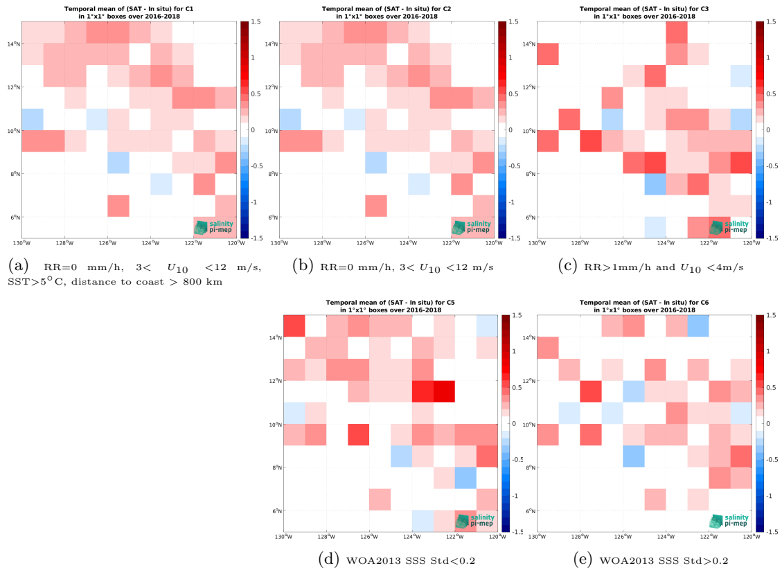
Figure 11: Temporal mean gridded over spatial boxes of size 1^\circ \times 1^\circ of \Delta SSS (SMOS SSS L3 v8 - 18 Days (CATDS-CEC-LOCEAN) - Surface drifters) for 5 different subdatasets corresponding to:RR=0 mm/h, 3 < U_{10} < 12 m/s, SST >5^\circ C, distance to coast > 800 km (a), RR=0 mm/h, 3 < U_{10} < 12 m/s (b), RR >1 mm/h and U_{10} < 4 m/s (c), WOA2013 SSS Std <0.2 (d), WOA2013 SSS Std >0.2 (e).
