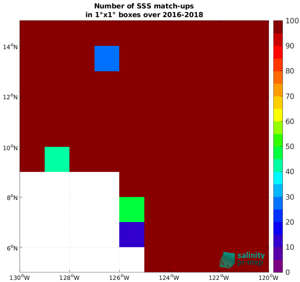
Figure 3: Number of SSS match-ups between Surface drifters SSS and the SMOS SSS L3 v8 - 18 Days (CATDS-CEC-LOCEAN) SSS product for the SPURS 2 Pi-MEP region over 1°x1° boxes and for the full satellite product period.
